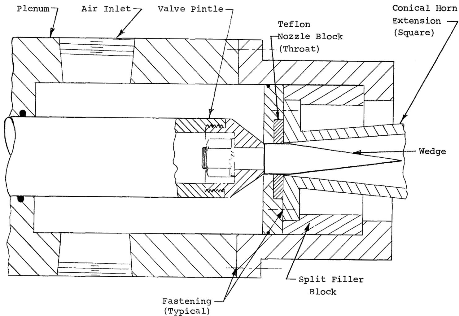
FIGURE 13 - VALVE CONFIGURATION - 10^{\circ} DOUBLE WEDGE
