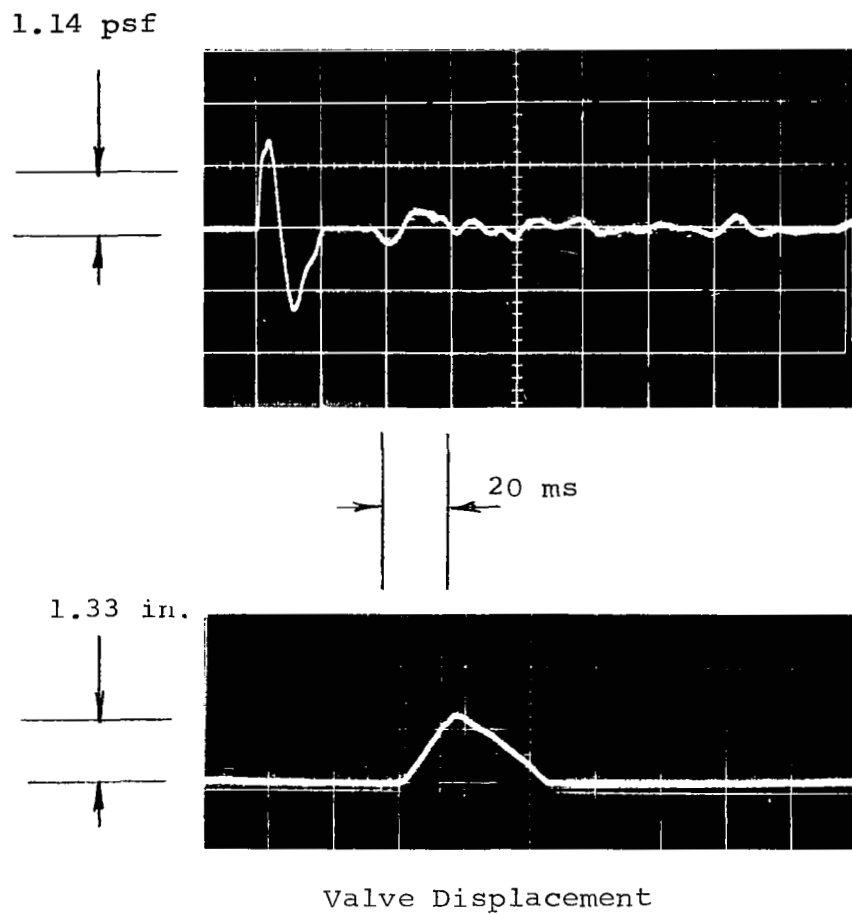
FIGURE 33 - MODERATE RISE TIME SIGNATURE RECORDED AT 84 FEET FROM THROAT. PLENUM STAGNATION PRESSURE = 50 psig. SQUARE PINTLE.
