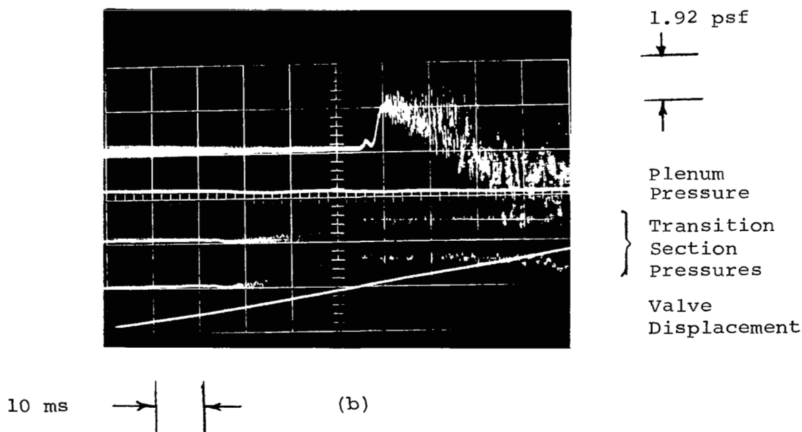
FIGURE 9 - OSCILLOSCOPE DATA DEPICTING JET NOISE SUPERIMPOSED ON SIGNATURE OBTAINED AT a) 70 AND b) 80 FEET FROM THROAT
