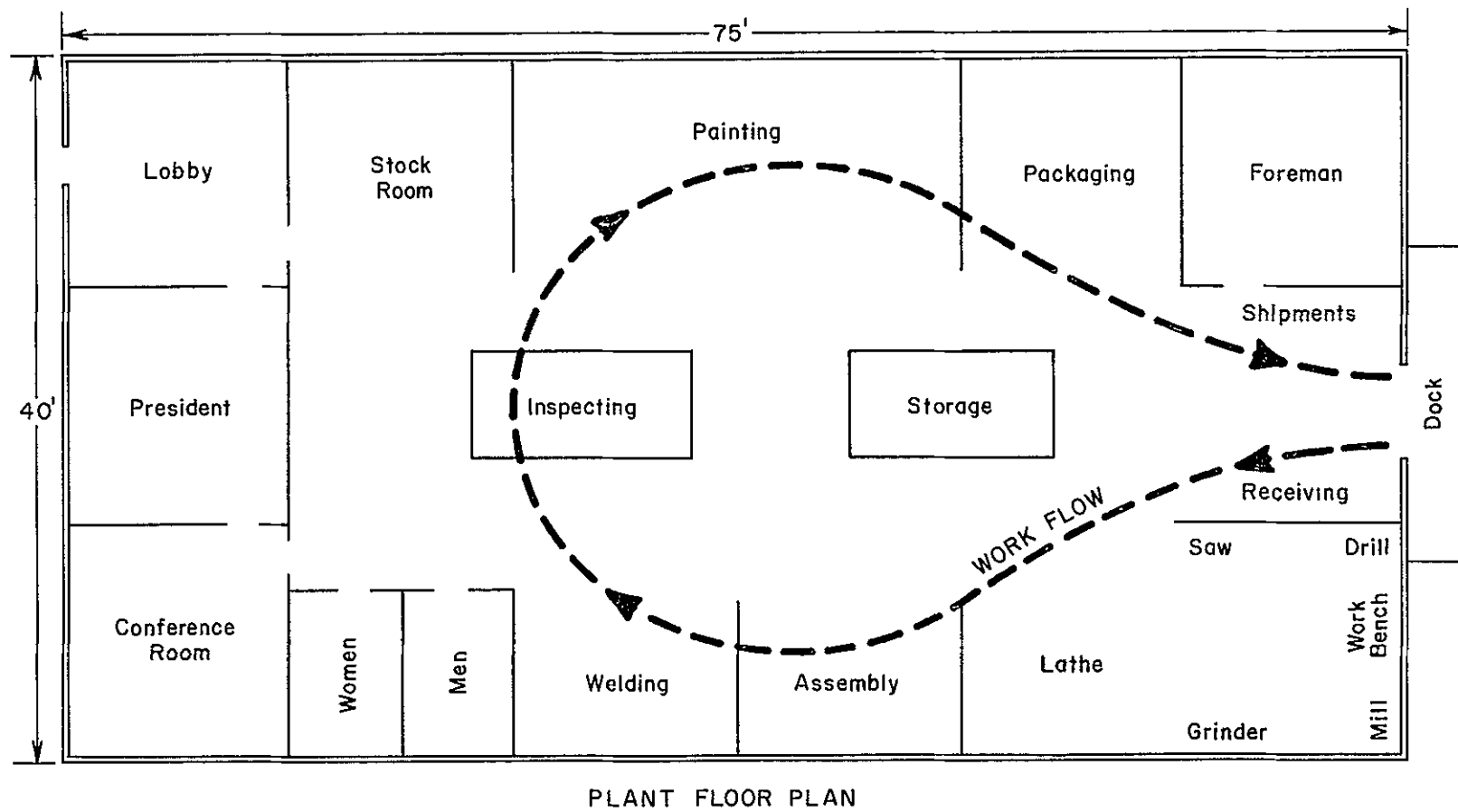
Figure 11.1 Plant Floor Plan
