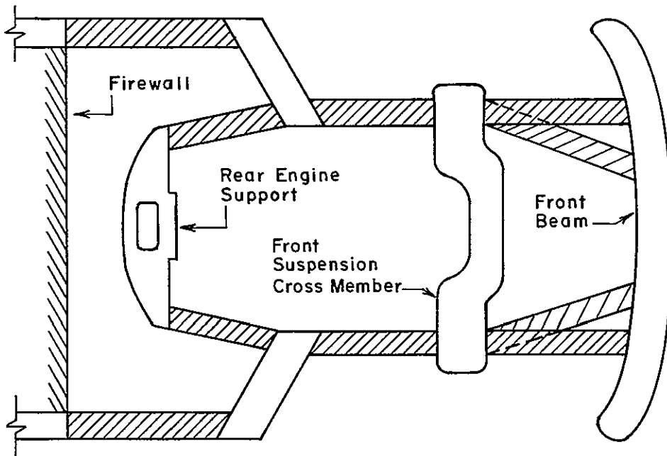
Figure 9.5.3 Energy Absorbing Frame (1)
