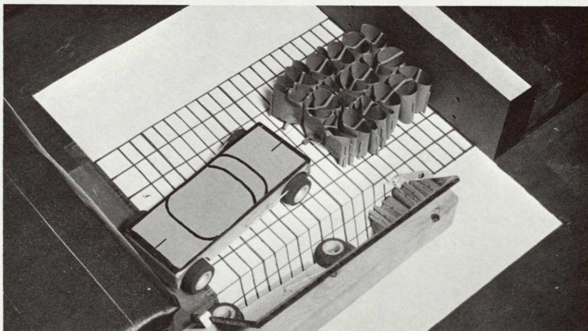
(b) Car and Barrier After Impact. (Simulated)
