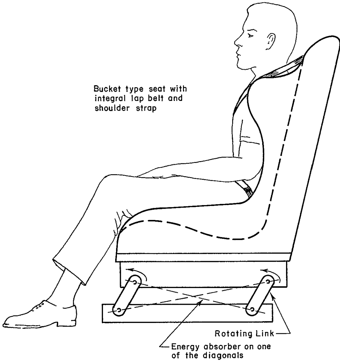
Figure 9.4.1 Sketch of Proposed Energy Absorbing Seat
