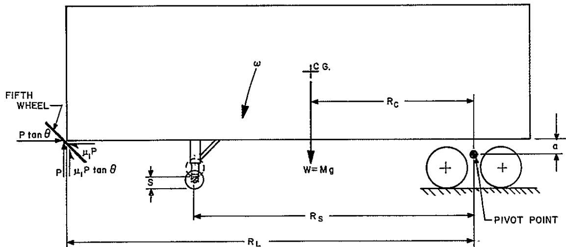
Figure 6.4 Sketch of Trailer Showing the Forces Acting at the Interface Between the Fifth Wheel and the Trailer and the Important Trailer Dimensions
