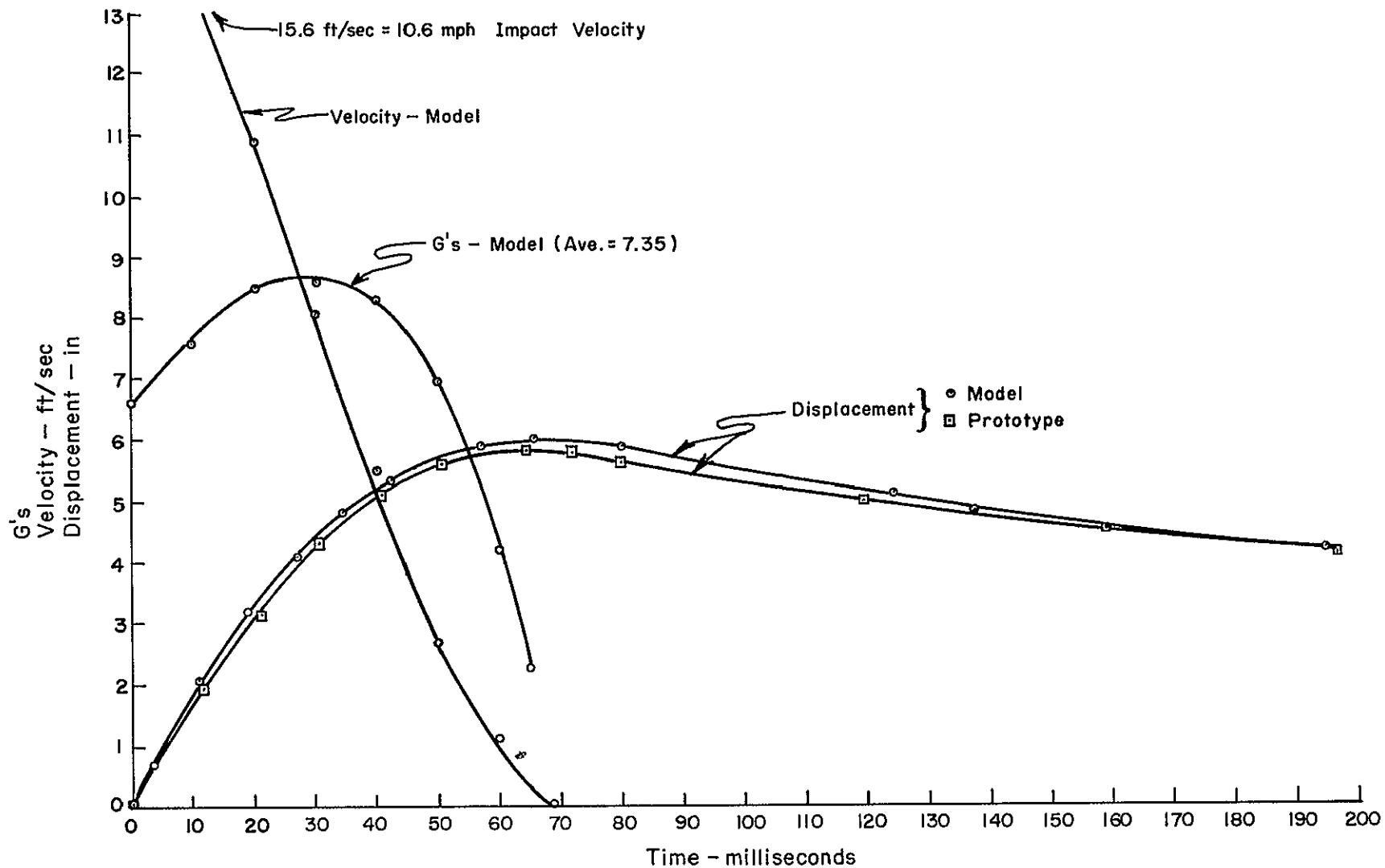
Figure 8. B. 6 Results of the Scale Model Impact Test Compared to the Results of the Actual Test (1146-5). (11) The Actual Test Data Has Been Scaled Down to the Model Dimensions of Distance and Time.
