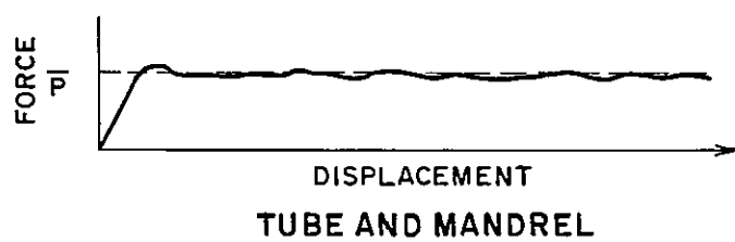
Figure 4.2 Force-Displacement Curves
