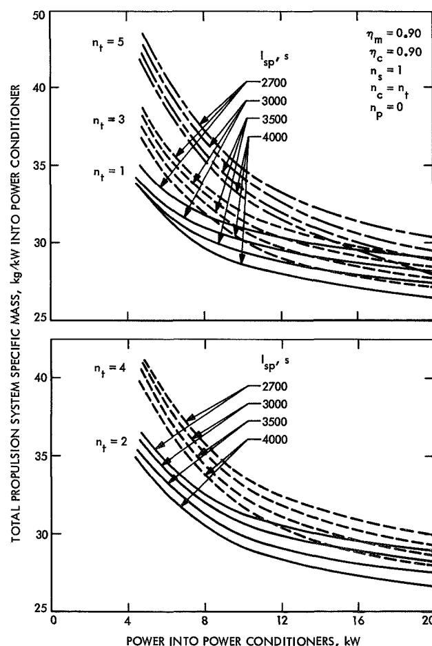
Fig. 7. Total mass of a basic thrust subsystem
