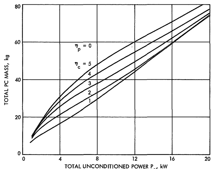
Fig. 6. Total mass of power conditioning and control elements for a multi-thruster system
