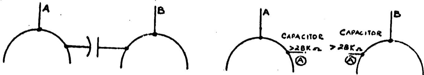
FIGURE 3-6. High Impedance Sub-Tree Partitions
