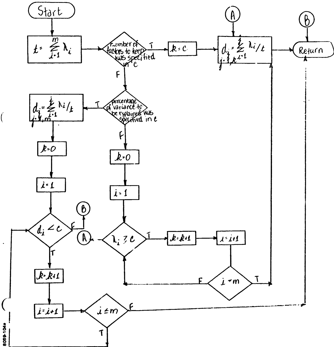
Figure 1-5 Subroutine TRACE
