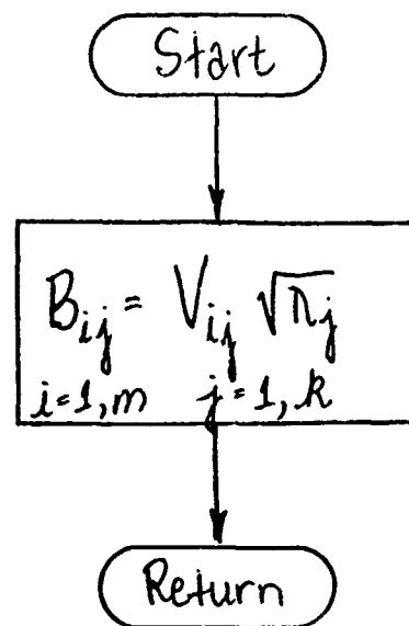
Figure 1-6 Subroutine LOAD
