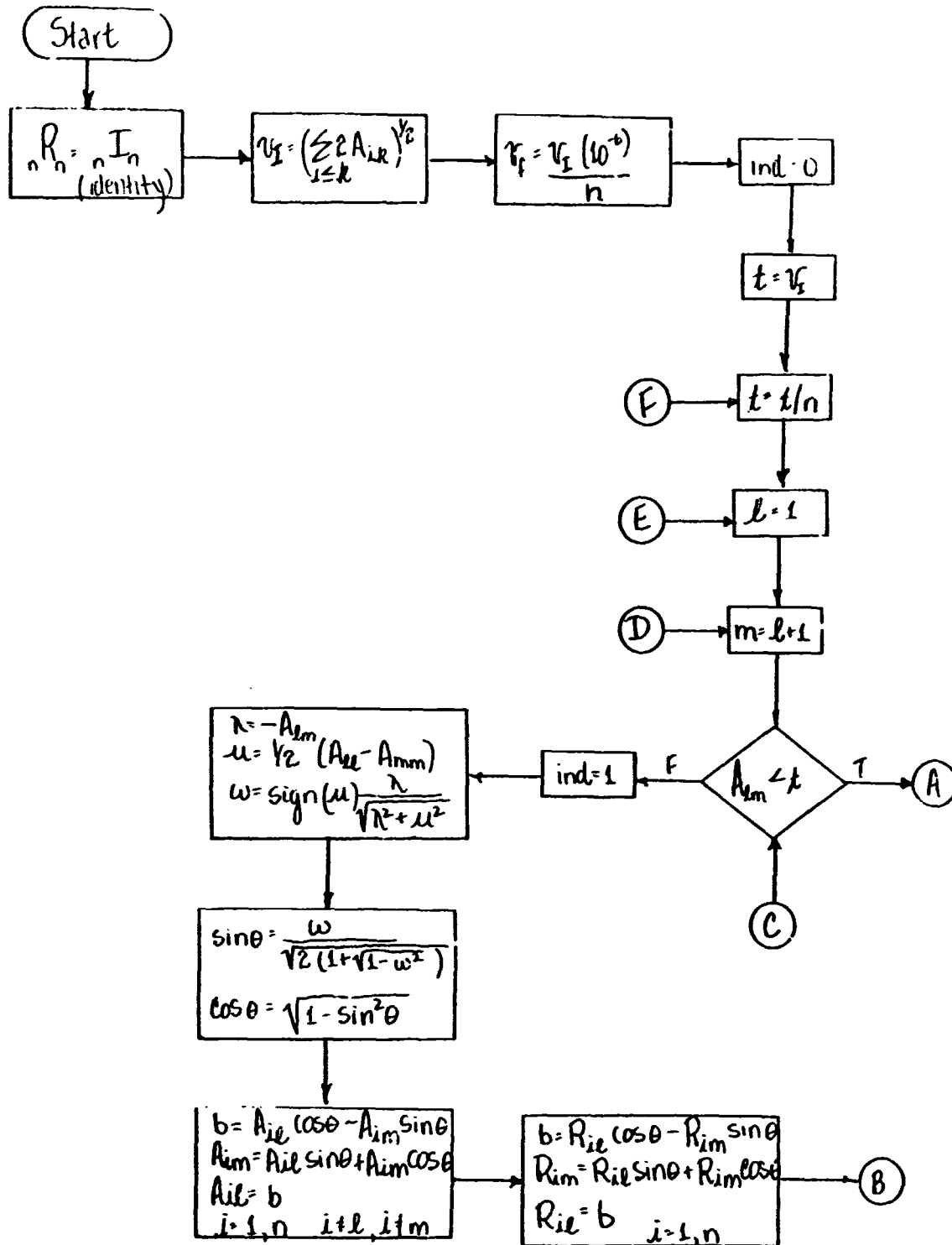
Figure 1-4 Subroutine EIGEN
