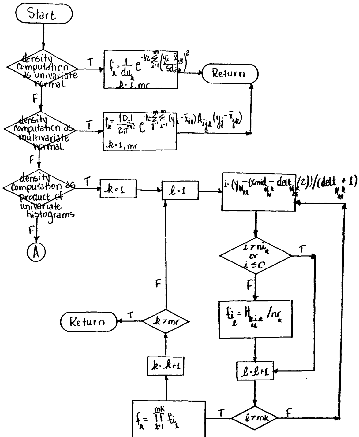
Figure 1-9 Subroutine COMPUT
