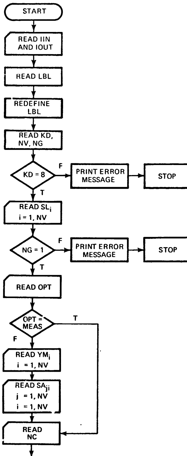
Figure 1-14 Main Program, Cluster Analysis
