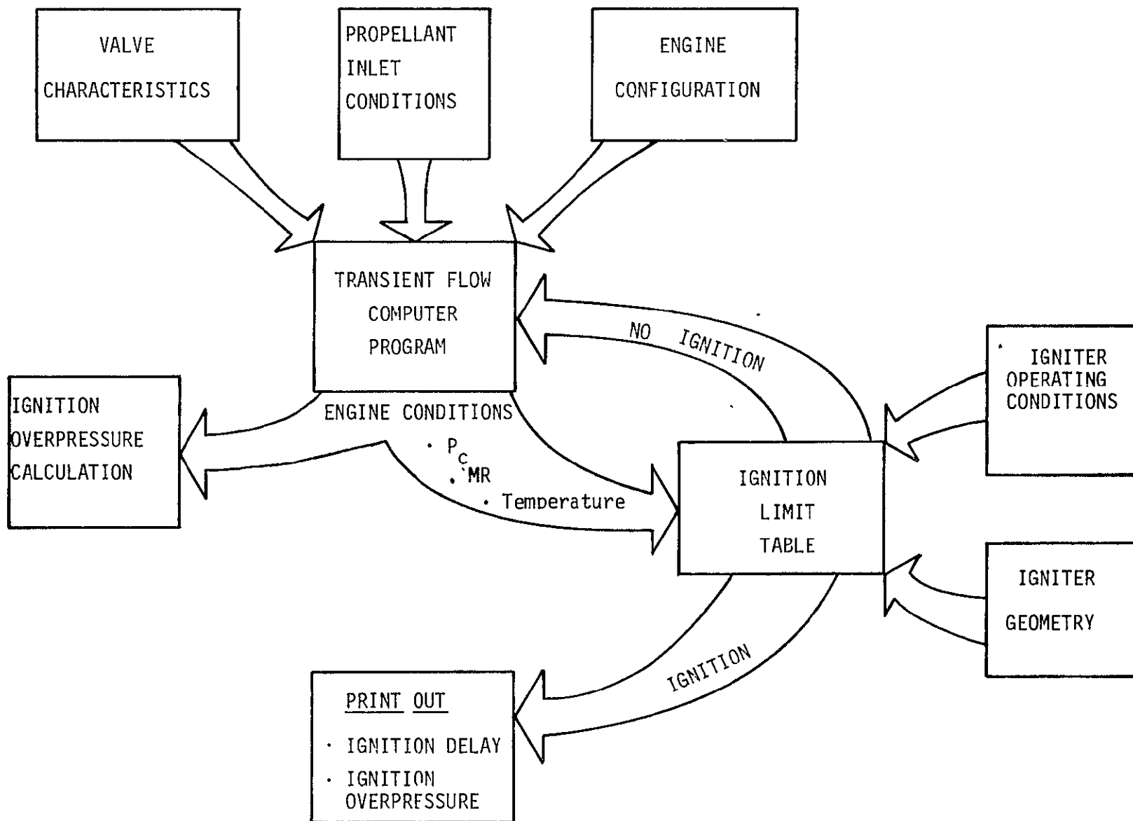
Figure 17. Engine Ignition Model - Flow Diagram
