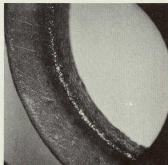
STAINLESS STEEL CATHODE POST-TEST S-2
