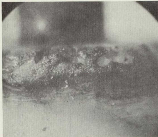
INSULATOR DETAIL - POST-TEST I-1 (15x)
