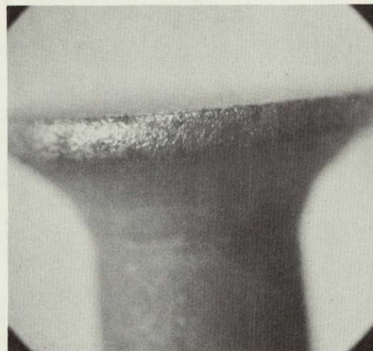
ANODE - POST-TEST I-1 (15x)
