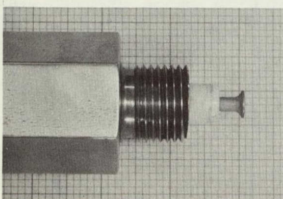
ANODE - INSULATOR ASSEMBLY PRE-TEST I-1
