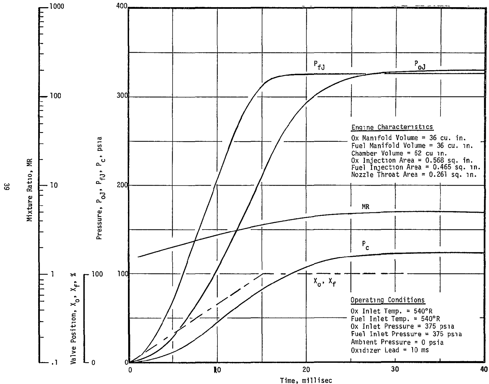
Figure 18. Calculated O_2/H_2 Engine Cold Flow Transient, Simultaneous Start
