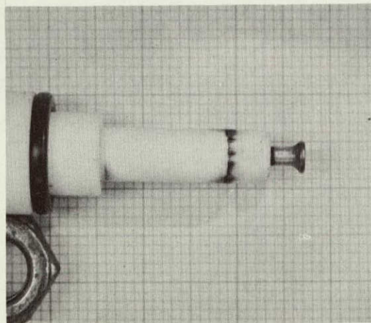
DEPOSITS ON INSULATOR POST-TEST N-1 (1.4x)
