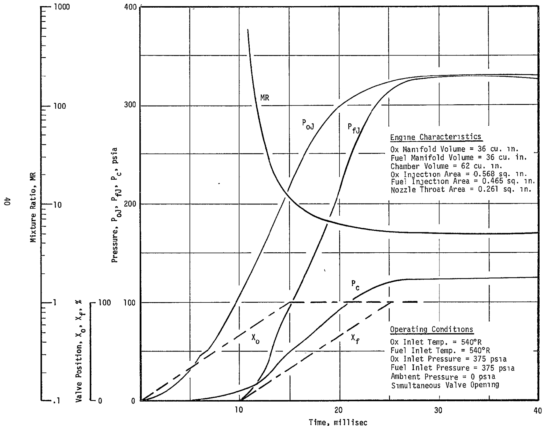
Figure 19. Calculated O_2/H_2 Engine Cold Flow Transient, Oxidizer Lead
