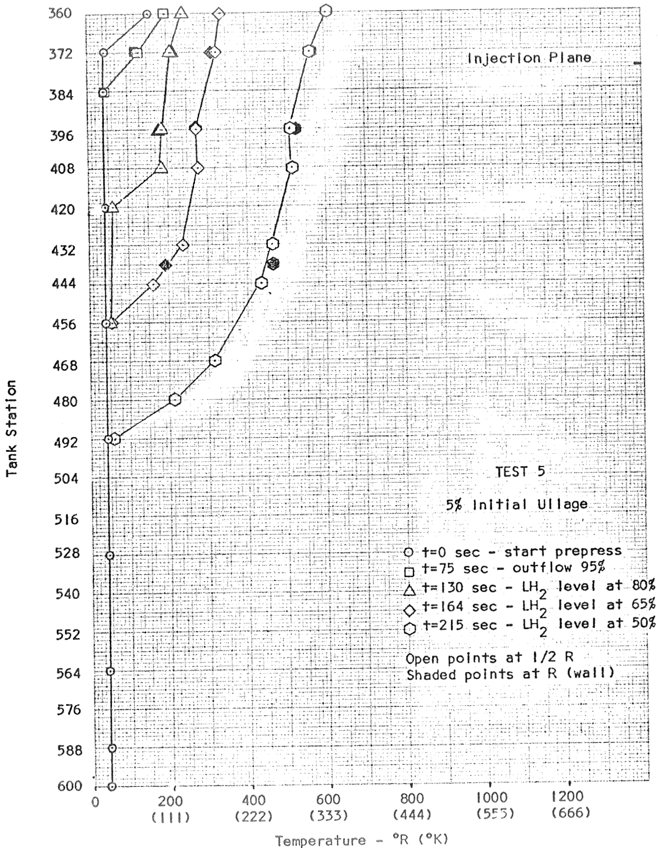
Figure 73. Axial Temperature Distribution for Test 5
