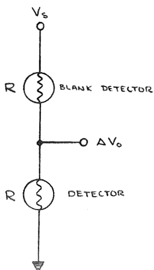
FIGURE 32 DETECTOR CONFIGURATION
