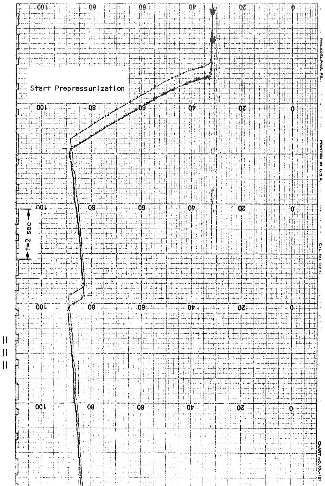
Figure 62. Control System Response - 5% Ullage - Prepressurization.
