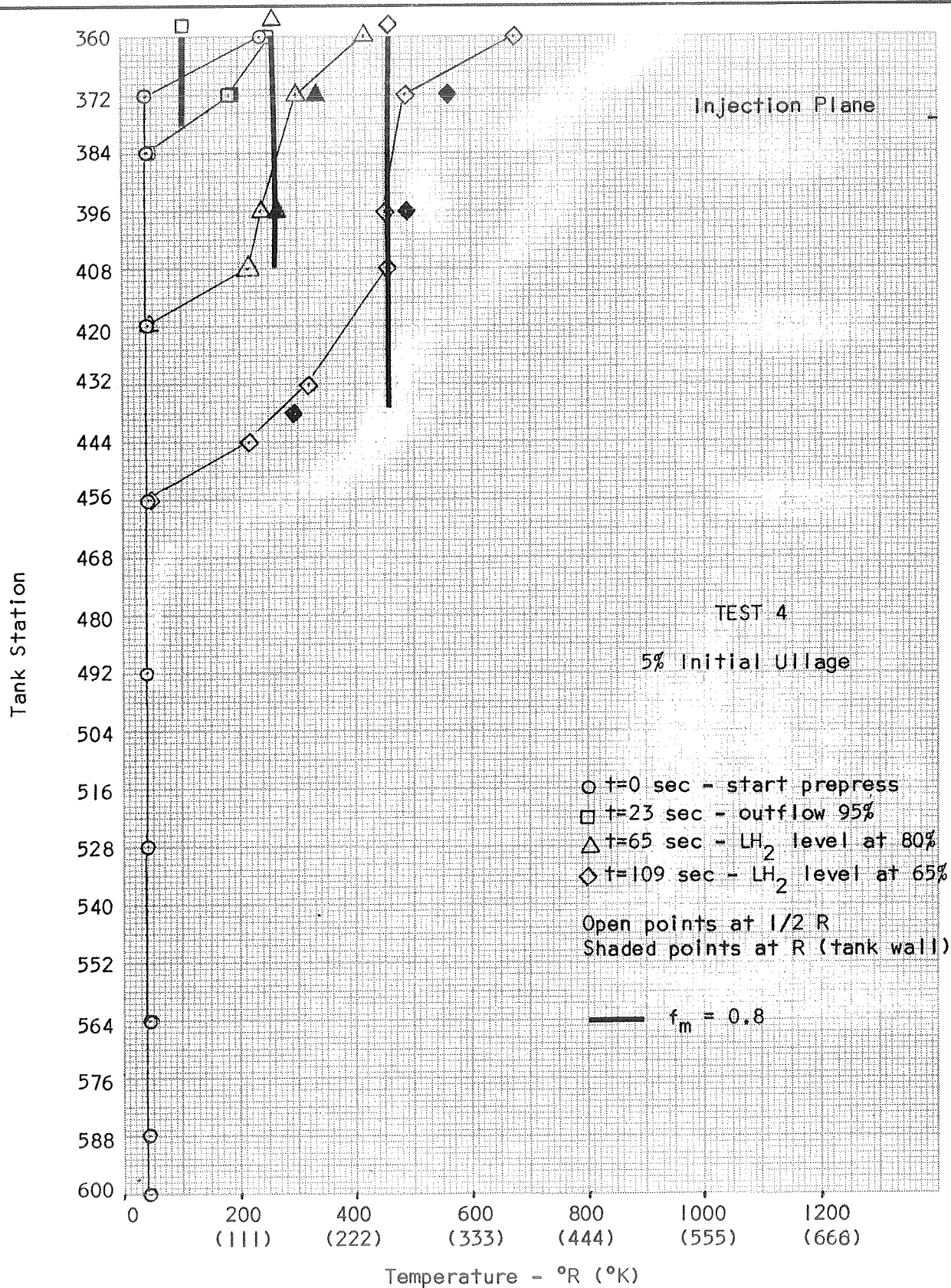
Figure 17. Temperature Correlation for Test 4
