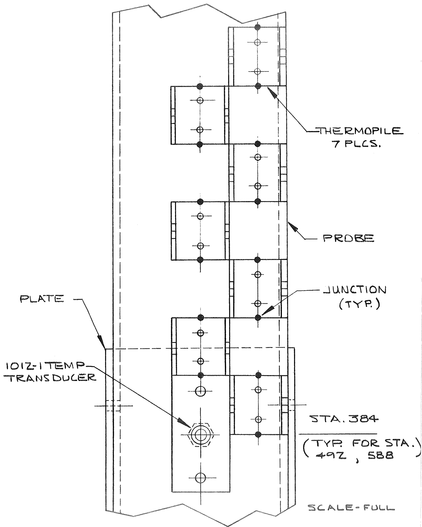
Figure 57. Thermopile Assembly
