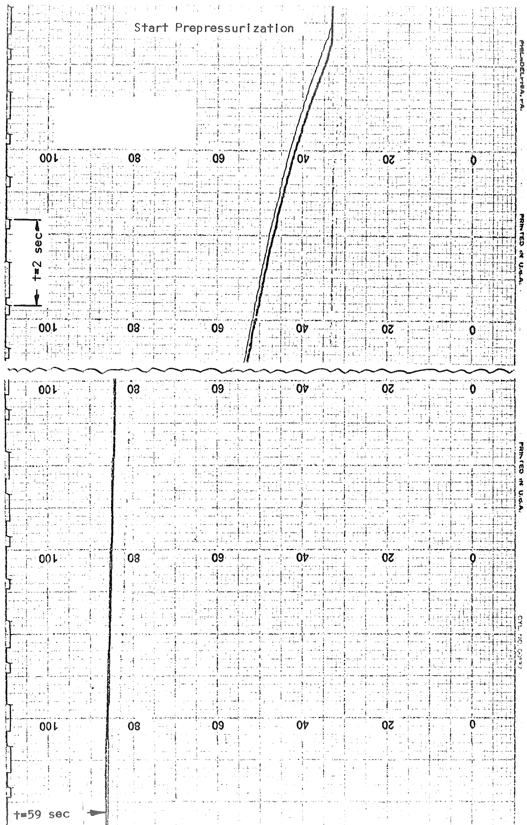
Figure 66. Control System Response - 90% Ullage - Prepressurization
