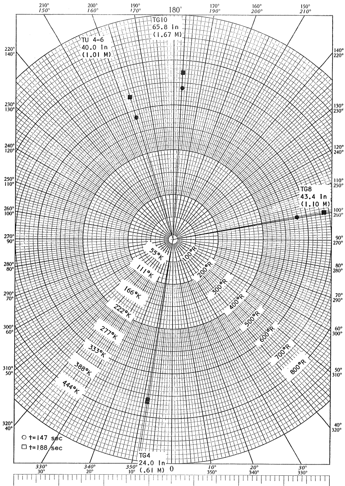
Figure 88. Radial Temperature Distribution - Test 8
