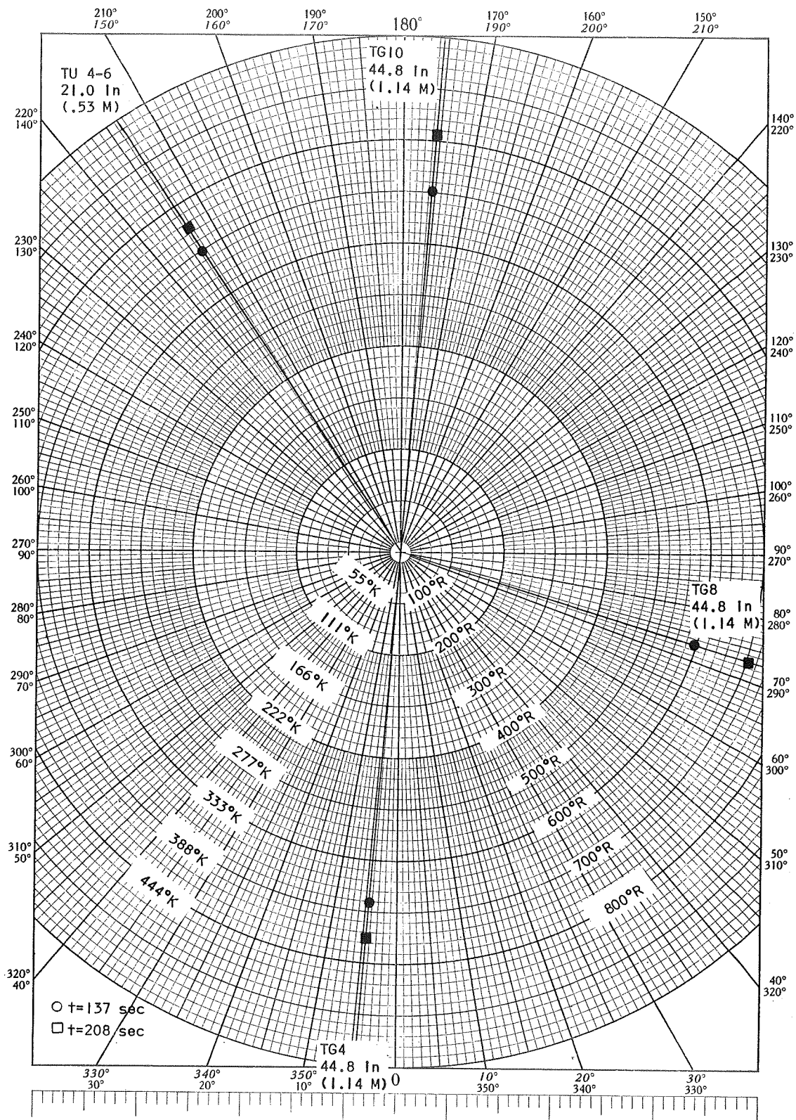
Figure 86. Radial Temperature Distribution - Test 6
