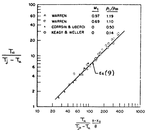
Figure 5. Comparison of Laufer's Analysis with Experimental Data
