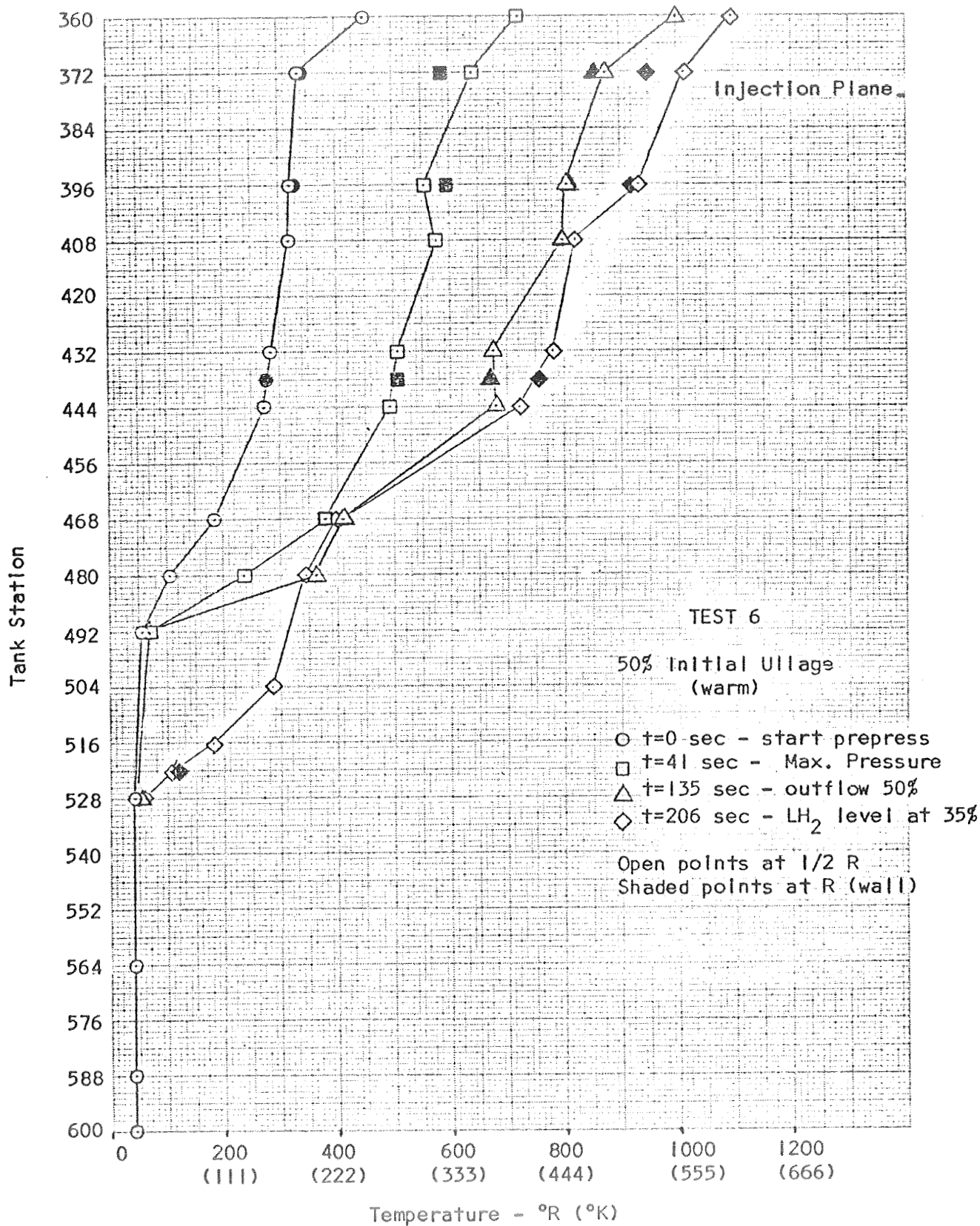
Figure 74. Axial Temperature Distribution for Test 6
