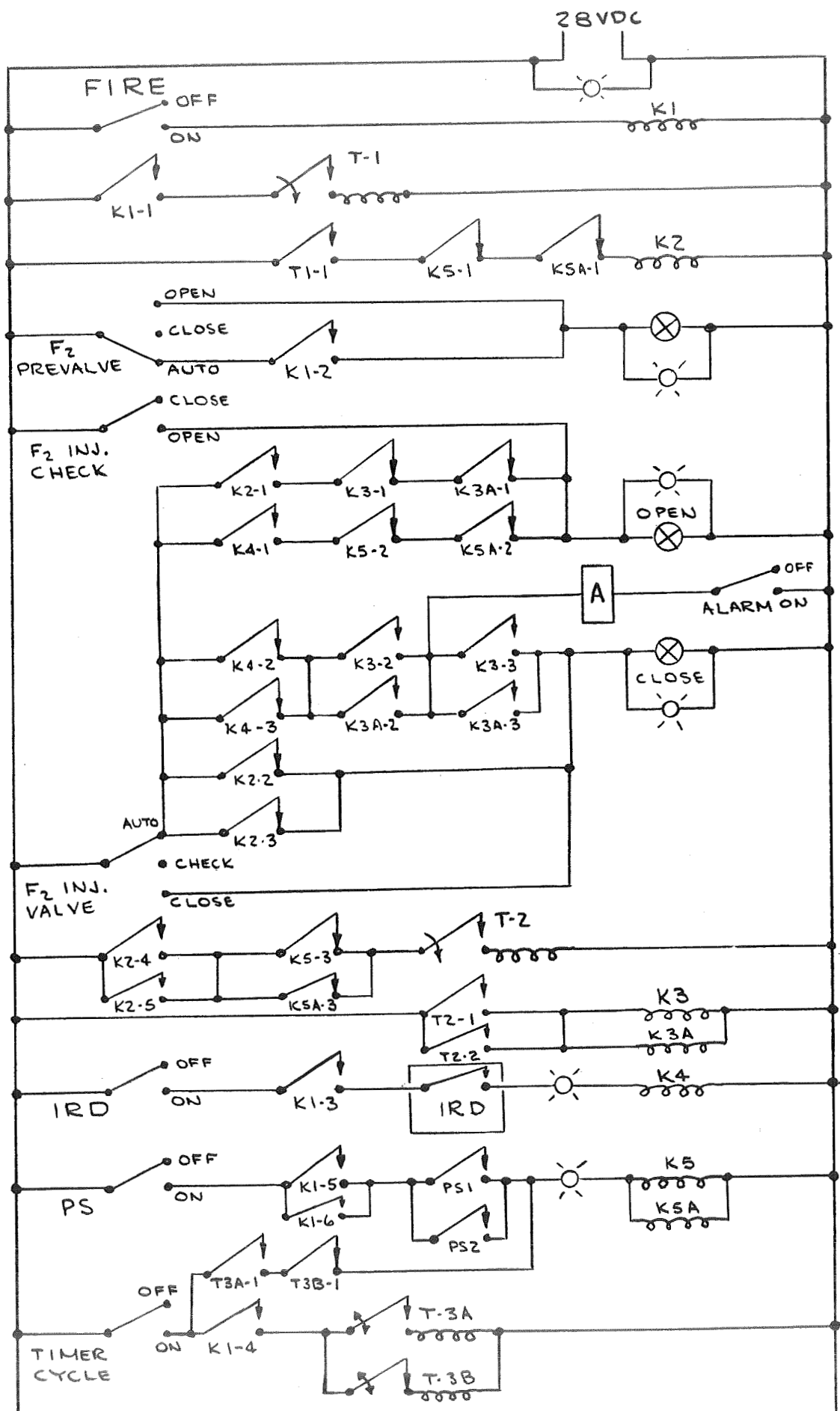
Flaure 33. MTI Control System Schematic
