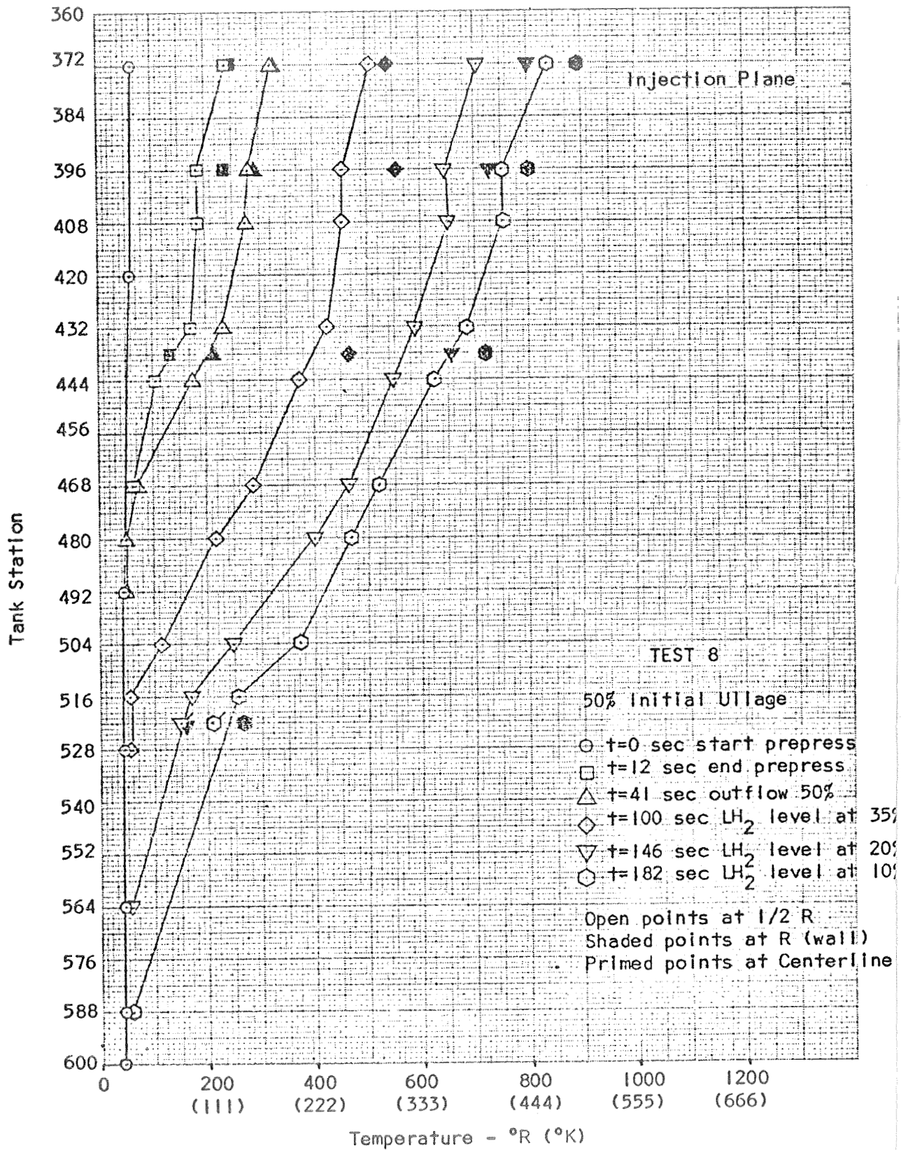
Figure 76. Axial Temperature Distribution for Test 8
