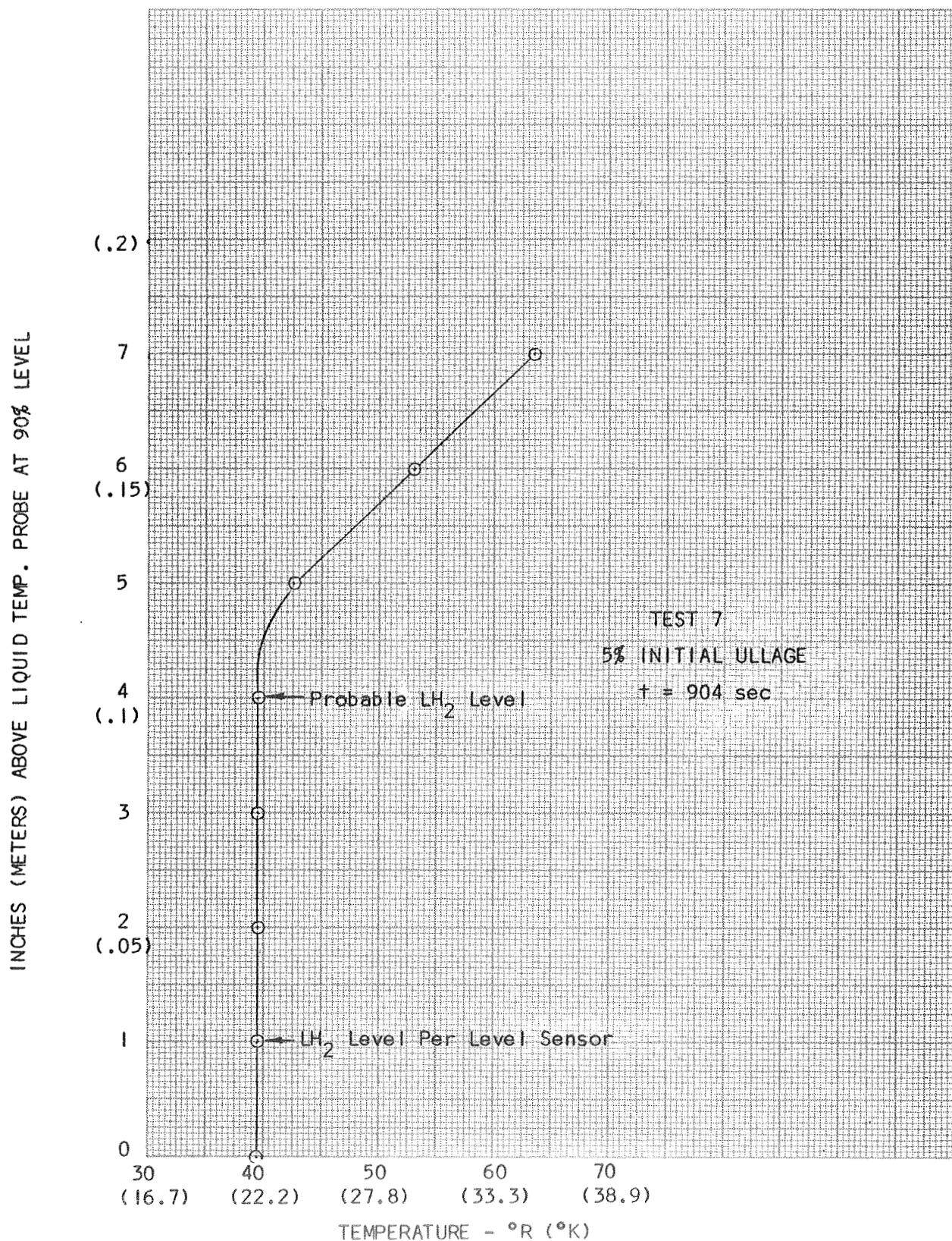
Figure 92. Temperature Gradient at 90% Level-Test 7
