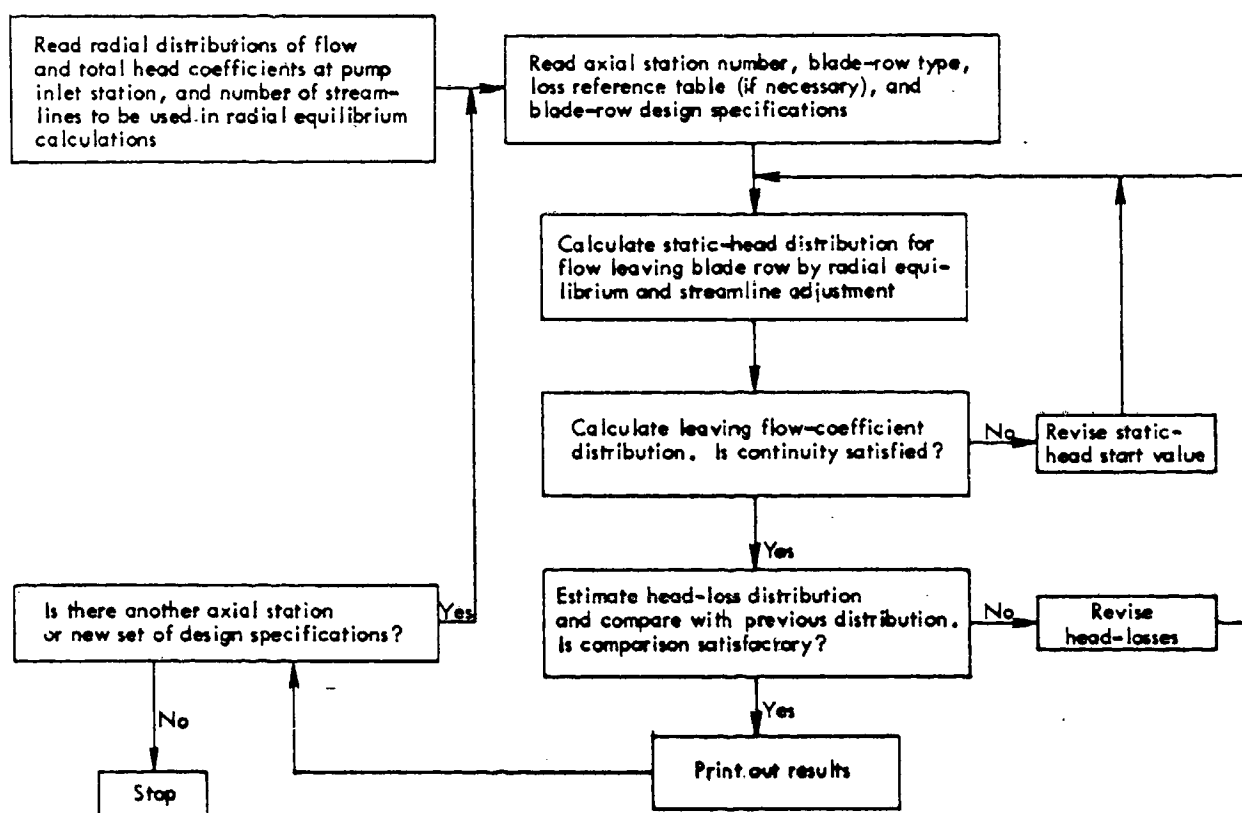
Fig. 4. General scheme of computer program radial equilibrium solution method.
