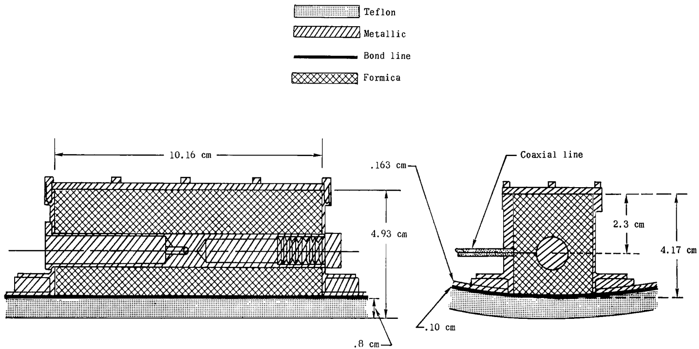
(a) L-band.
