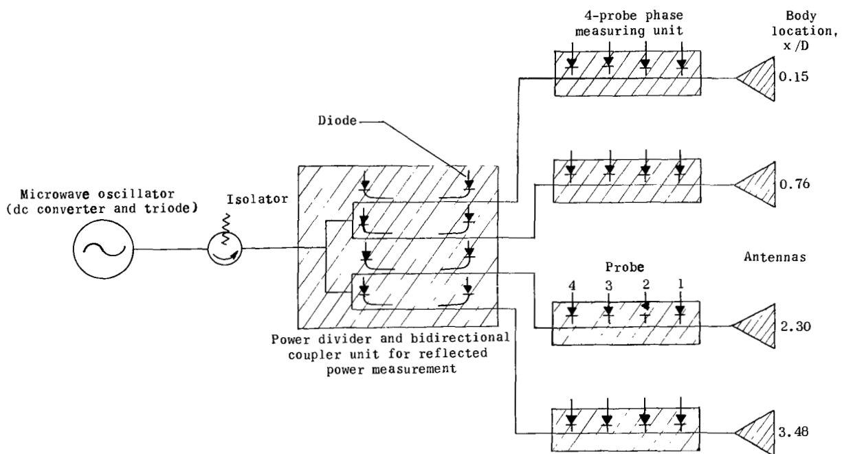
Figure 6.- S-band reflectometer block diagram.
