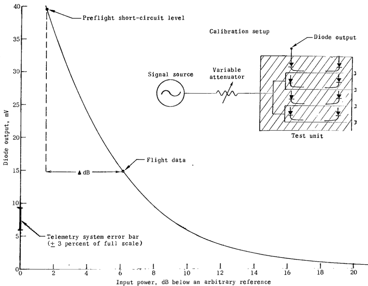
Figure 14.- Diode calibration curve for S-band reflected signal (typical) at station 1. \Gamma_p = 10^{-\frac{\Delta \text{dB}}{10}} .
