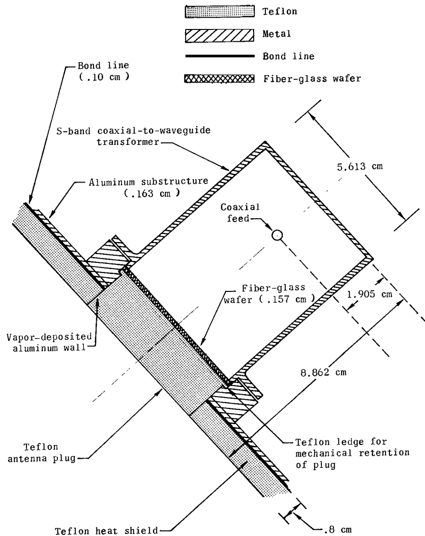
(b) S-band.
