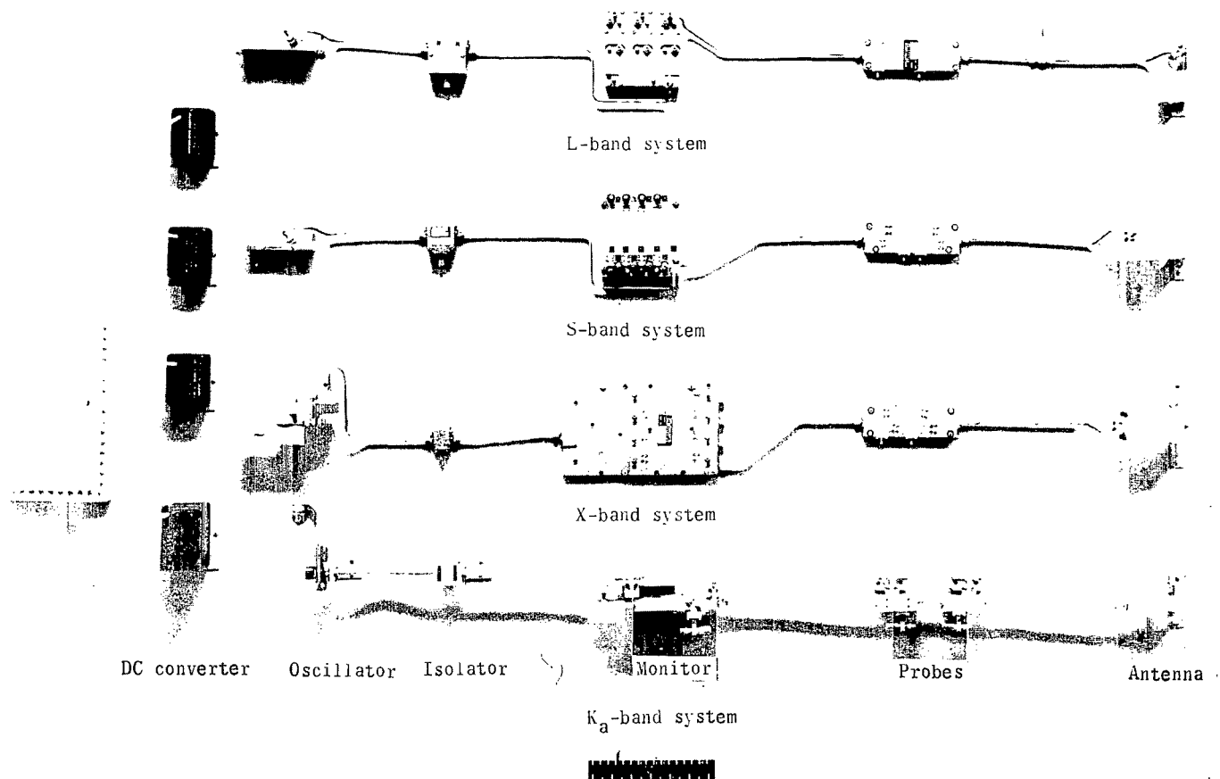
Figure 7.- Reflectometer flight components (only one probe unit and antenna shown for each frequency).
