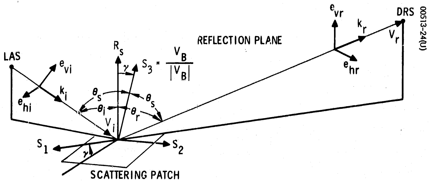
Figure 2-23. Depolarization Geometry
