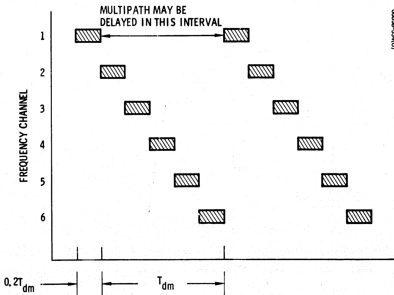
Figure 4-8. Frequency Hopping
