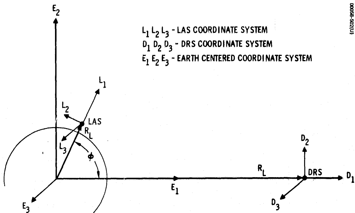
Figure 2-3. Coordinate Systems
