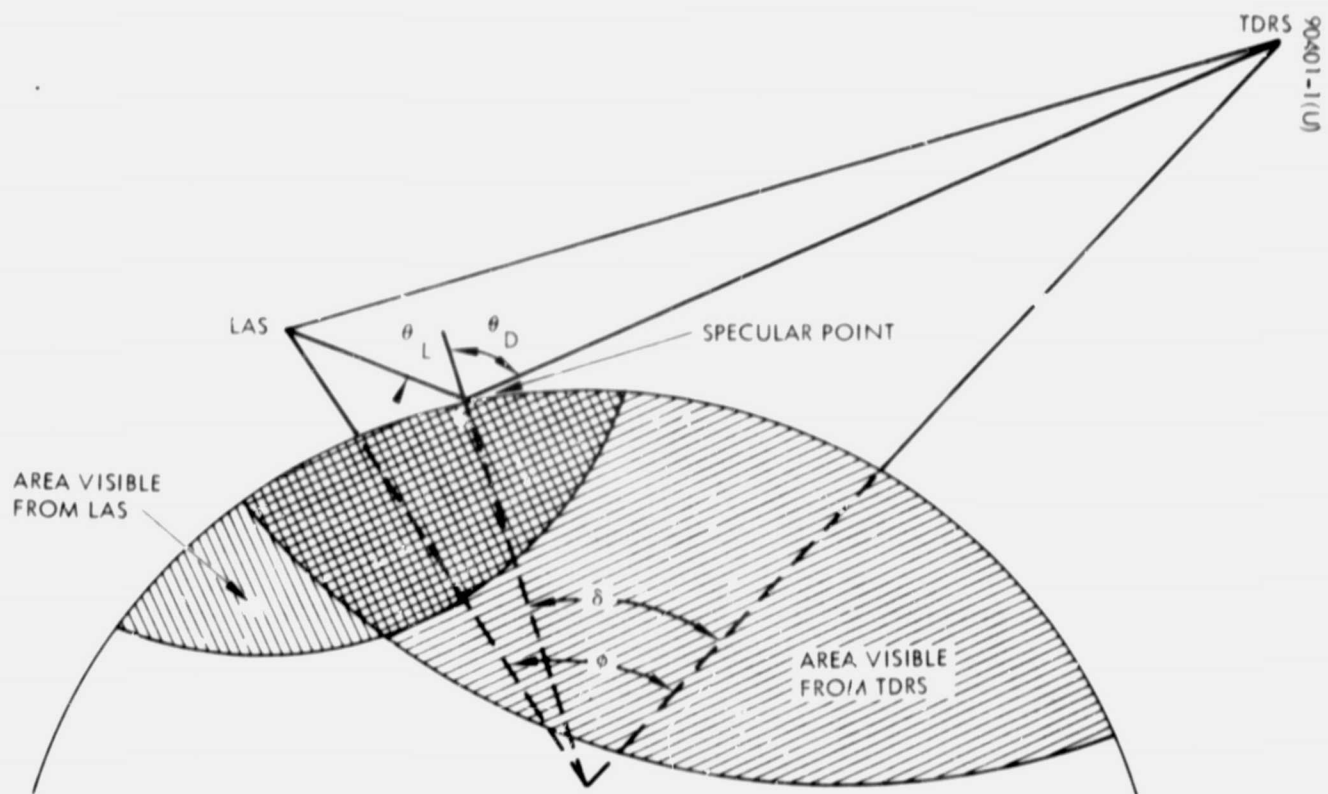
Figure 1-1. LAS-DRS Geometry
