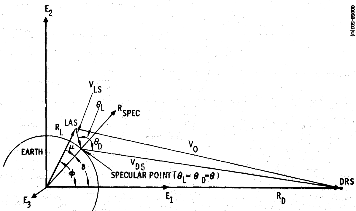
Figure 2-4. Specular Point Quantities
