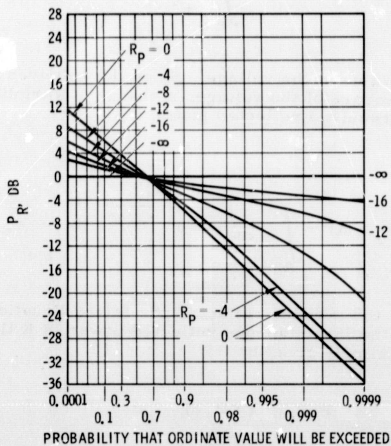
Figure 3-9. Inverse Probability Distribution of P_R
