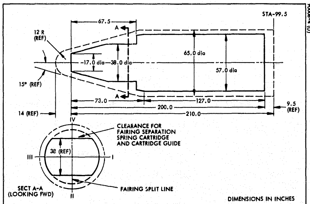
Figure 9-1. Improved Thor-Delta Booster Shroud
