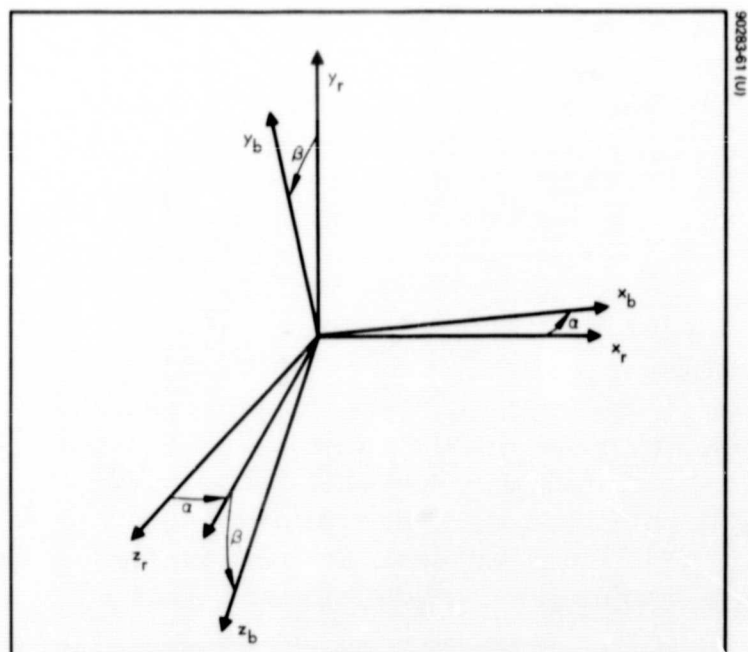
Figure 7-5. Relation Between Body and Earth Reference Coordinate Systems
