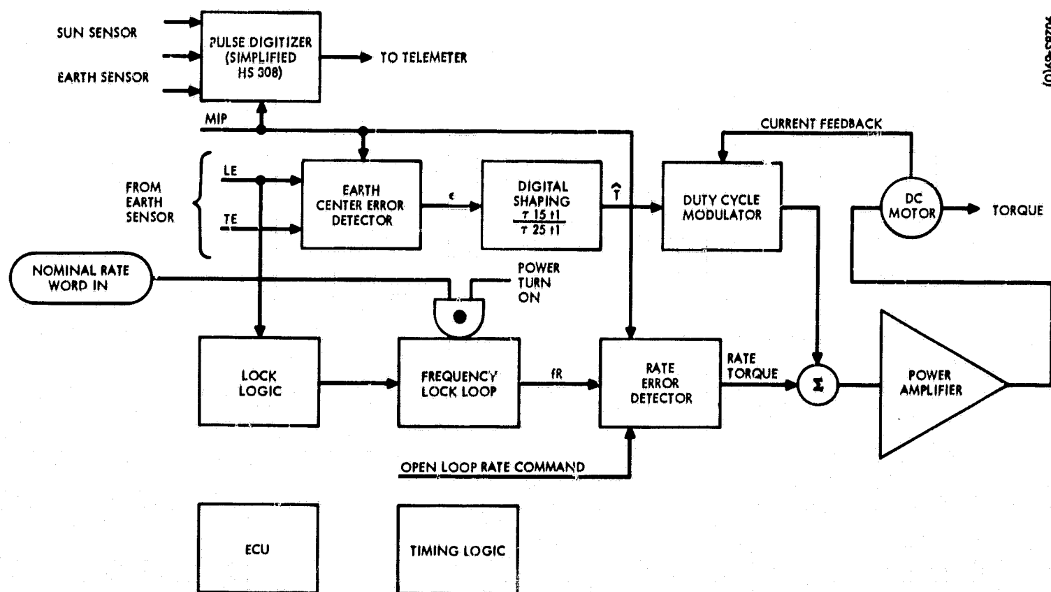
Figure 7-13. Control Electronics Mechanization
