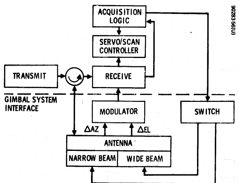
Figure 6-18. Acquisition/Antenna Control System
