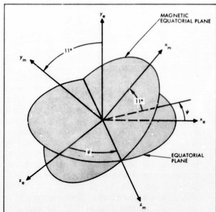
Figure 7-6. Magnetic and Inertial Reference Coordinate Systems
