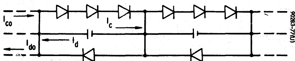
Figure 8-5. Battery Cell Protection Method
