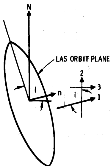
Figure 2-2. Three-Gimbal System
