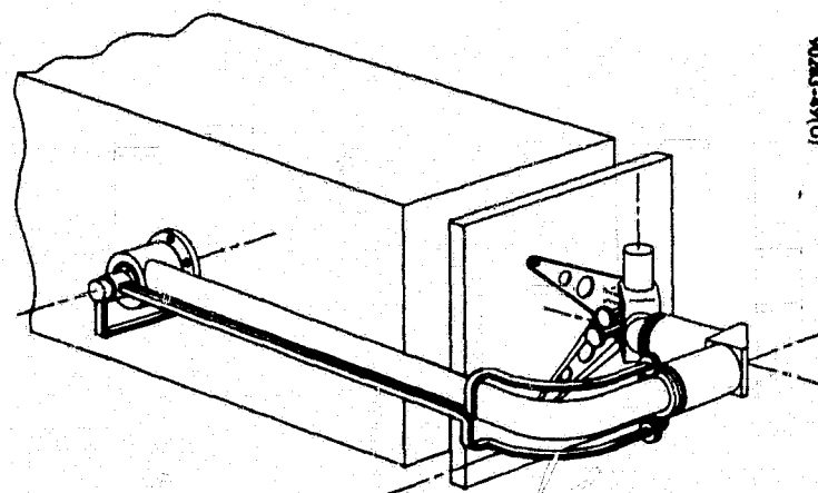
Figure 6-11. DTS Antenna in Stowed Position
