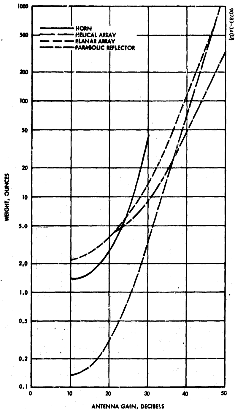
Figure 5-6. Antenna Weight Comparison at 15 GHz
