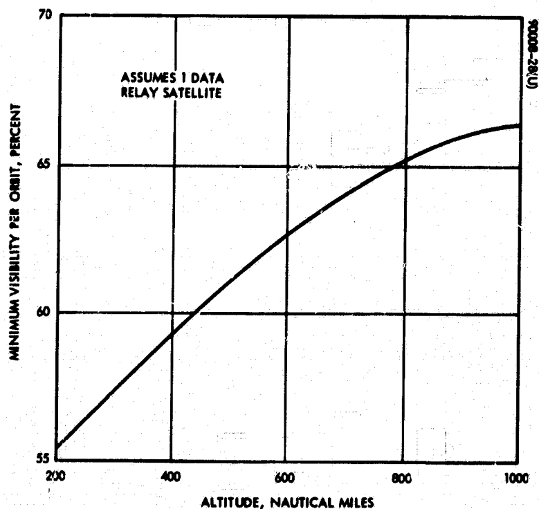
Figure 4-12. Minimum Visibility of LAS by DRS
