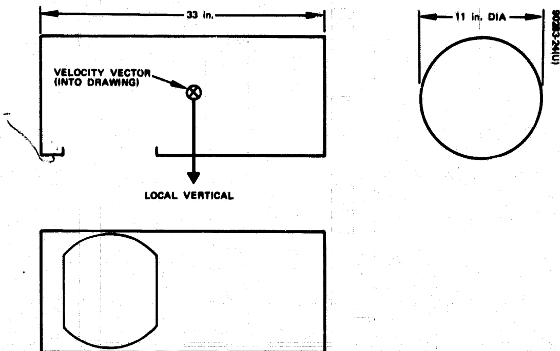
Figure 3-3. Multispectral Scanning Camera Dimensions
