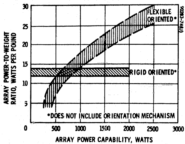
Figure 8-2. Comparison of Solar Array Specific Power Ratios
