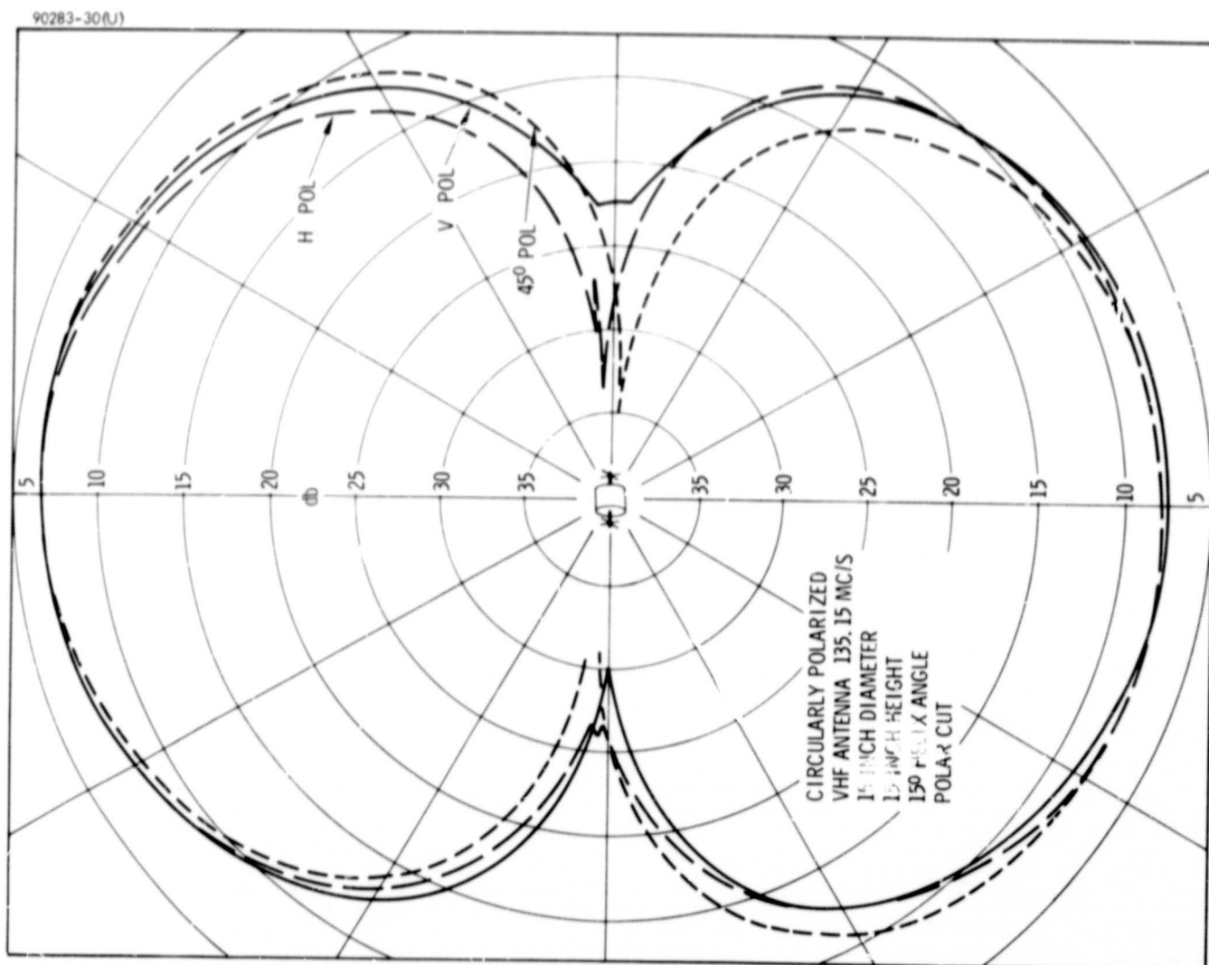
Figure 5-2. Antenna Pattern
