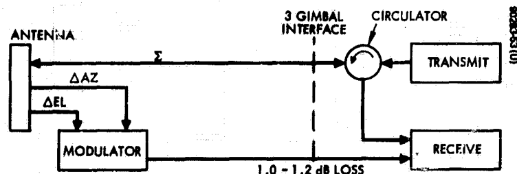
Figure 6-15. Double RF Feed
