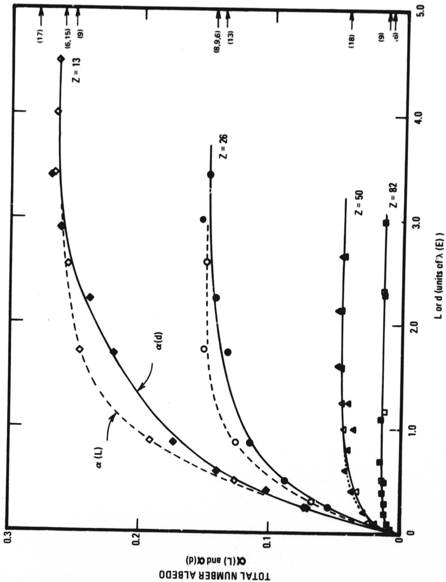
TOTAL NUMBER ALBEDO AS A FUNCTION OF L AND d FOR E_0 = 0.662 MeV AND NORMAL INCIDENCE
