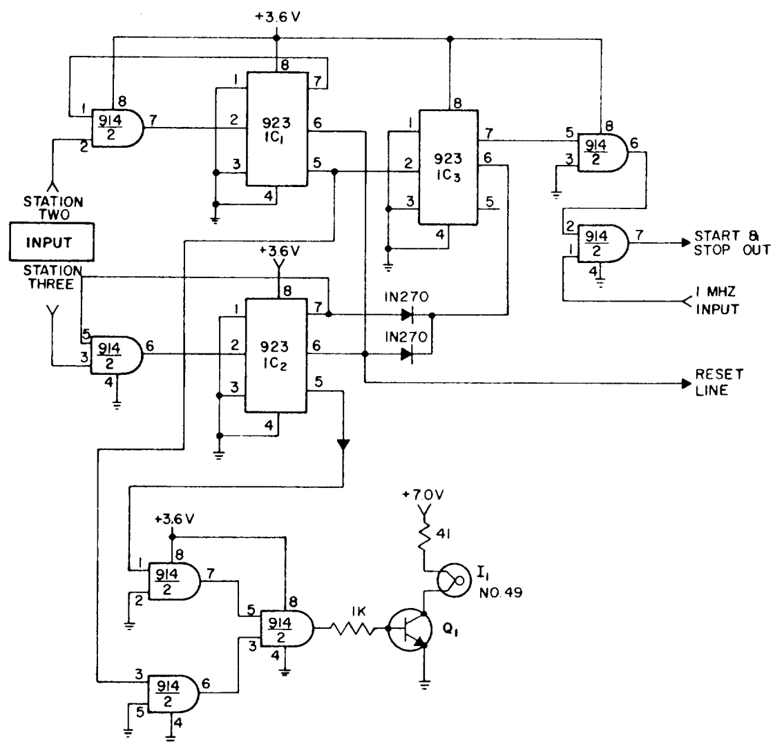
FIGURE-7 VELOCITY MEASURING SYSTEM — INPUT GATE &amp; READY INDICATOR
