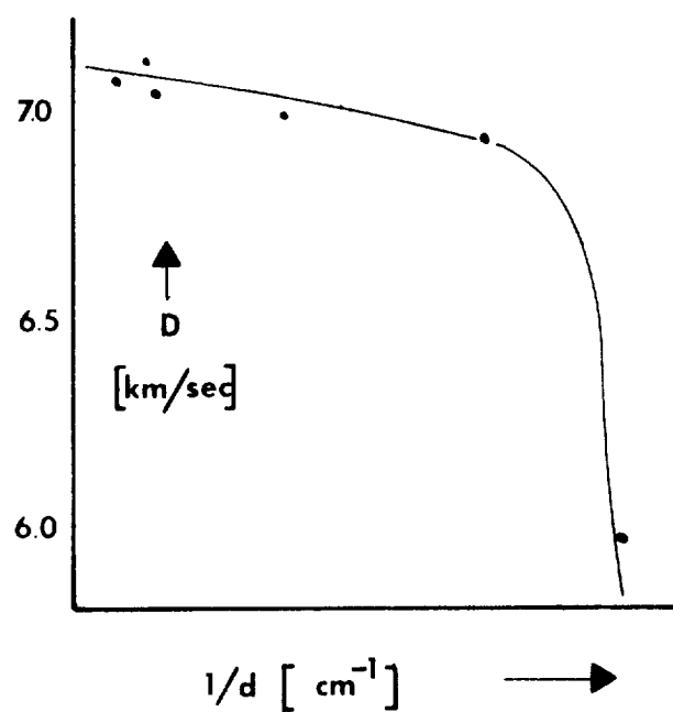
Detonation rate of PETN sheets ( \Delta \approx 1.4, 15\% natural rubber) as a function of inverse thickness d^4
