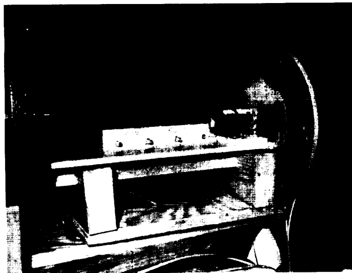
Instrument tray and photodiode velocity measuring system
