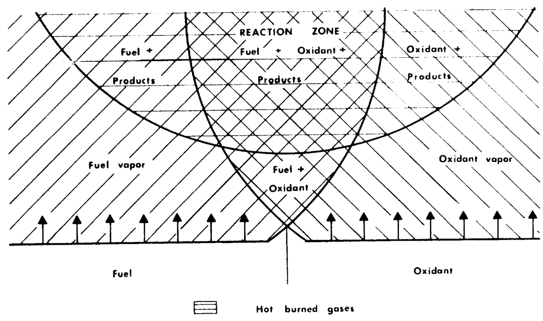
Compositional structure of a diffusion flame 27
