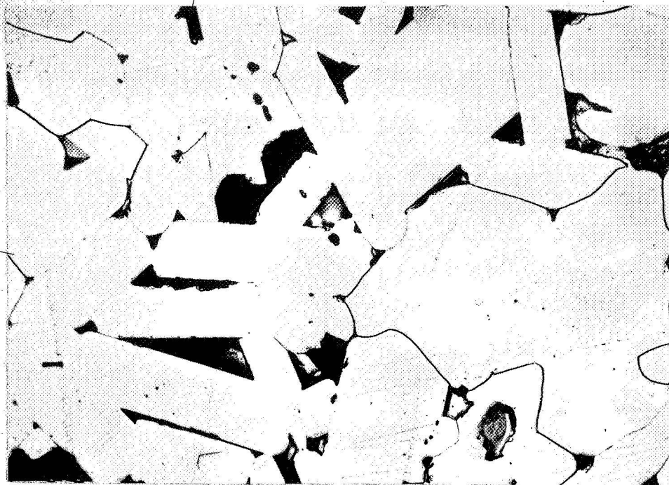
Figure 7. Etched Microstructure of SiC with 1 w/o \text{Al}_2\text{O}_3 and 3 w/o C. Billet 1293, Density 3.25 gm/cc, Grain Size 45 \mu .
