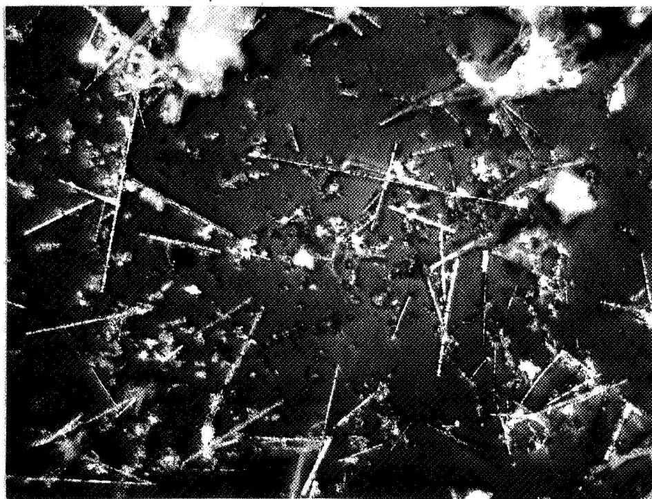
Figure 7. Etched Microstructure of SiC with 1 w/o \text{Al}_2\text{O}_3 and 3 w/o C. Billet 1293, Density 3.25 gm/cc, Grain Size 45 \mu .
