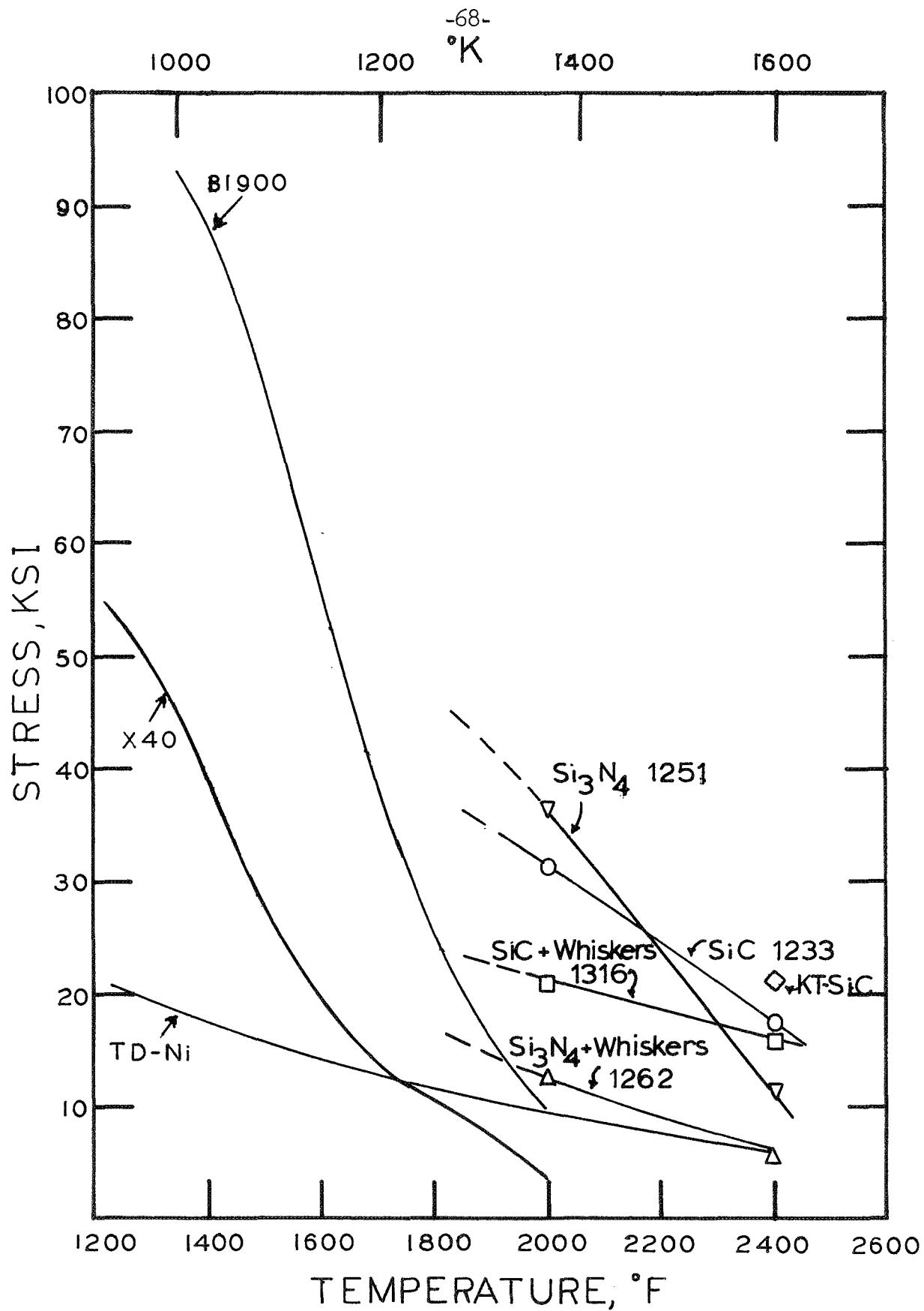
Figure 39. 100 Hour Rupture Stress versus Temperature for a Number of Ceramic and Metal Alloy Systems.
