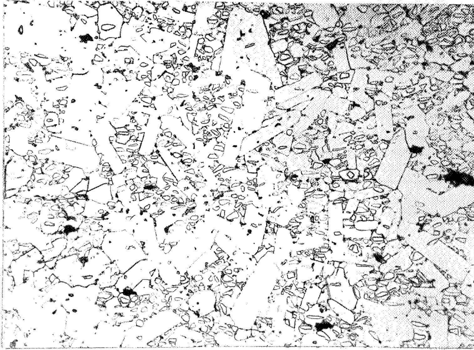
Figure 5. Etched Structure of SiC with 3 w/o \text{Al}_2\text{O}_3 and 1 w/o C. Billet 1237, Density 3.08 gm/cc, Grain Size 8 \mu .
