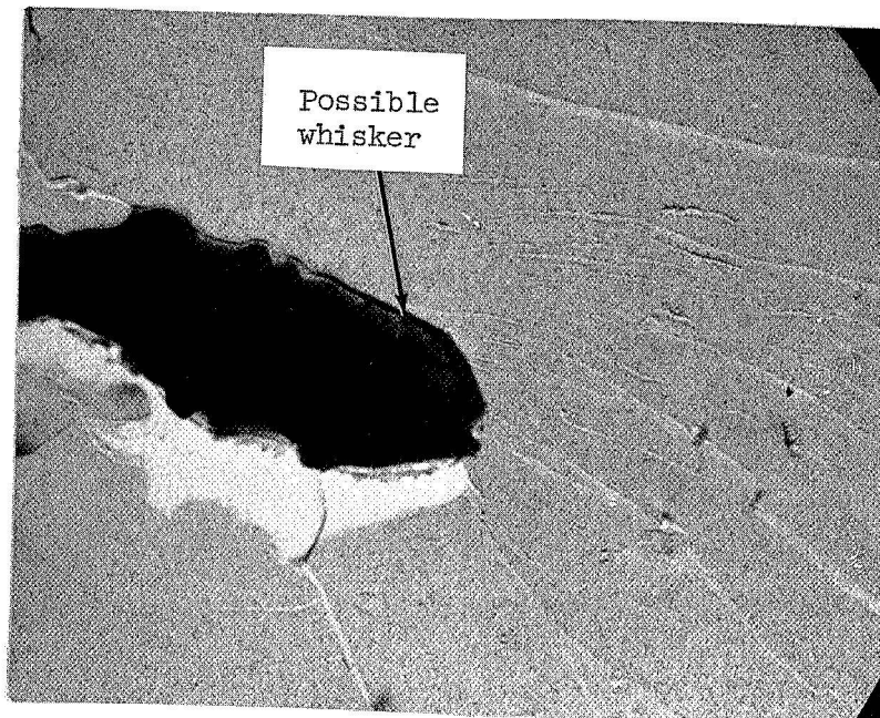
Figure 31. Fractograph of Si 3 N 4 Billet 1251 Broken at 2000°F (1366°K). Density 3.19 gm/cc, Grain Size .2 μ - Small, 2.5 μ Large.
