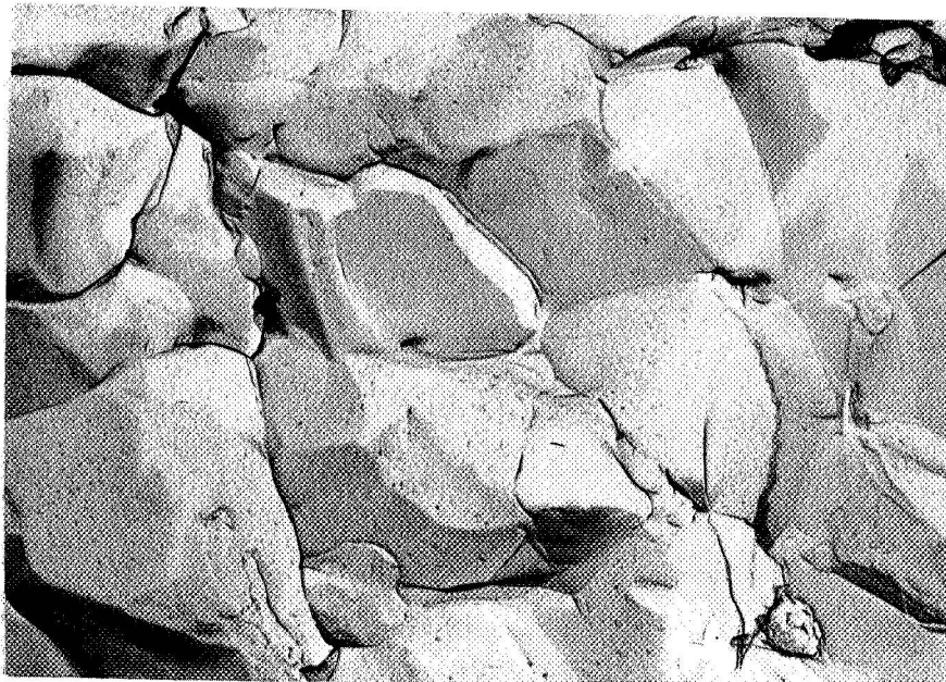
Figure 29b. Fractograph at 2400°F (1589°K) for Billet 1233. Density 3.14 gm/cc, Grain Size 3.3 \mu .
