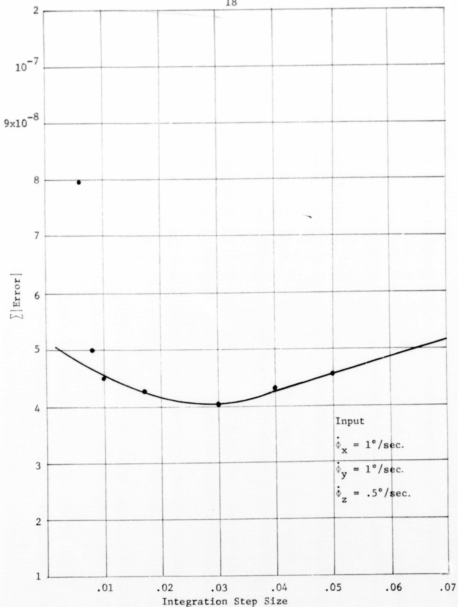
Figure 6. Error vs. integration step size for fixed point mode of operation.
