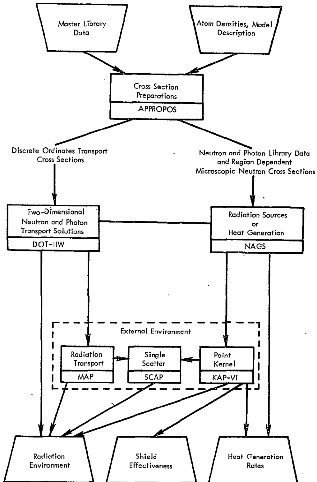
Figure 1-2. Flow Chart for Detailed Radiation Analysis
