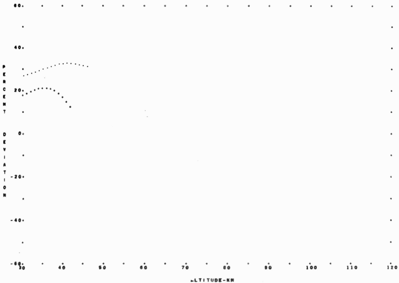
FIGURE 37- COMPARISON OF DIURNAL VARIATIONS FOR THE SUMMER EXTREME, ... DIURNAL TRANSITION ... DAYTIME
