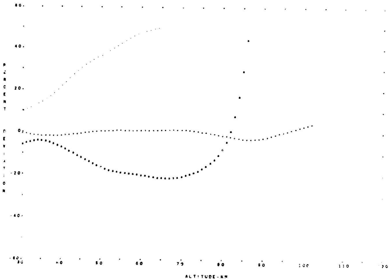
FIGURE 11 - COMPARISON OF DIURNAL VARIATIONS FOR NATURAL MEAN, SUBARCTIC STRATIFICATION, AND DIURNAL TRANSITION --- DIURNAL TRANSITION --- DAYTIME --- NIGHTTIME
