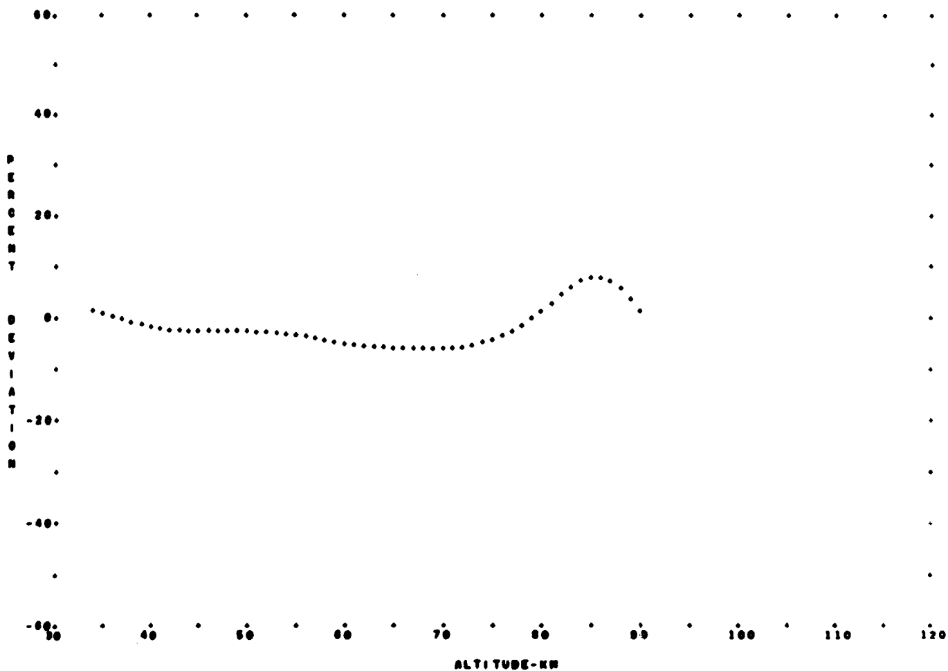
FIGURE 26 - COMPARISON OF DIURNAL VARIATIONS FOR THE SPRING, ... DIURNAL TRANSITION
