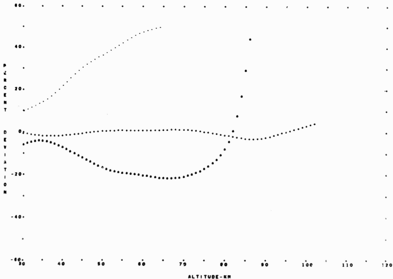
FIGURE 32 - COMPARISON OF DIURNAL VARIATIONS FOR THE ANNUAL MEAN, ... DIURNAL TRANSITION ... DAYTIME ... NIGHTTIME
