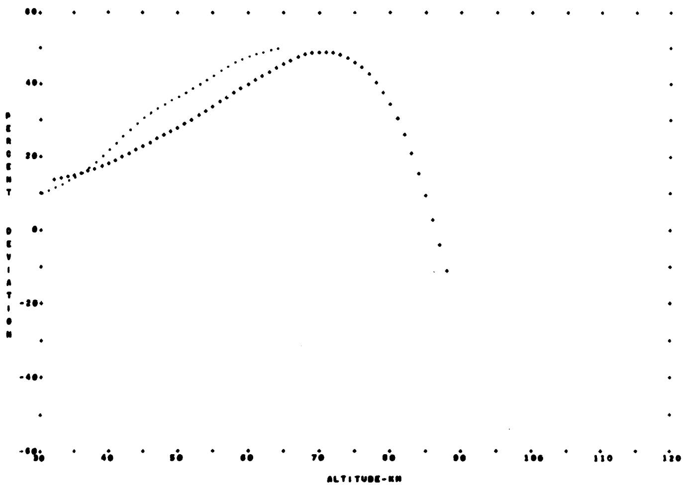
FIGURE 27 - COMPARISON OF DIURNAL VARIATIONS FOR THE SUMMER, SUBARCTIC STRATIFICATION ... DIURNAL TRANSITION ... DAYTIME
