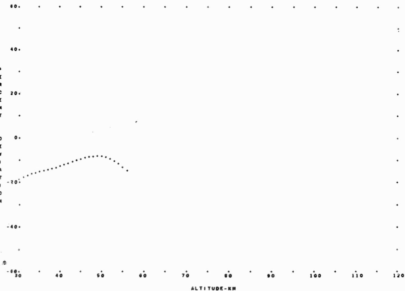
FIGURE 33 - COMPARISON OF DIURNAL VARIATIONS FOR THE SPRING, ... DIURNAL TRANSITION
