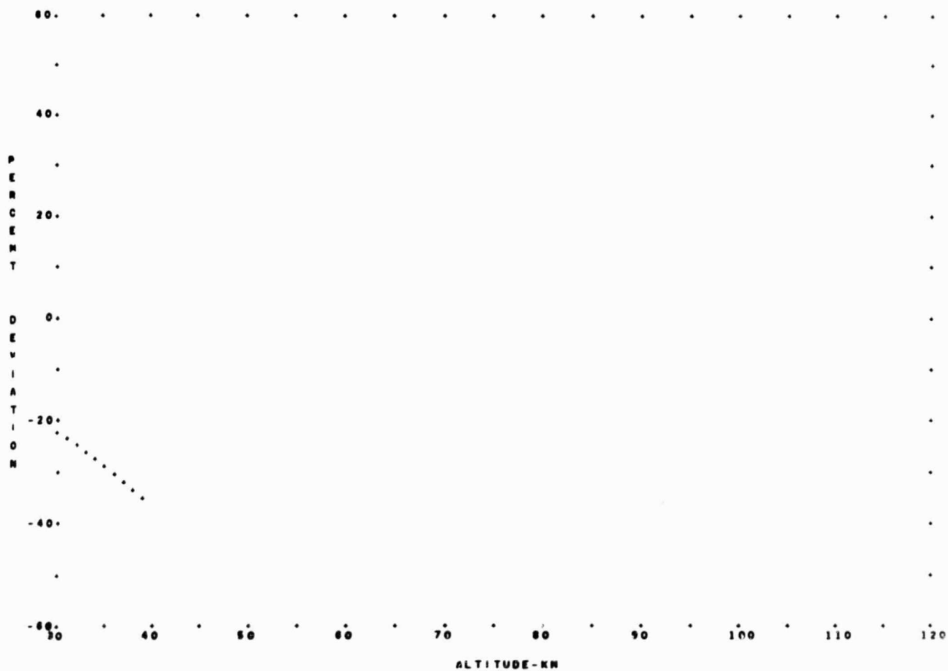
FIGURE 38- COMPARISON OF DIURNAL VARIATIONS FOR THE WINTER EXTREME, ... DIURNAL TRANSITION
