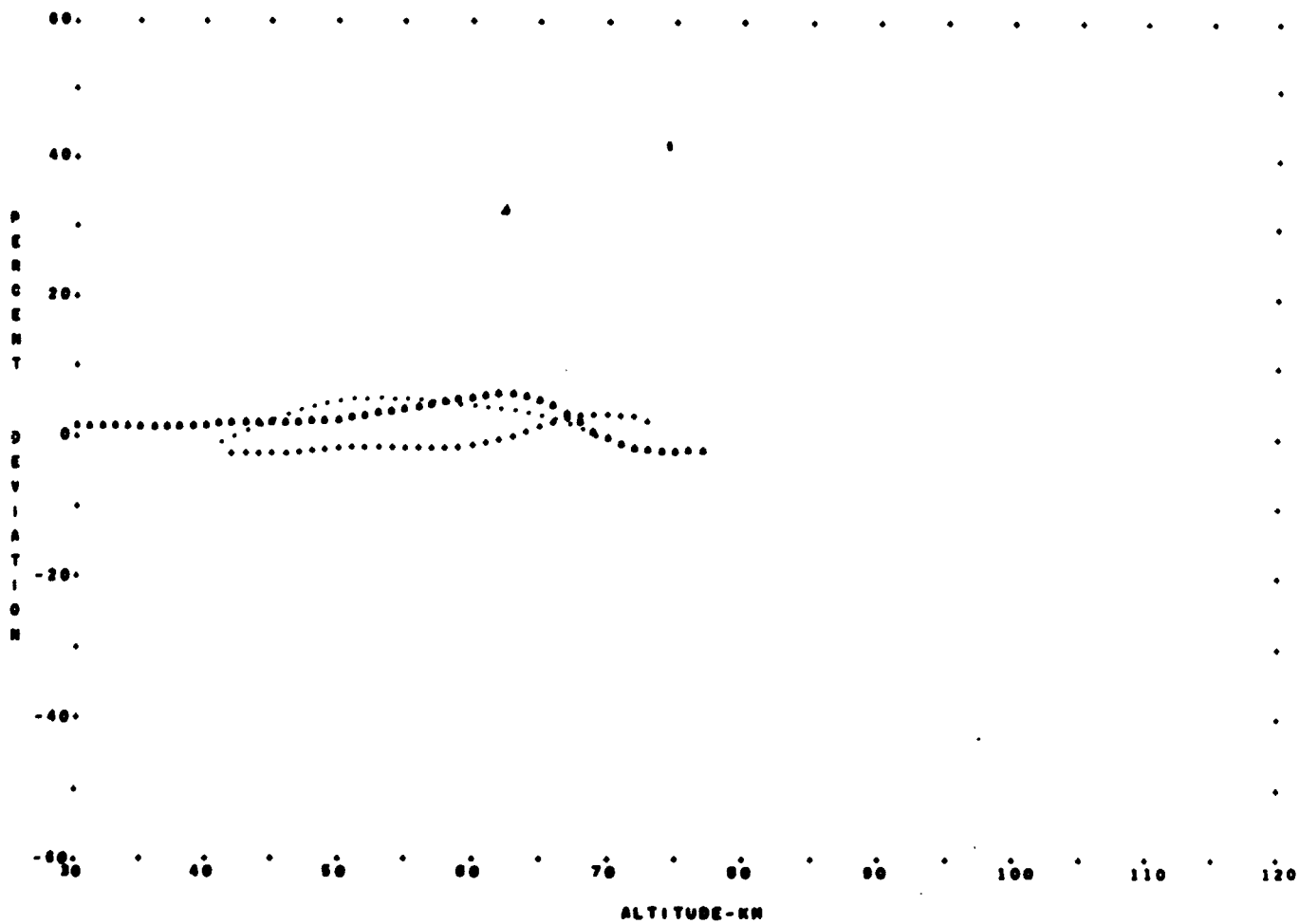
FIGURE 14 - COMPARISON OF DIURNAL VARIATIONS FOR THE SUMMER, ... DIURNAL TRANSITION ... DAYTIME ... NIGHTTIME
