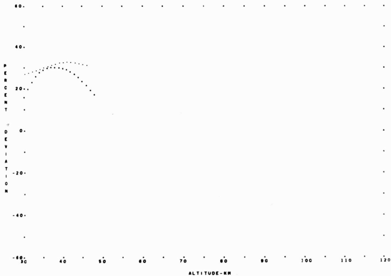
FIGURE 34 - COMPARISON OF DIURNAL VARIATIONS FOR THE SUMMER. +++ DIURNAL TRANSITION ... DAYTIME
