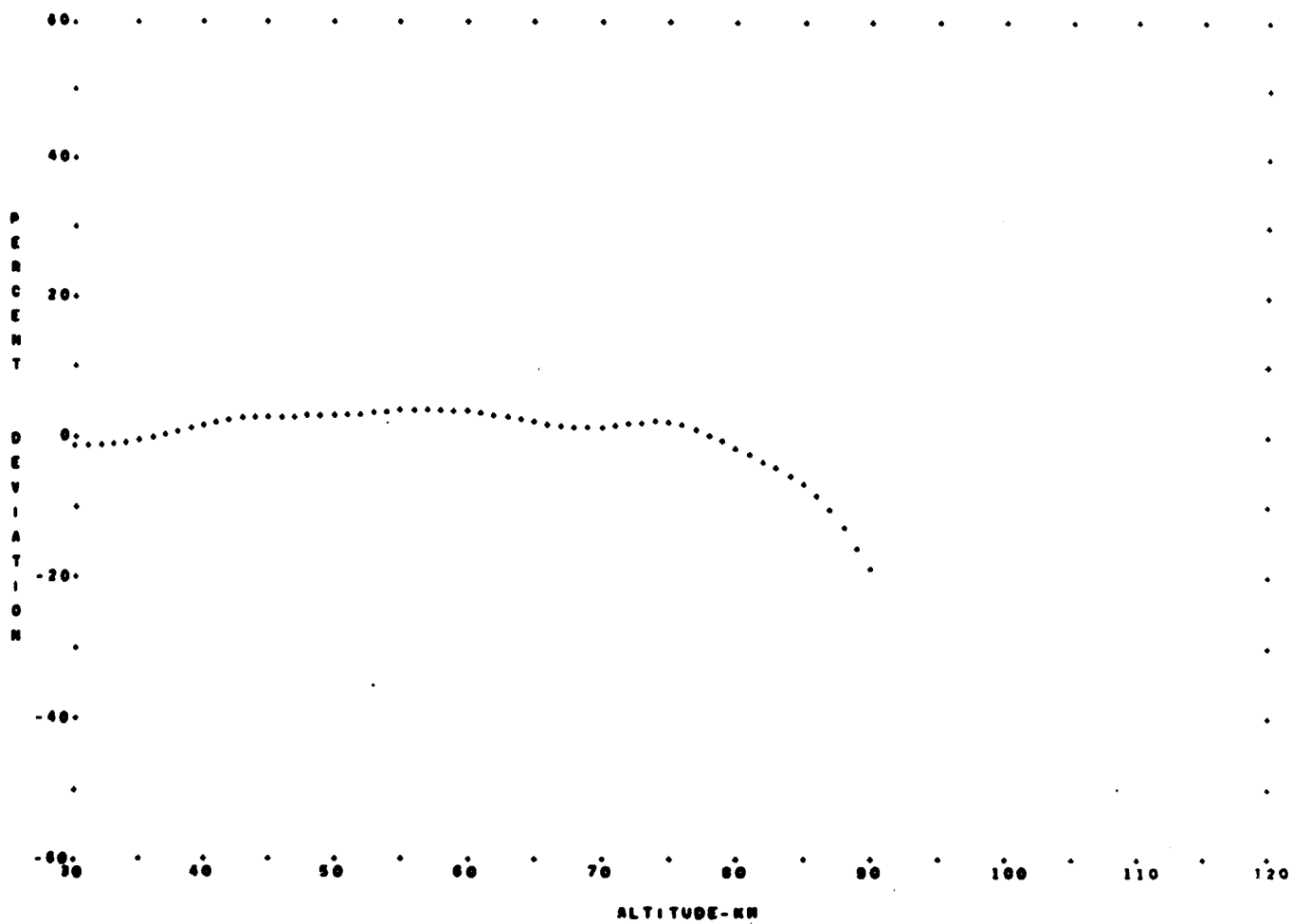
FIGURE 20 - COMPARISON OF DIURNAL VARIATIONS FOR THE SPRING, ... DIURNAL TRANSITION
