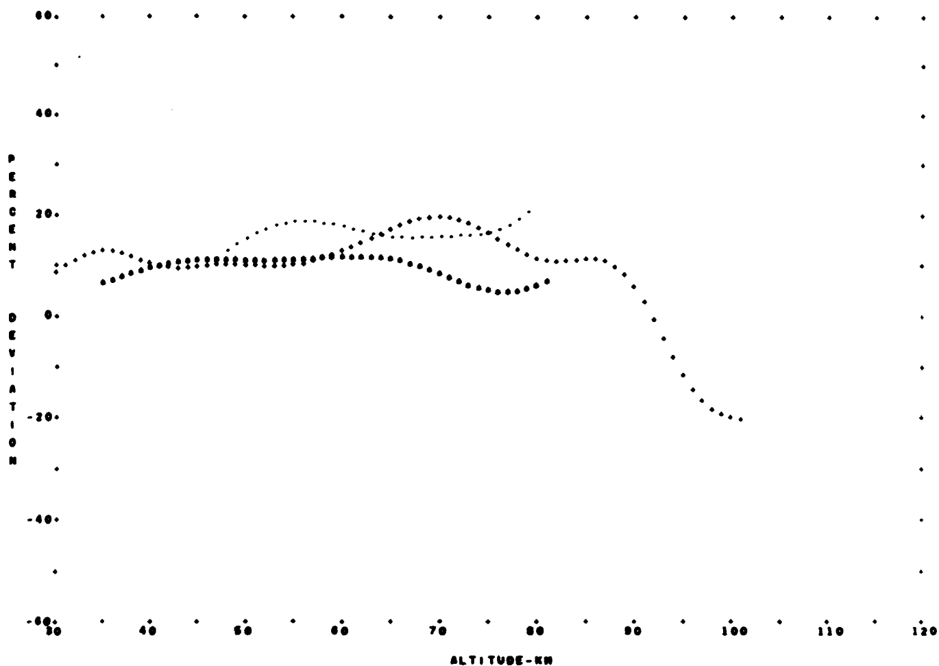
FIGURE 21 - COMPARISON OF DIURNAL VARIATIONS FOR THE SUMMER, ... DIURNAL TRANSITION ... DAYTIME ... NIGHTTIME
