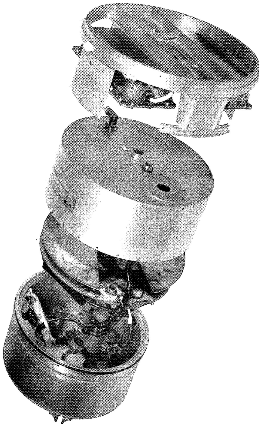
Figure 5. 10 keV - 1/2 Ampere Electron Accelerator - Exploded View 2.
