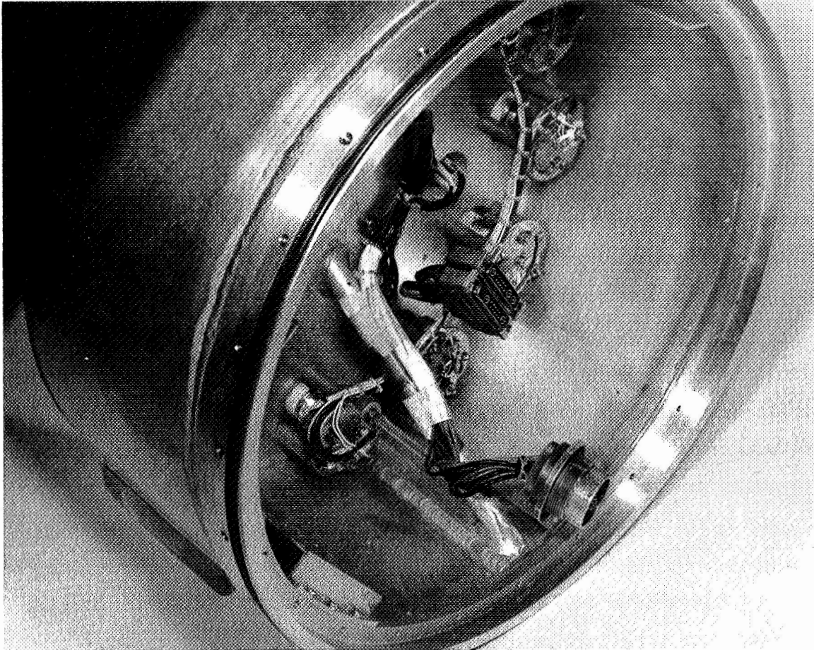
Figure 18. Gun Mounts and Cabling - Pressurized Side.
