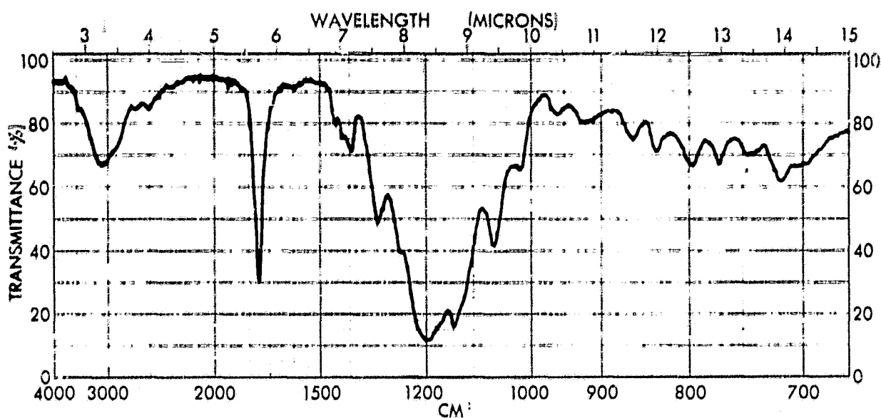
Figure 2 - Infrared Spectrum of 2-( 1' -Heptyloxy)-tetrafluoropropionic Acid (Liquid)
