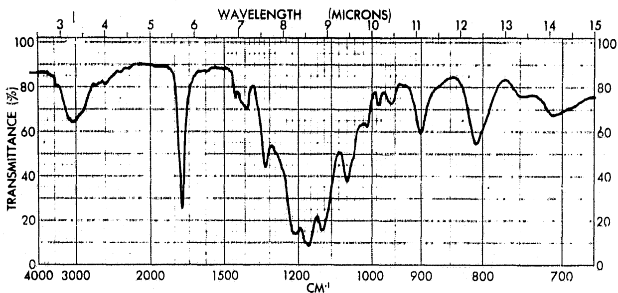
Figure 3 - Infrared Spectrum of 2-( 1' -Pentyloxy)-tetrafluoropropionic Acid (Liquid)
