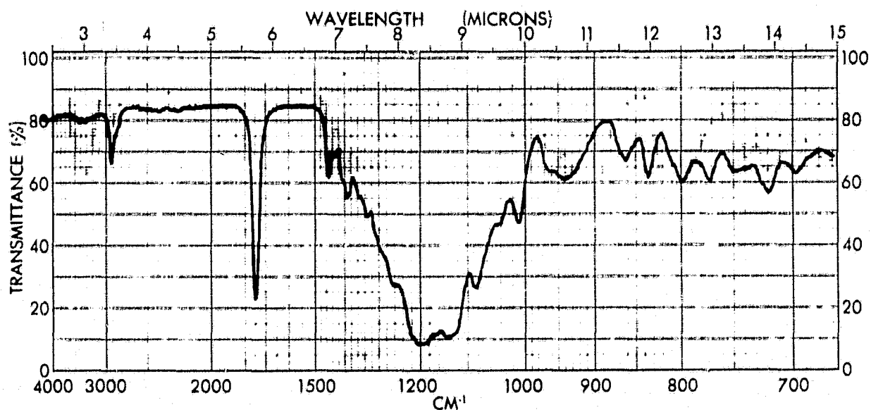
Figure 6 - Infrared Spectrum of Bis[2-(1-heptyloxy)-2,3,3,3-tetrafluoro-1-propyl] 3-Methylglutarate (Liquid)
