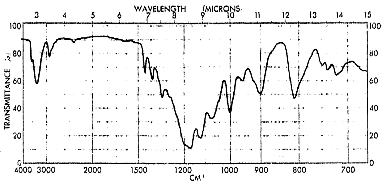
Figure 5 - Infrared Spectrum of 2-(1-pentyloxy)-2,3,3,3-tetrafluoro-1-propanol (Liquid)
