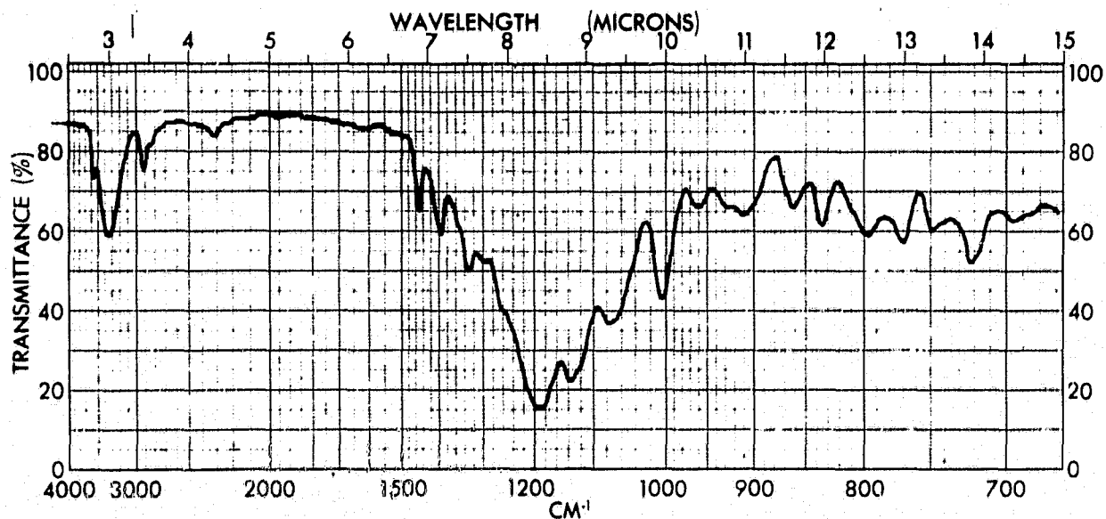
Figure 4 - Infrared Spectrum of 2-( 1' -Heptyloxy)-2,3,3,3-tetrafluoro-1-propanol (Liquid)
