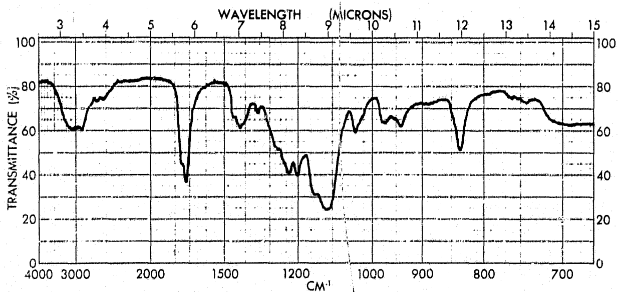
Figure 10 - Infrared Spectrum of \psi' -Pentyloxyacetic Acid (Liquid)
