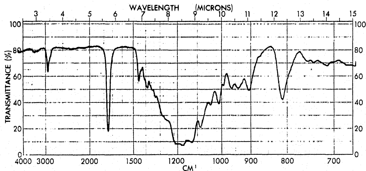
Figure 7 - Infrared Spectrum of Bis[2-(1-pentyloxy)-2,3,3,3-tetrafluoro-1-propyl] 3-Methylglutarate (Liquid)
