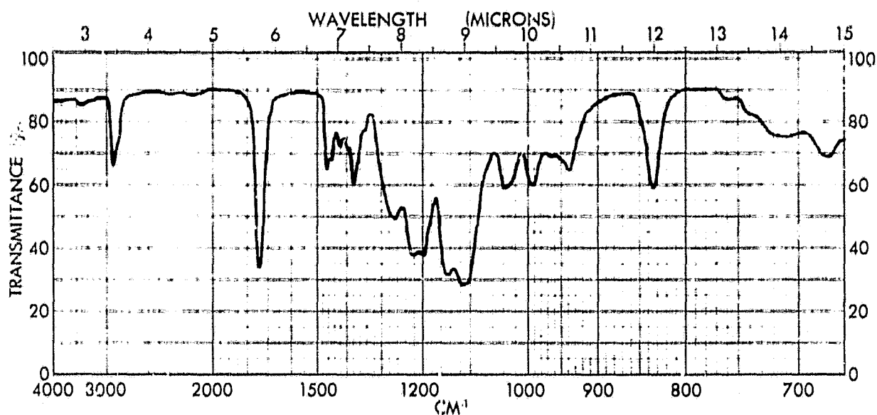
Figure 14 - Infrared Spectrum of 2,2-Dimethylolpropane Bis-( \eta -propyloxyacetate) (Liquid)
