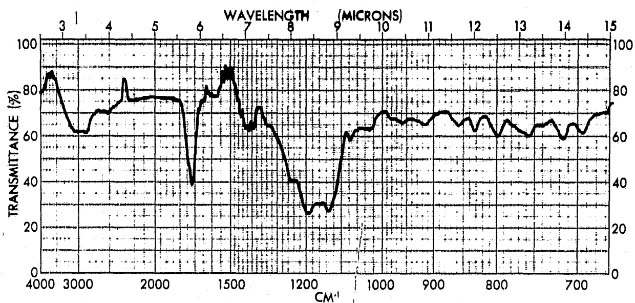
Figure 9 - Infrared Spectrum of \psi' -Propyloxyacetic Acid (Liquid)
