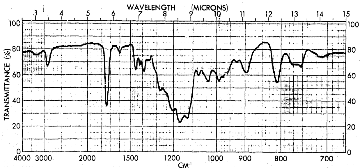
Figure 16 - Infrared Spectrum of 1,1,1-Trimethylolpropane Tris( \eta -pentyloxyacetate) (Liquid)
