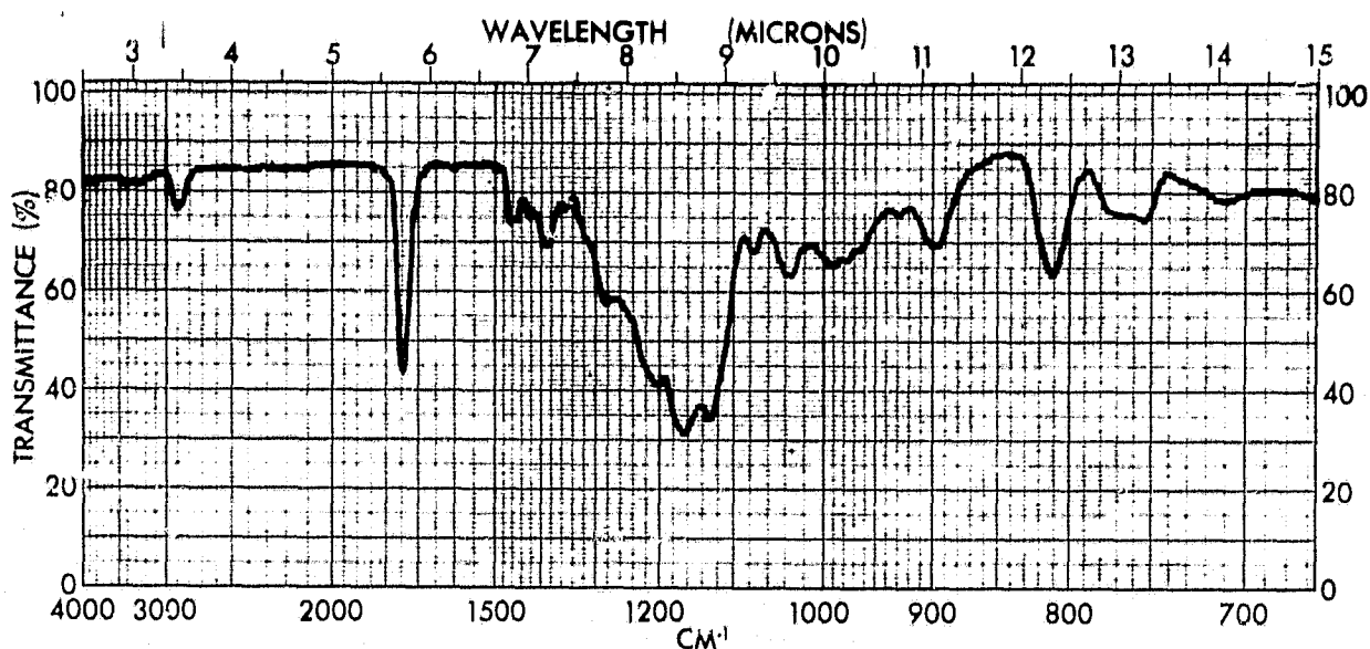
Figure 15 - Infrared Spectrum of 1,1,1-Trimethylolethane Tris( \eta -pentyloxyacetate) (Liquid)
