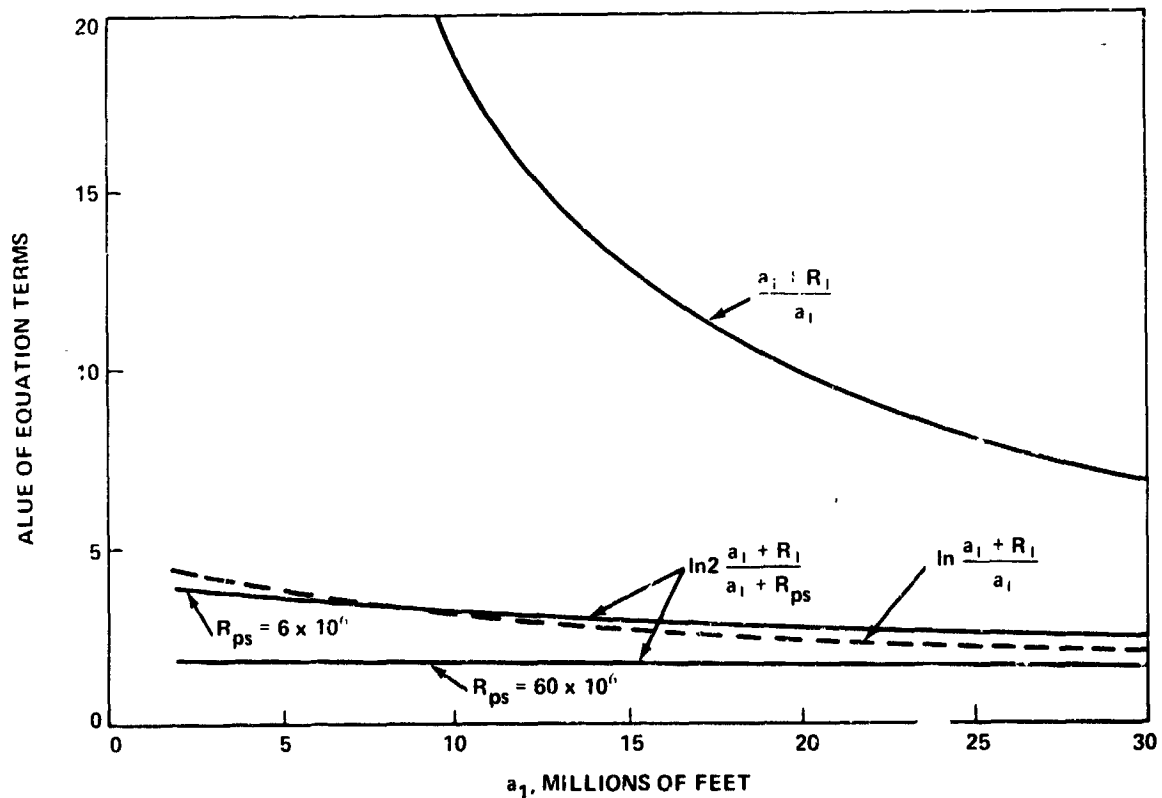
FIGURE 3 - VALUES OF THE TERMS IN EQN. (26) FOR LUNAR TRAJECTORIES
