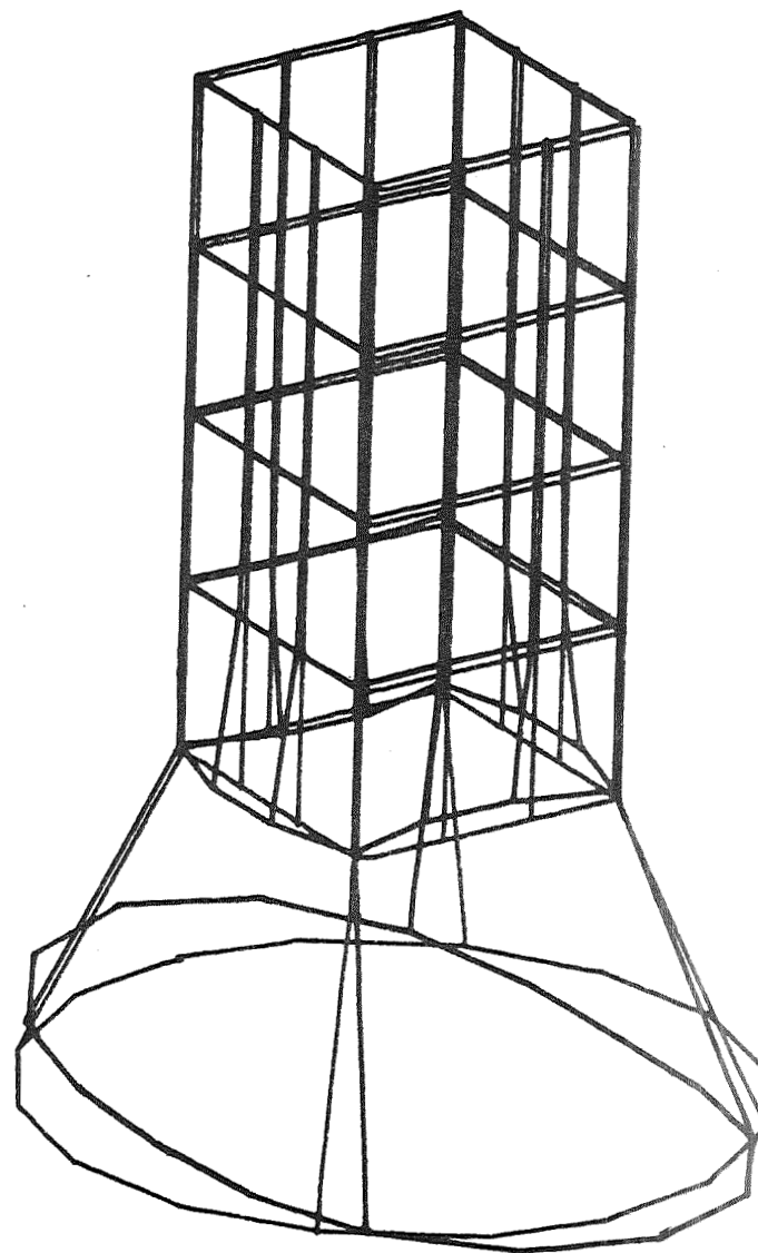
Fig. 5 Mode 13 Nat. Freq.=66cps
