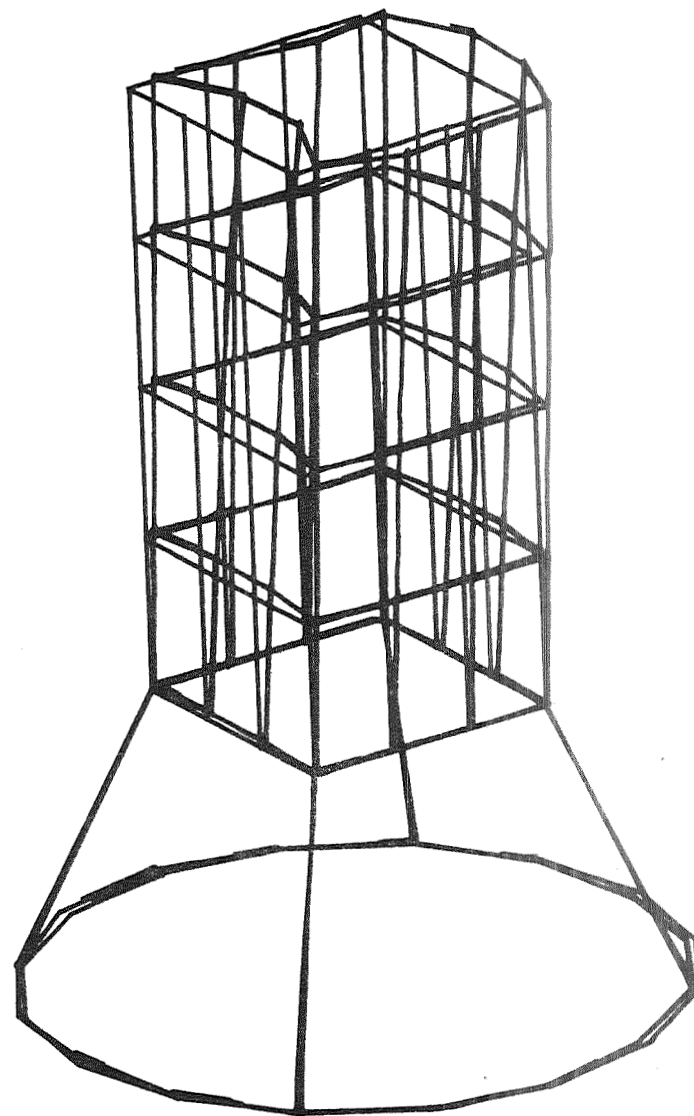
Fig. 8 Mode 30 Nat. Freq.=173cps
