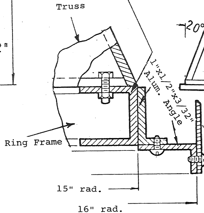
Fig. 9b. Stiffened Shroud Details
