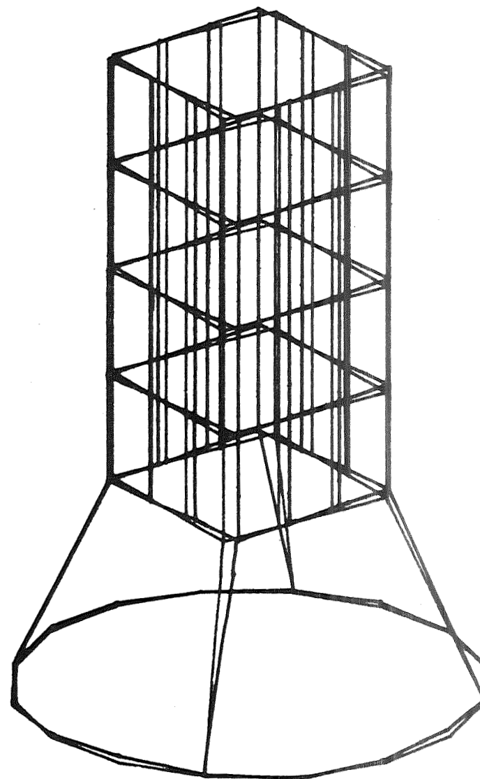
Fig. 3 Mode 10 Nat. Freq.=61cps
