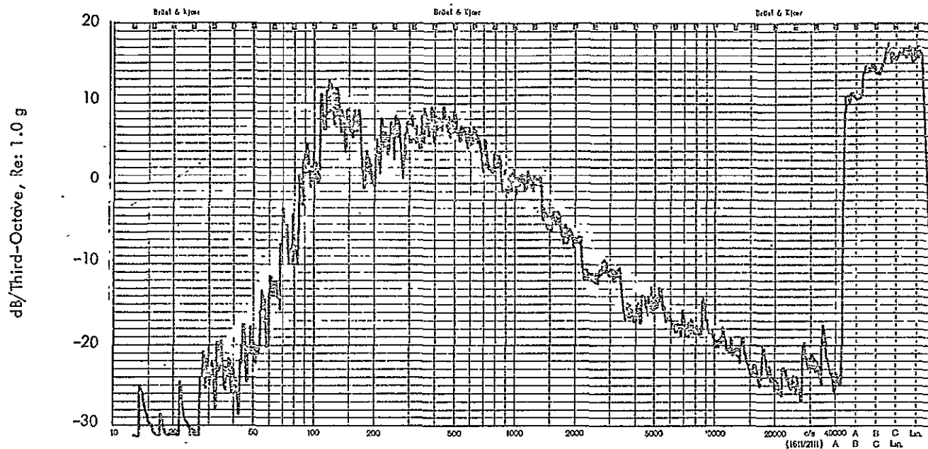
Figure B-49: Measured One-Third Octave Acceleration Response Levels, Experiment No. 6; Accelerometer A3
