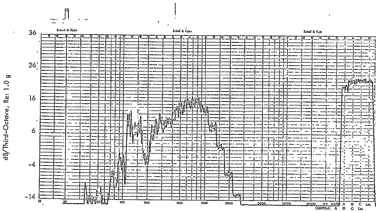
Figure B-6: Measured One-Third Octave Acceleration Response Levels, Experiment No. 1; Accelerometer A3
