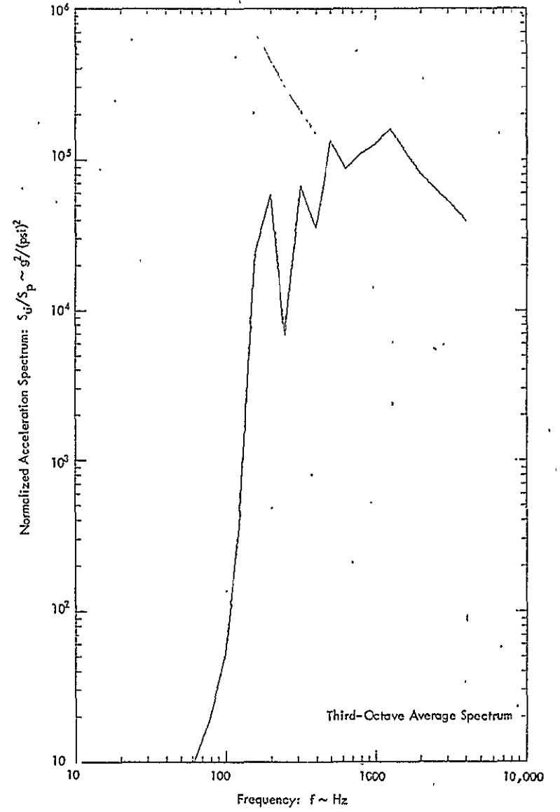
Figure A-13: Predicted Normalized Acceleration Response of Cylinder for Configuration No. 4; Q \approx 15
