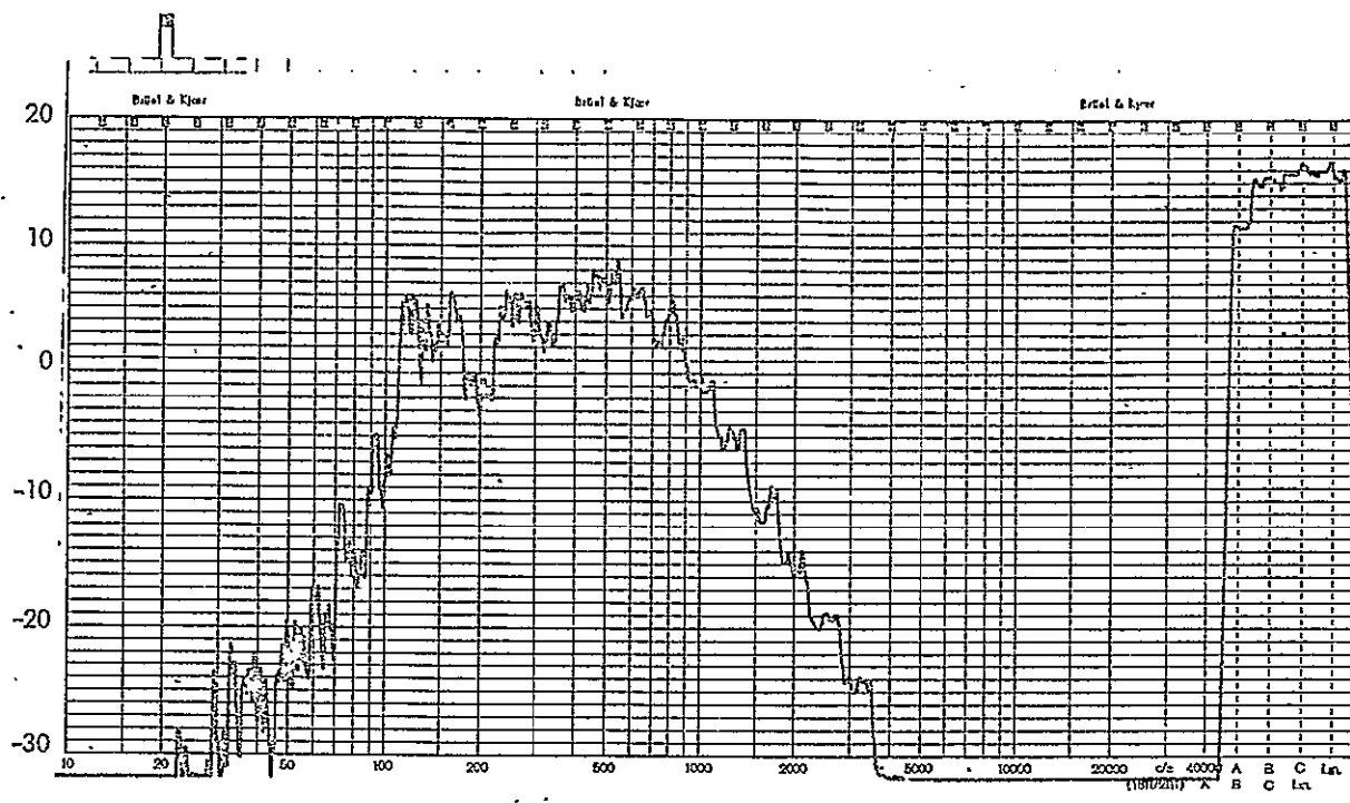
Figure B-42: Measured One-Third Octave Acceleration Response Levels, Experiment No. 5; Accelerometer A2
