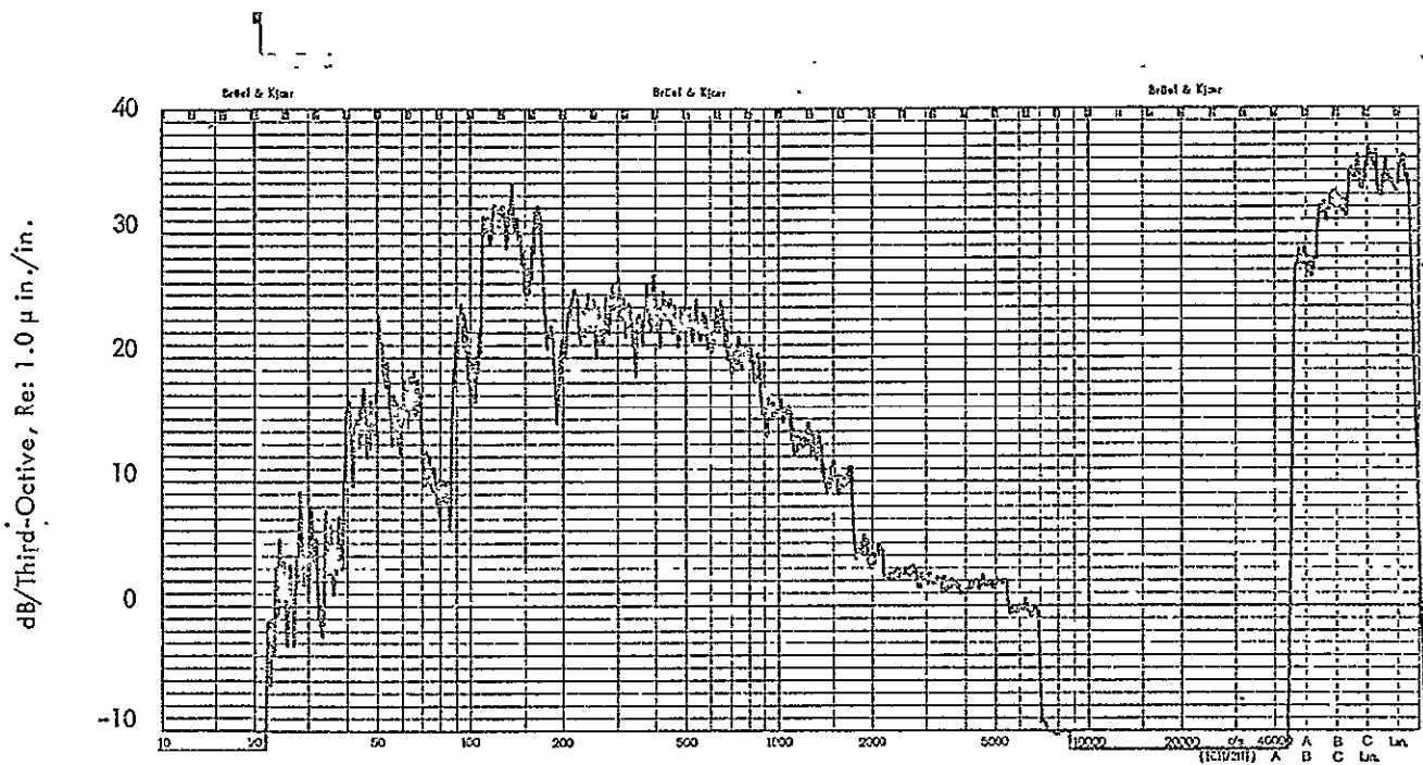
Figure B-10: Measured One-Third Octave Strain Levels, Experiment No. 1; Strain Gauge SG2
