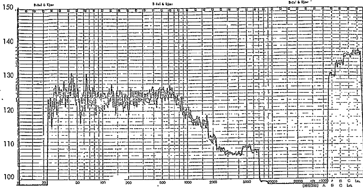
Figure B-1: Measured One-Third Octave Sound Pressure Levels, Experiment No. 1; External Microphone M1
