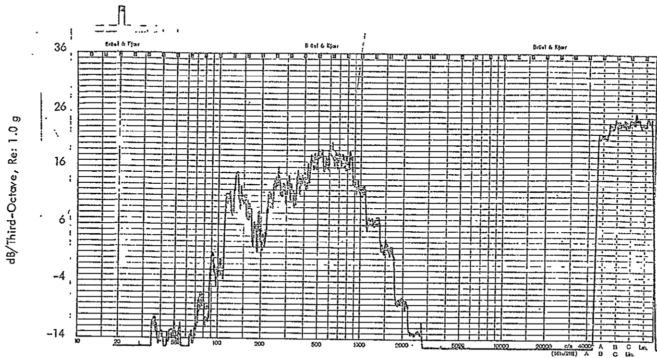
Figure B-5: Measured One-Third Octave Acceleration Response Levels, Experiment No. 1; Accelerometer A2
