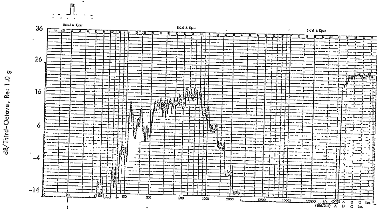
Figure B-14: Measured One-Third Octave Acceleration Response Levels, Experiment No. 2; Accelerometer A1
