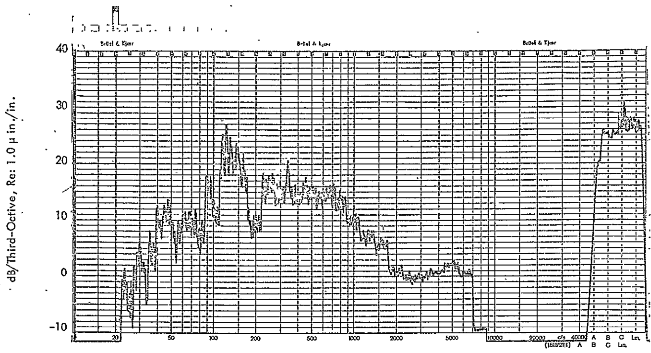
Figure B-9: Measured One-Third Octave Strain Levels, Experiment No. 1; Strain Gauge SG1
