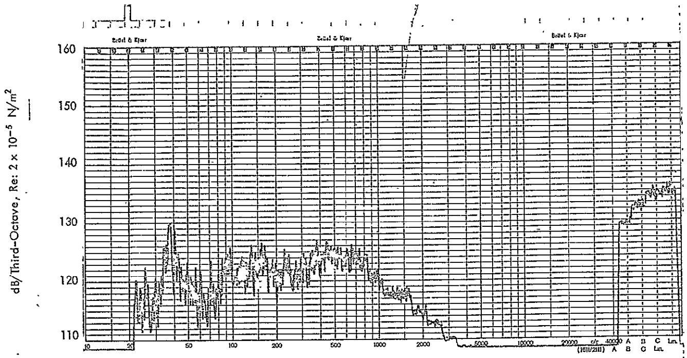
Figure B-23: Measured One-Third Octave Sound Pressure Levels, Experiment No. 3; External Microphone M3
