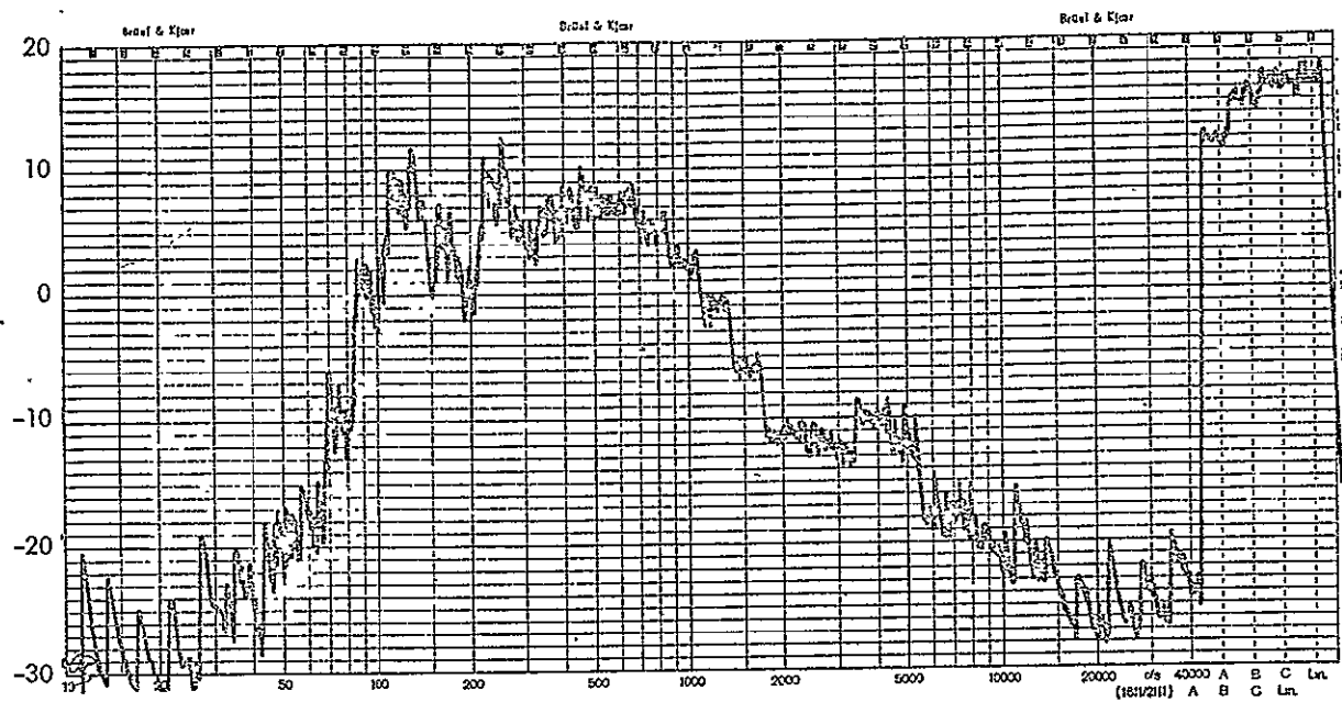
Figure B-47: Measured One-Third Octave Acceleration Response Levels, Experiment No. 6; Accelerometer A1
