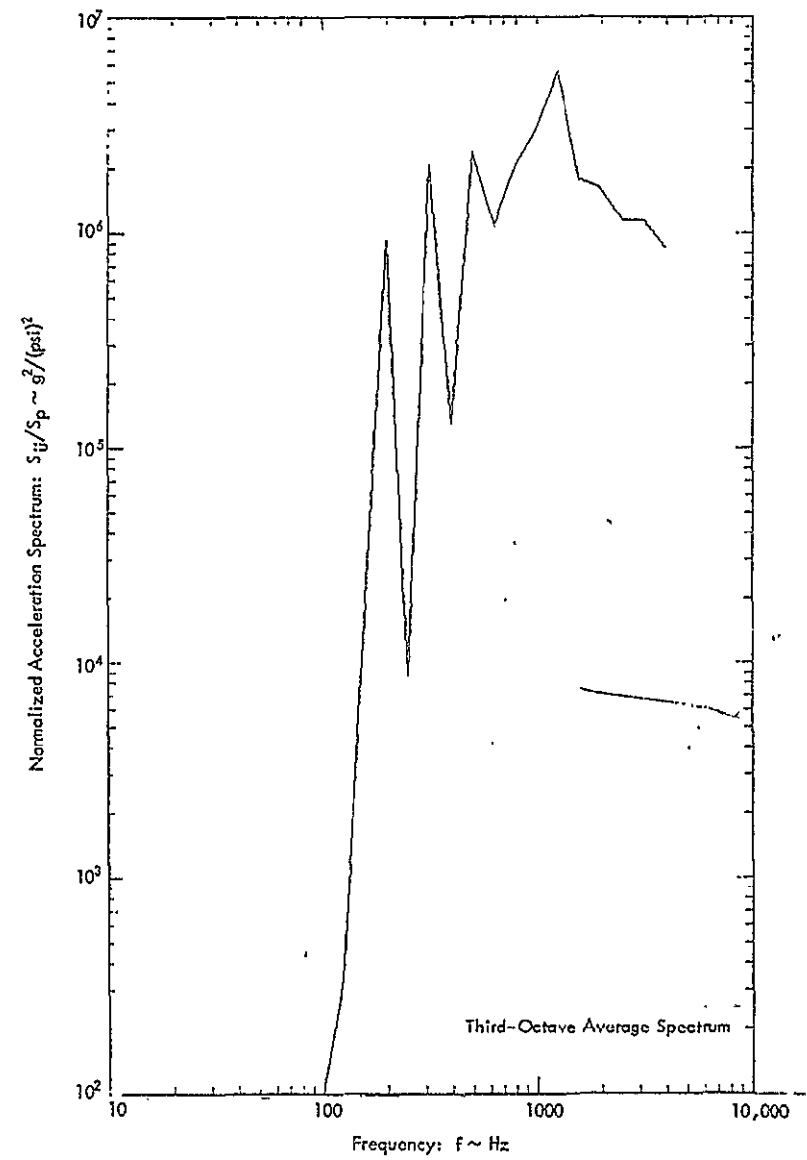
Figure A-8 : Predicted Normalized Acceleration Response of Cylinder for Configuration No. 2; Q = 200
