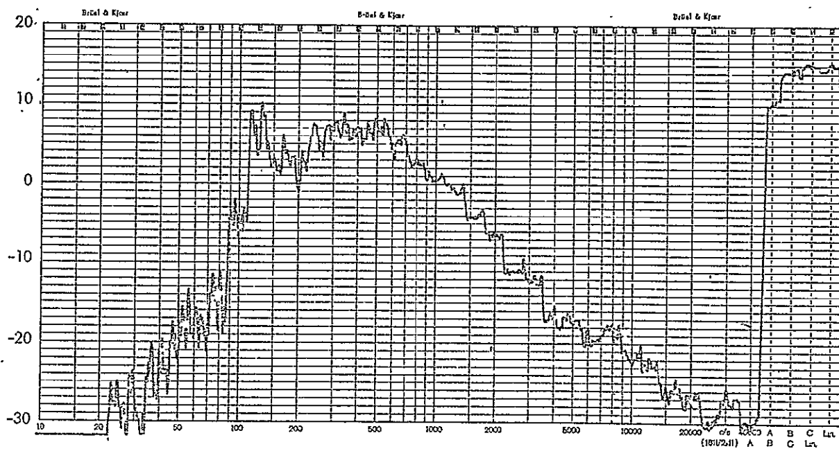
Figure B-43: Measured One-Third Octave Acceleration Response Levels, Experiment No. 5; Accelerometer A3
