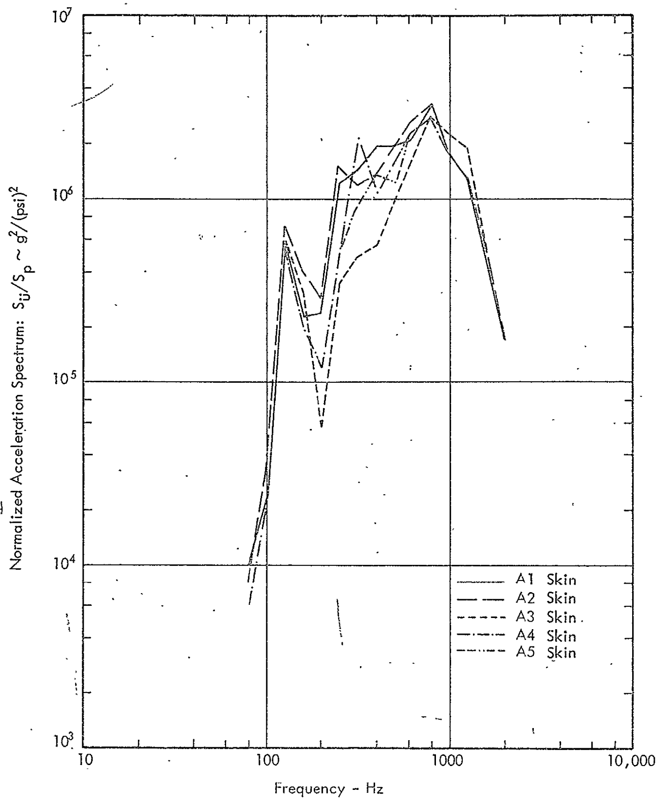
FIGURE 13. Acceleration Responses for Configuration No. 1, Measured During Experiment 1
