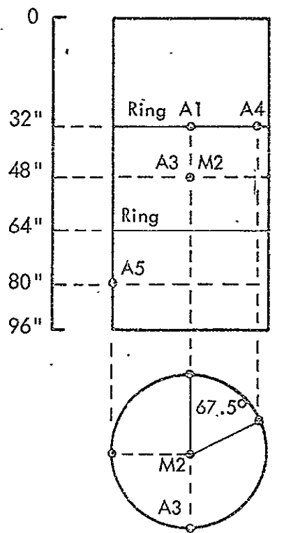
Shell with two rings Configuration No. 2
