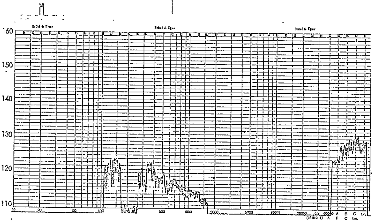
Figure B-12: Measured One-Third Octave Sound Pressure Levels, Experiment No. 2; Internal Microphone M2
