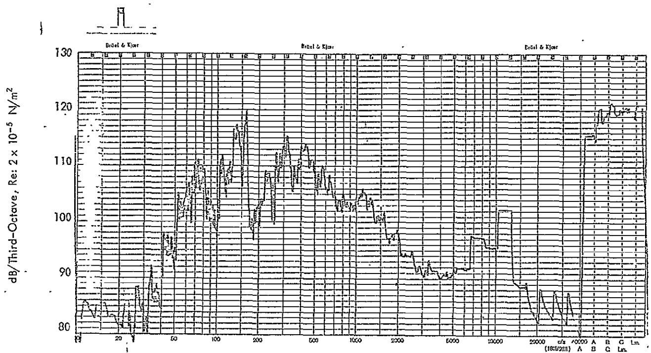
Figure B-32: Measured One-Third Octave Sound Pressure Levels, Experiment No. 4; Internal Microphone M2
