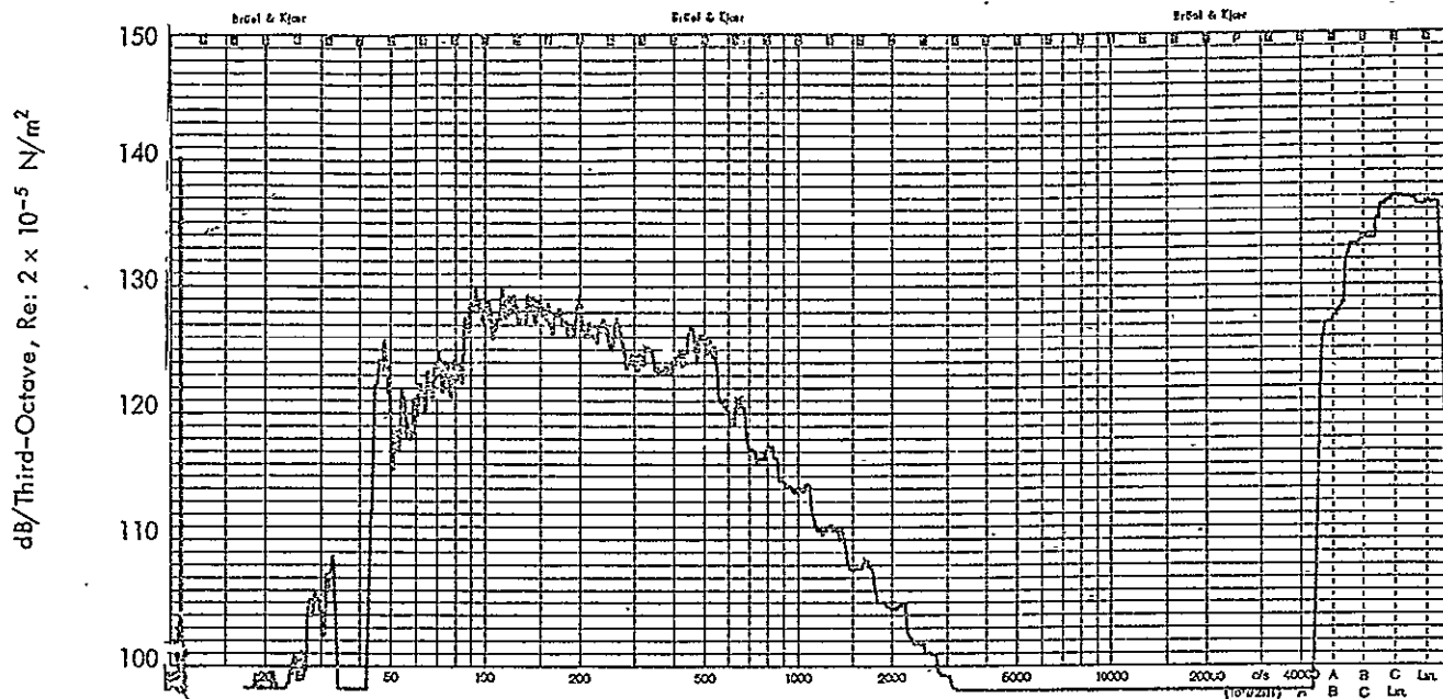
Figure B-51: Measured One-Third Octave Sound Pressure Levels, Experiment No. 7; External Microphone M1
