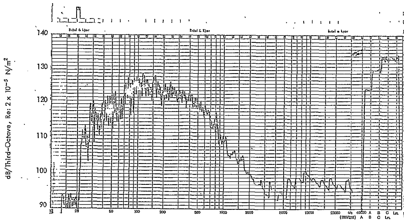
Figure B-31: Measured One-Third Octave Sound Pressure Levels, Experiment No. 4; External Microphone M1
