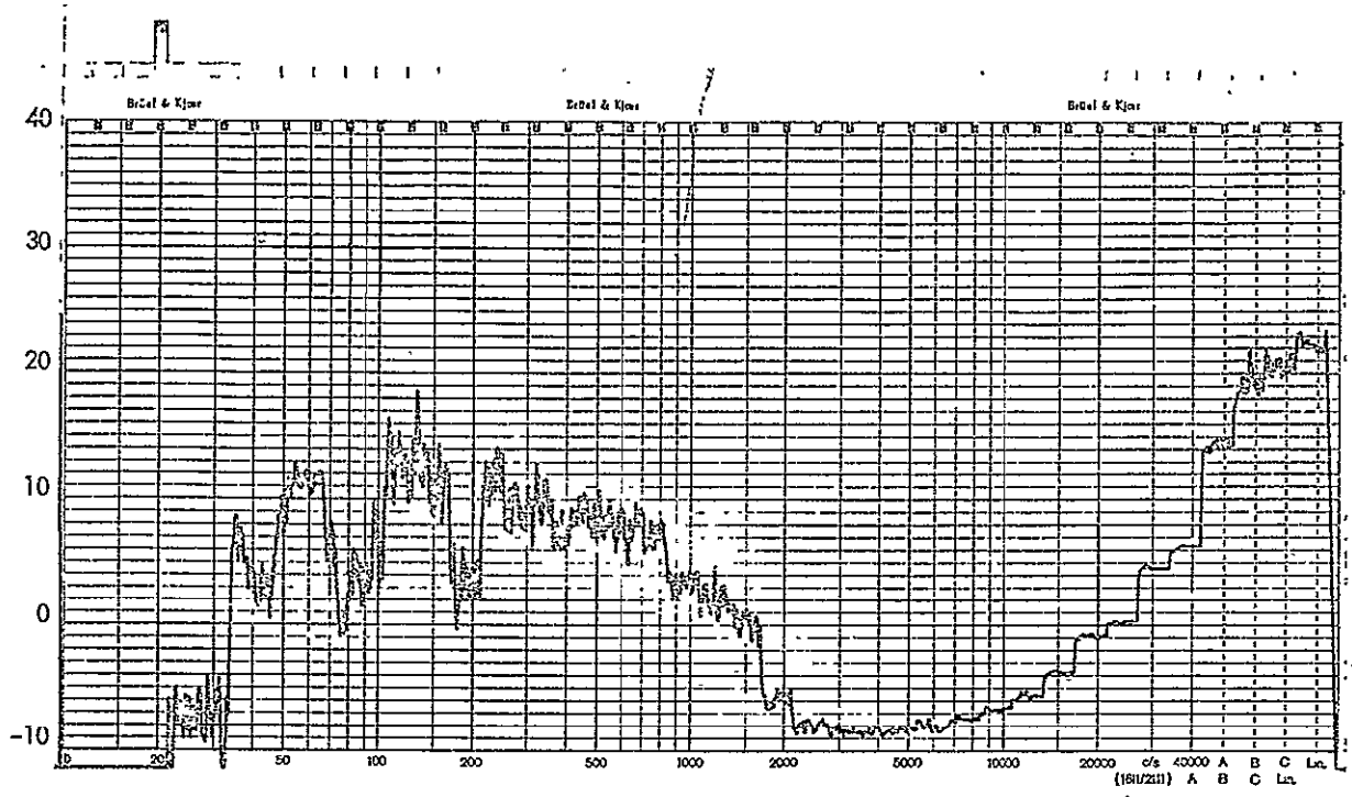
Figure B-29: Measured One-Third Octave Strain Levels, Experiment No. 3; Strain Gauge SG1
