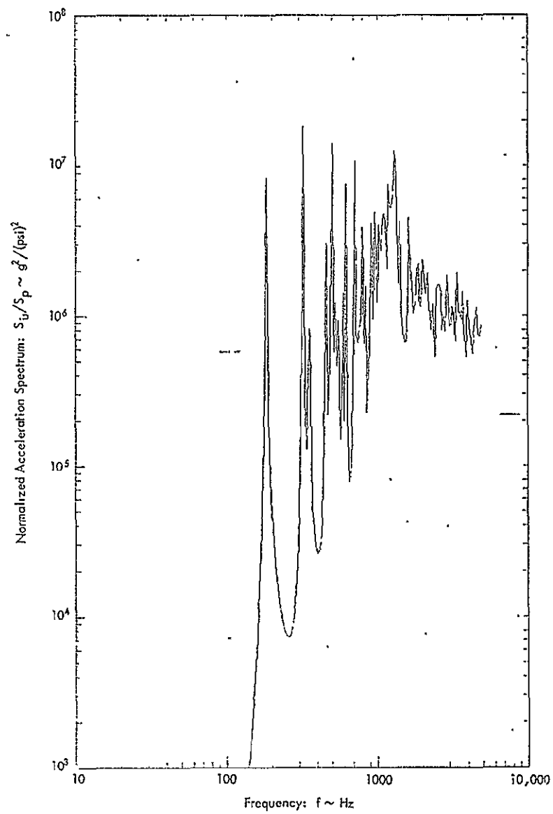
Figure A-8 : Predicted Normalized Acceleration Response of Cylinder for Configuration No. 2; Q = 200
