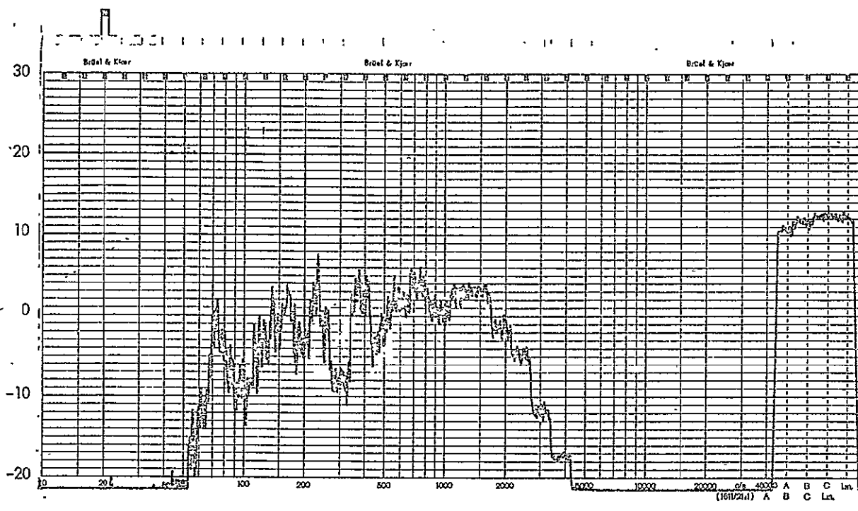
Figure B-15: Measured One-Third Octave Acceleration Response Levels, Experiment No. 2; Accelerometer A2
