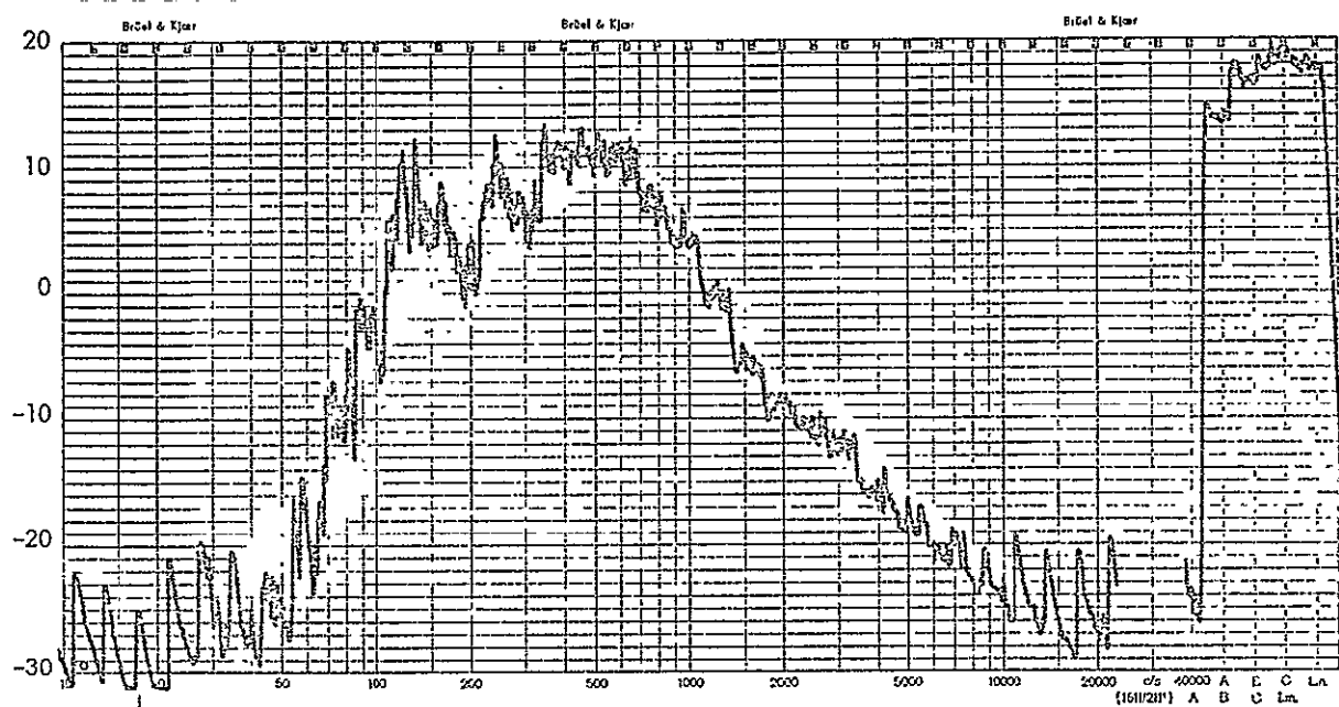
Figure B-48: Measured One-Third Octave Acceleration Response Levels, Experiment No. 6; Accelerometer A2
