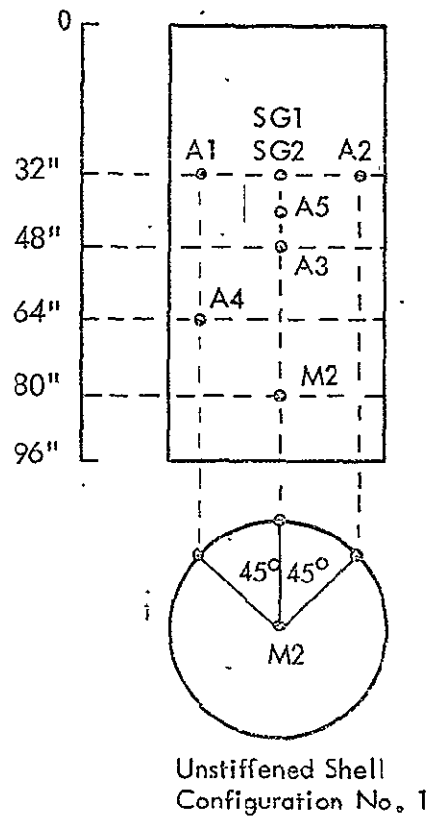
FIGURE 7. Test Configuration for Experiment No. 1
