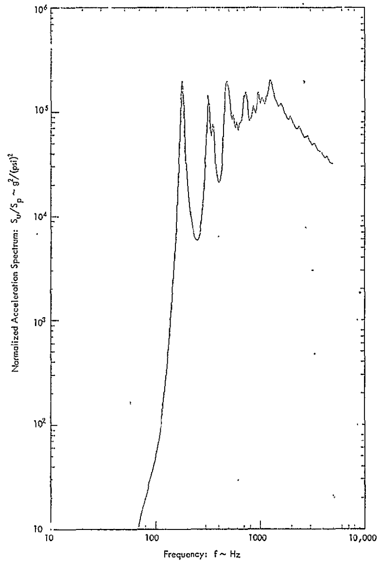
Figure A-13: Predicted Normalized Acceleration Response of Cylinder for Configuration No. 4; Q \approx 15
