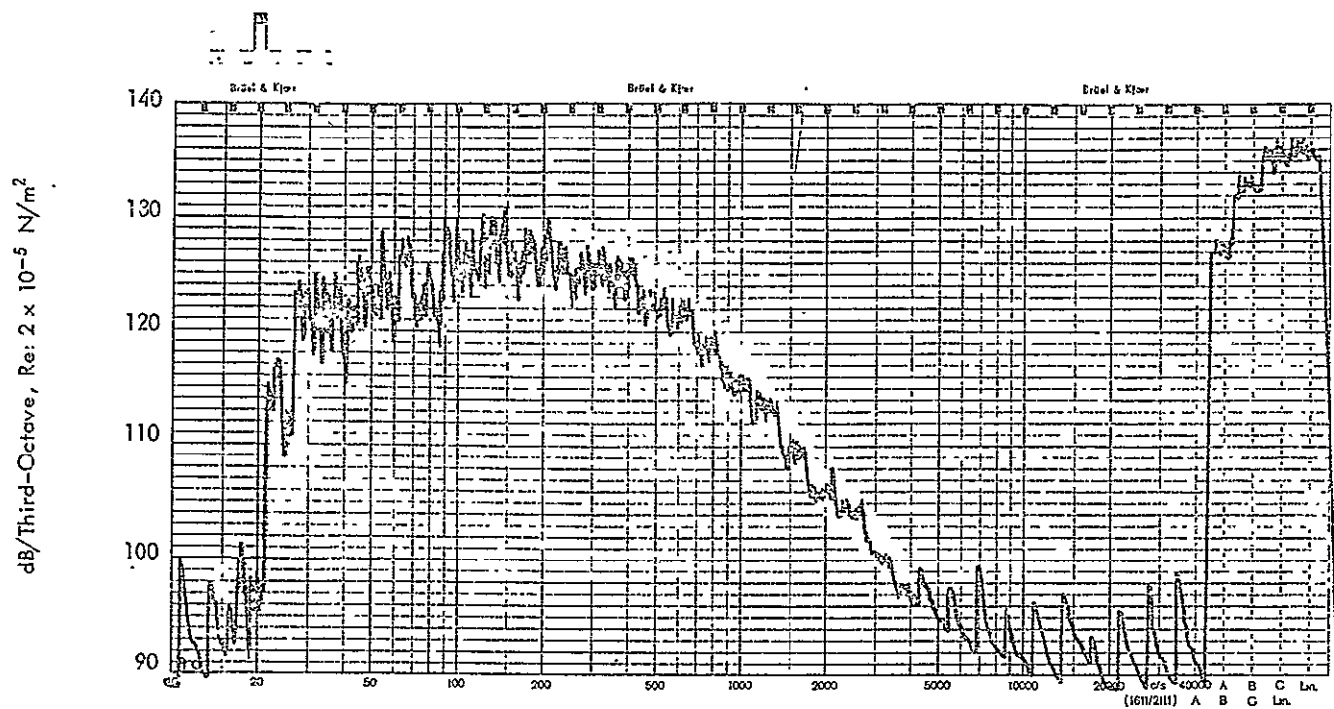
Figure B-45: Measured One-Third Octave Sound Pressure Levels, Experiment No. 6; External Microphone M1
