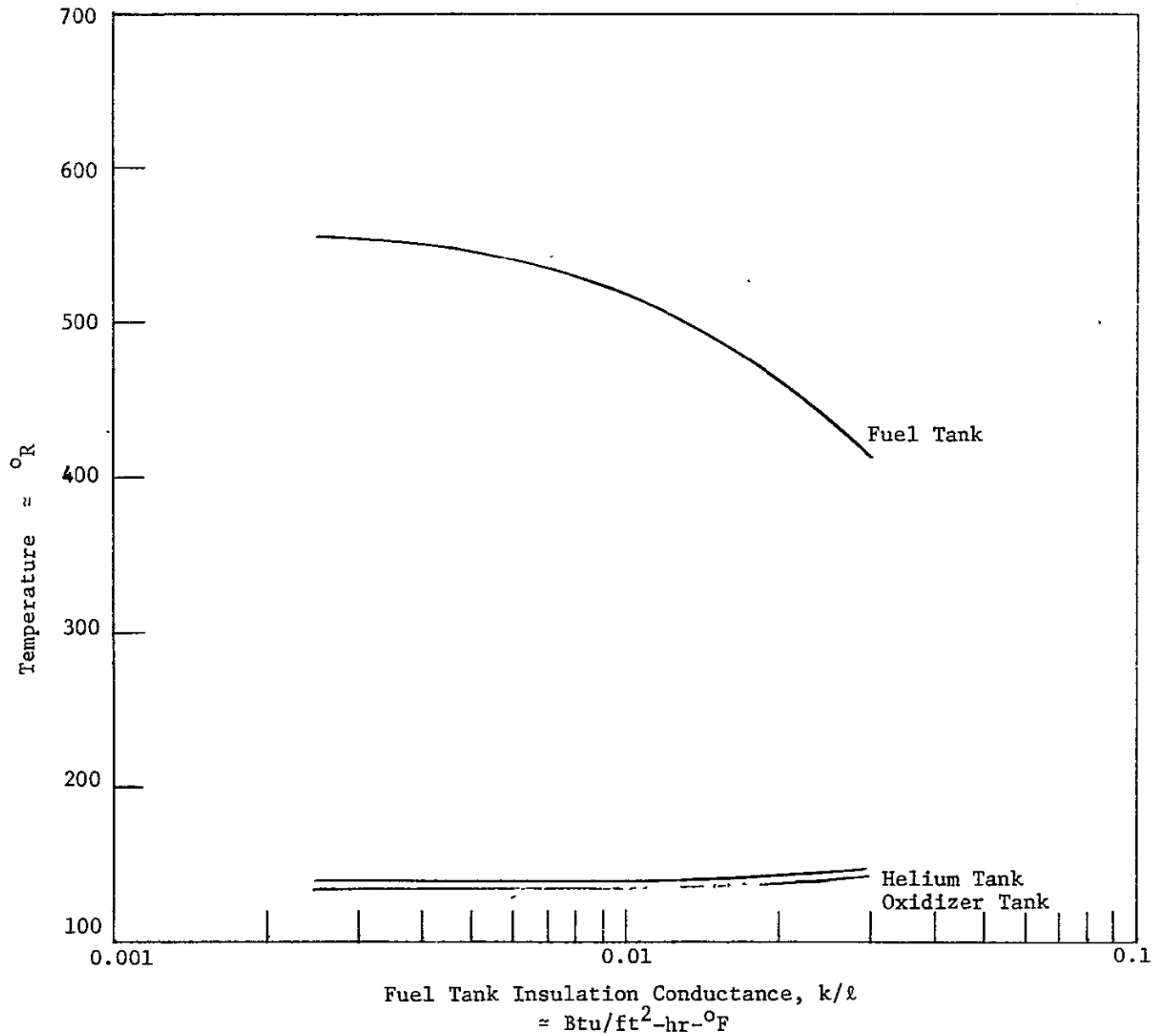
Figure 4-6. Effect of Fuel Tank Insulation Conductivity; RTG = 960^\circ\text{R}
