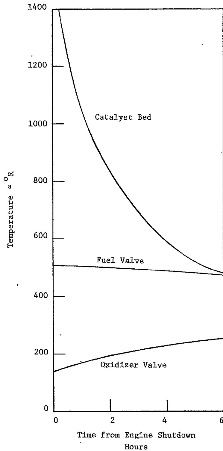
Figure 4-21. Thermal Transient After Engine Operation Non-Operative Engine
