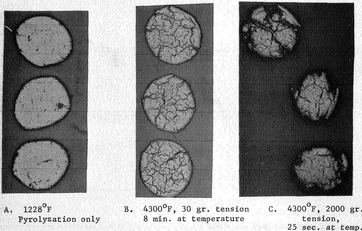
FIGURE 16. PYROLYZED R-1-50/EPOXY NOVOLAC-FURFURYL ALCOHOL, Heated to 4300°F, 100X.
