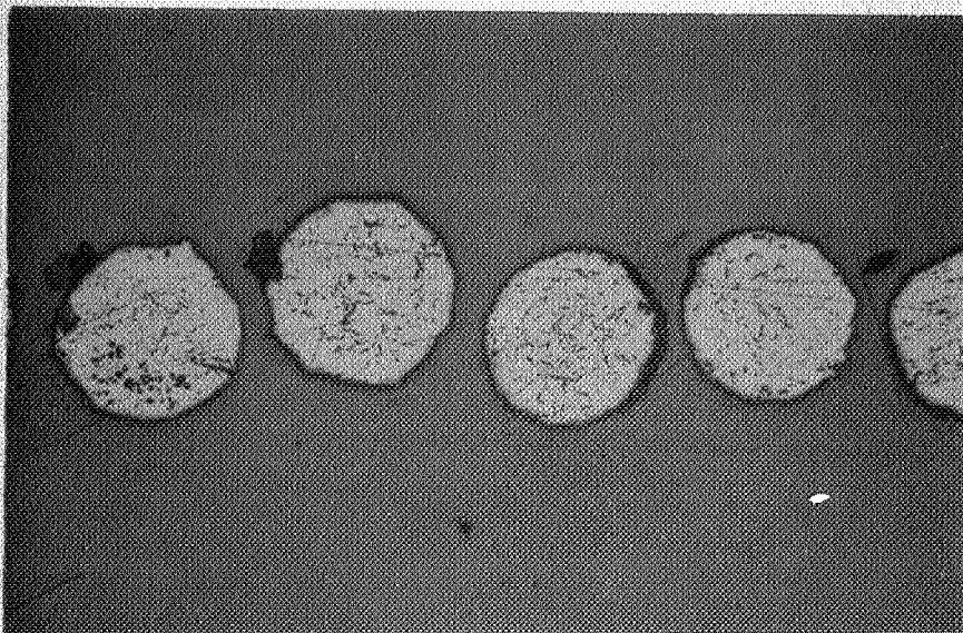
FIGURE 14. PYROLYZED R-1-50/EPOXY NOVOLAC-FURFURYL ALCOHOL, Die formed, 100X.
