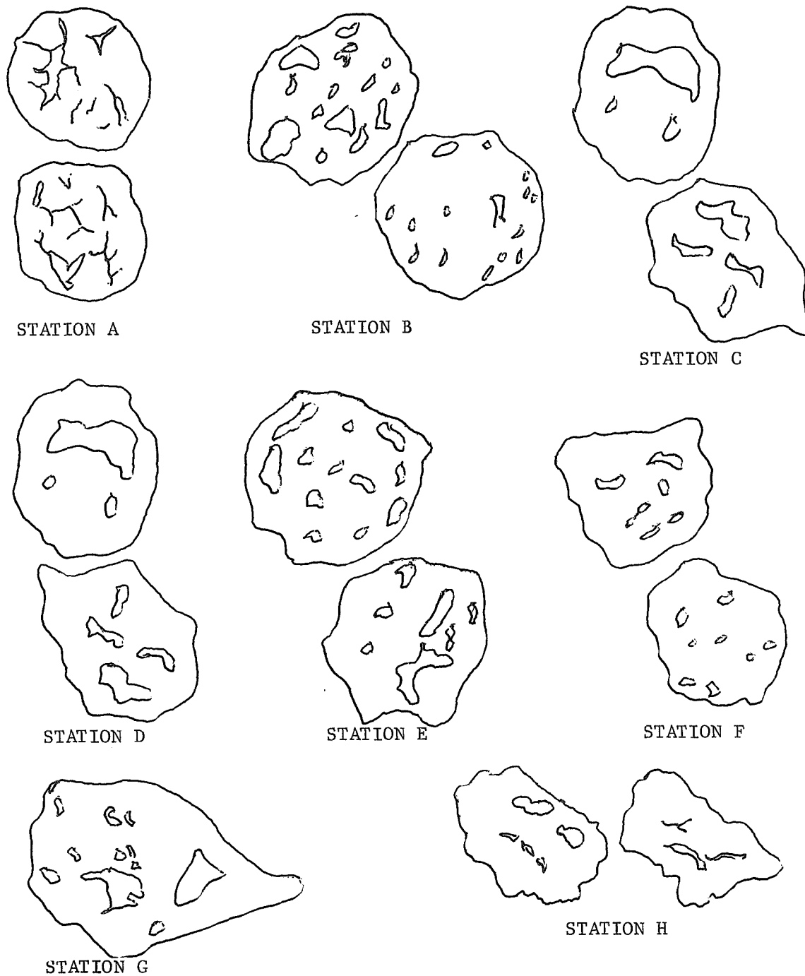
FIGURE 12. FILAMENTS FORMED ON GRAPHITE PULLEYS, 100X
