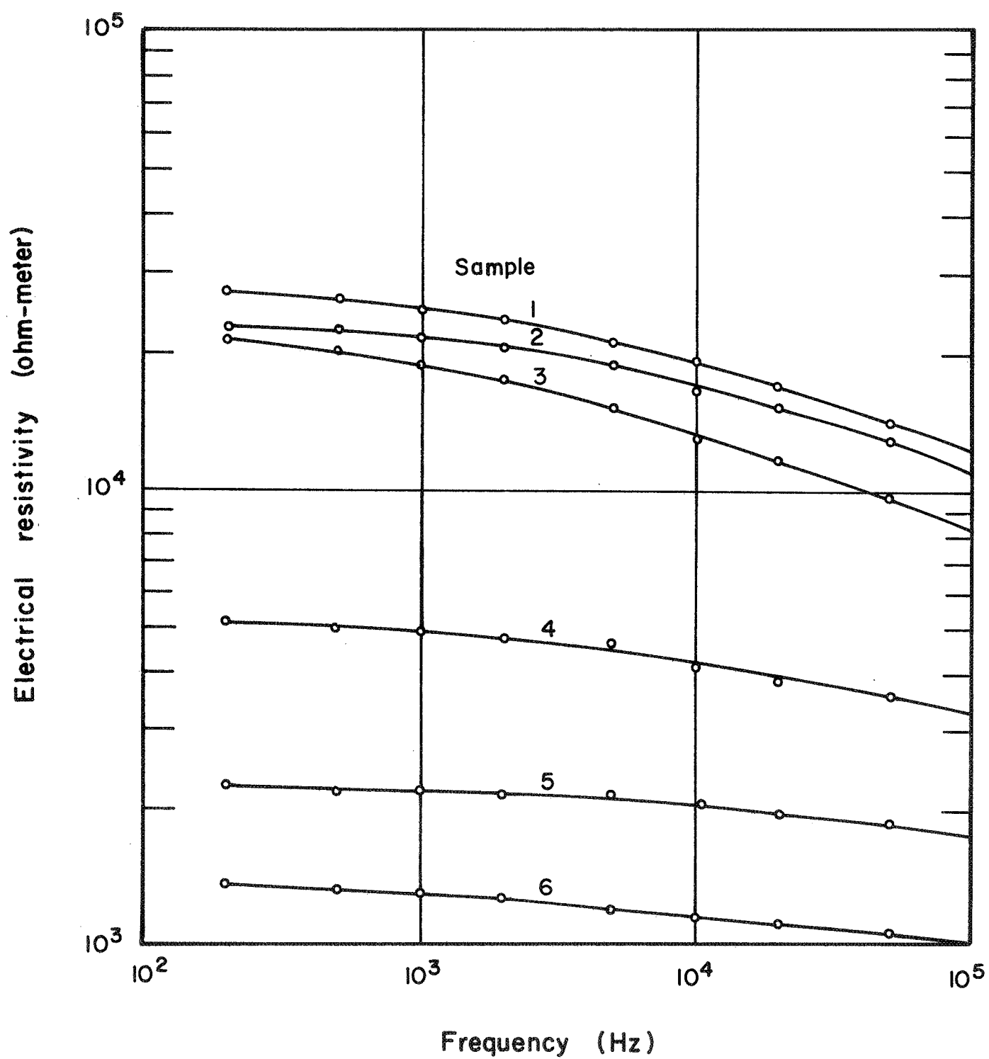
Fig. 16. Electrical resistivity as a function of frequency at -30^{\circ}\text{C} .
