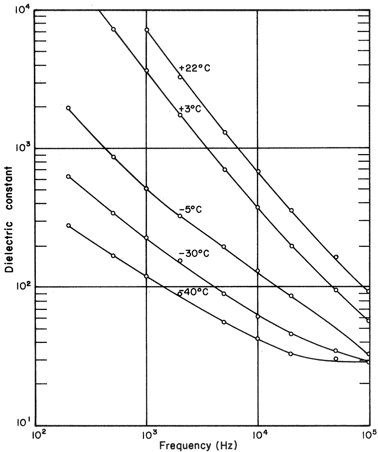
Fig. 19. Dielectric constant of sample 3 as a function of temperature and frequency.
