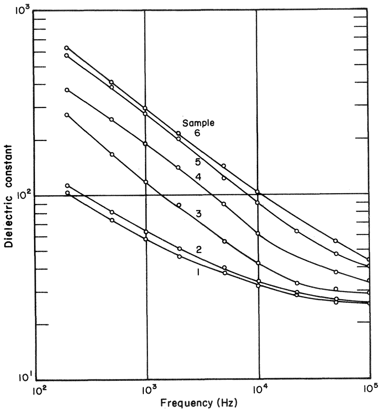
Fig. 17. Dielectric constant as a function of frequency at -40^\circ\text{C} .
