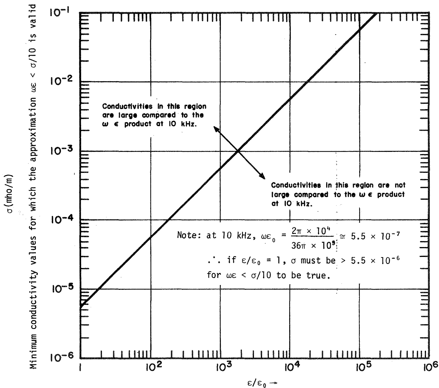
Fig. 20. Minimum values of conductivity as a function of \epsilon/\epsilon_0 for \omega\epsilon < \sigma/10 at 10 kHz.
