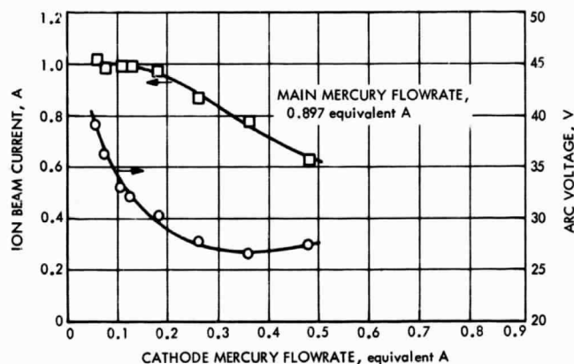
Fig. 13. Effect of cathode mercury flow on thruster performance, high main propellant flow
