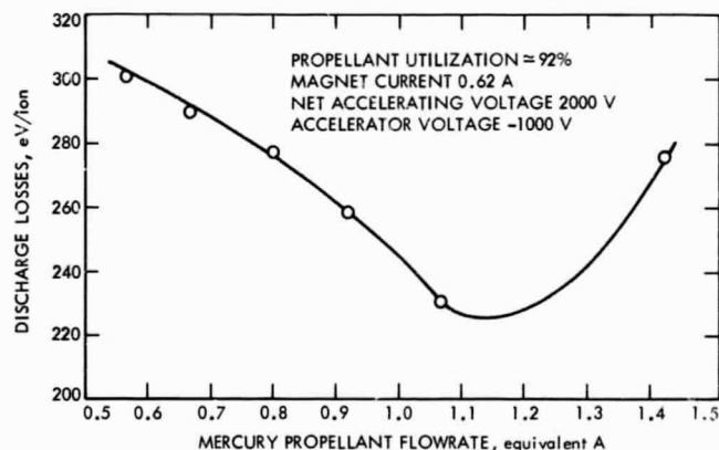
Fig. 7. Effect of propellant flowrate on the discharge loss at constant propellant utilization
