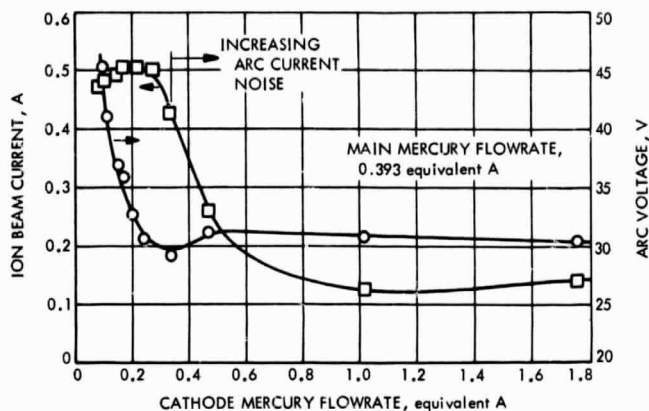
Fig. 12. Effect of cathode mercury flow on thruster performance, low main propellant flow
