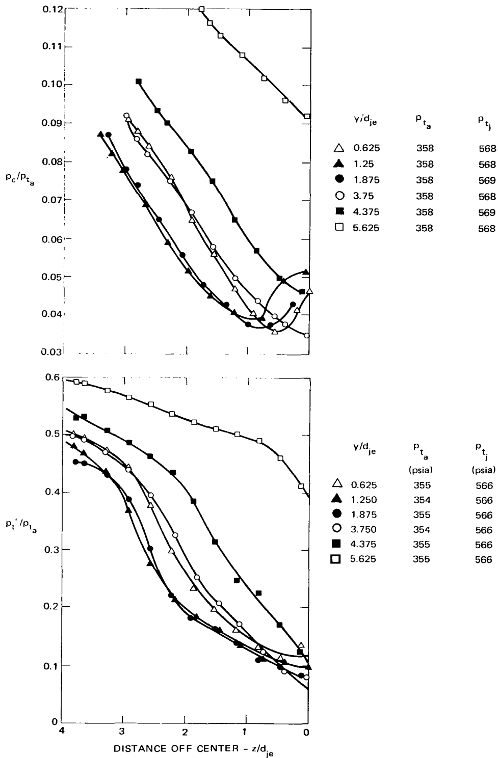
FIG. 8 MEASURED CONE SURFACE PRESSURE DATA AND PITOT PRESSURE DATA FOR FIVE-PORT INJECTOR ALIGNED WITH FLOW AT x/d_{je} = 5
