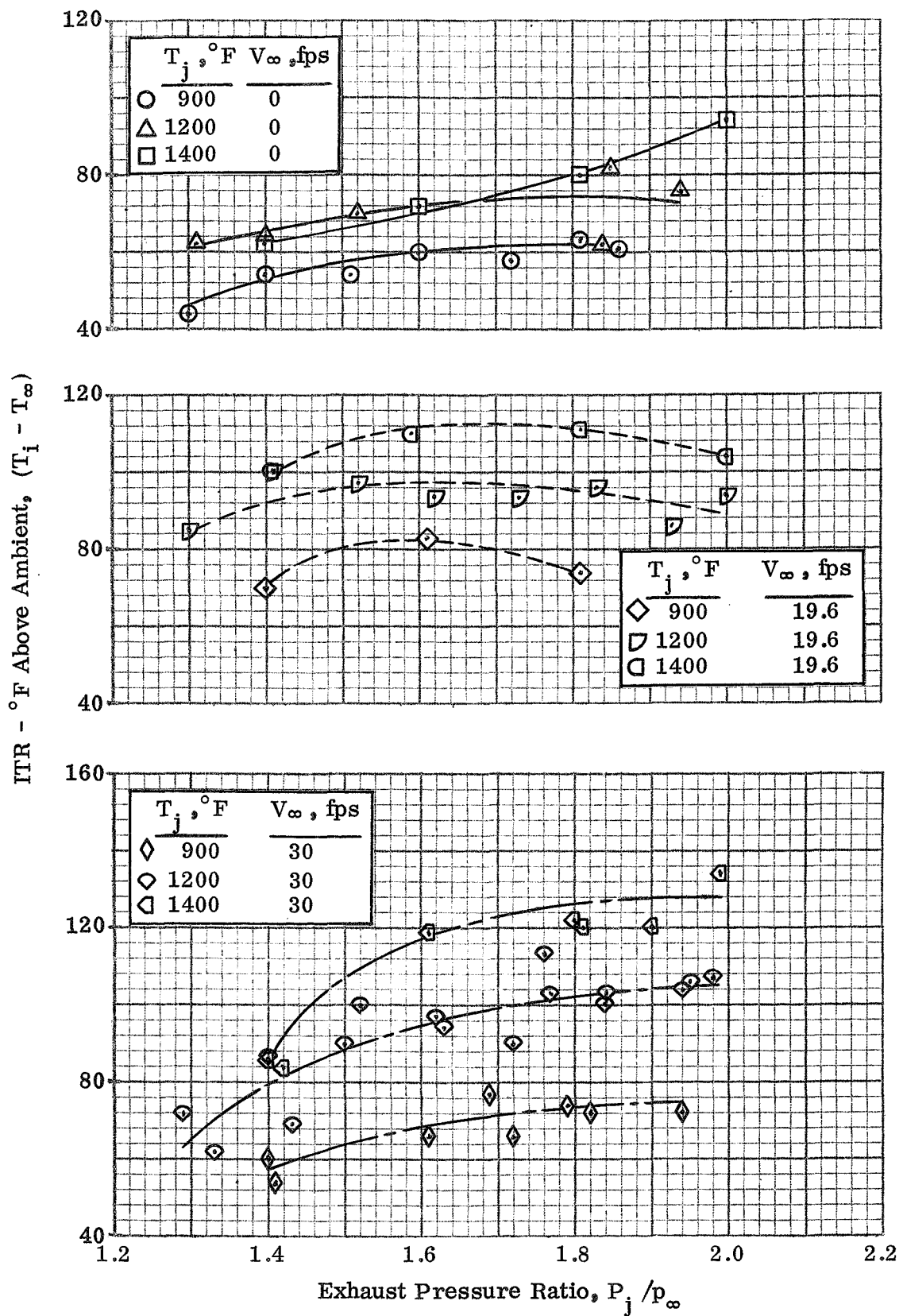
Figure 1. - Variation of ITR With Exhaust Pressure Ratio and Exhaust Temperature at Various Wind Velocities. Side Inlets Configuration, \psi = 0^\circ .
