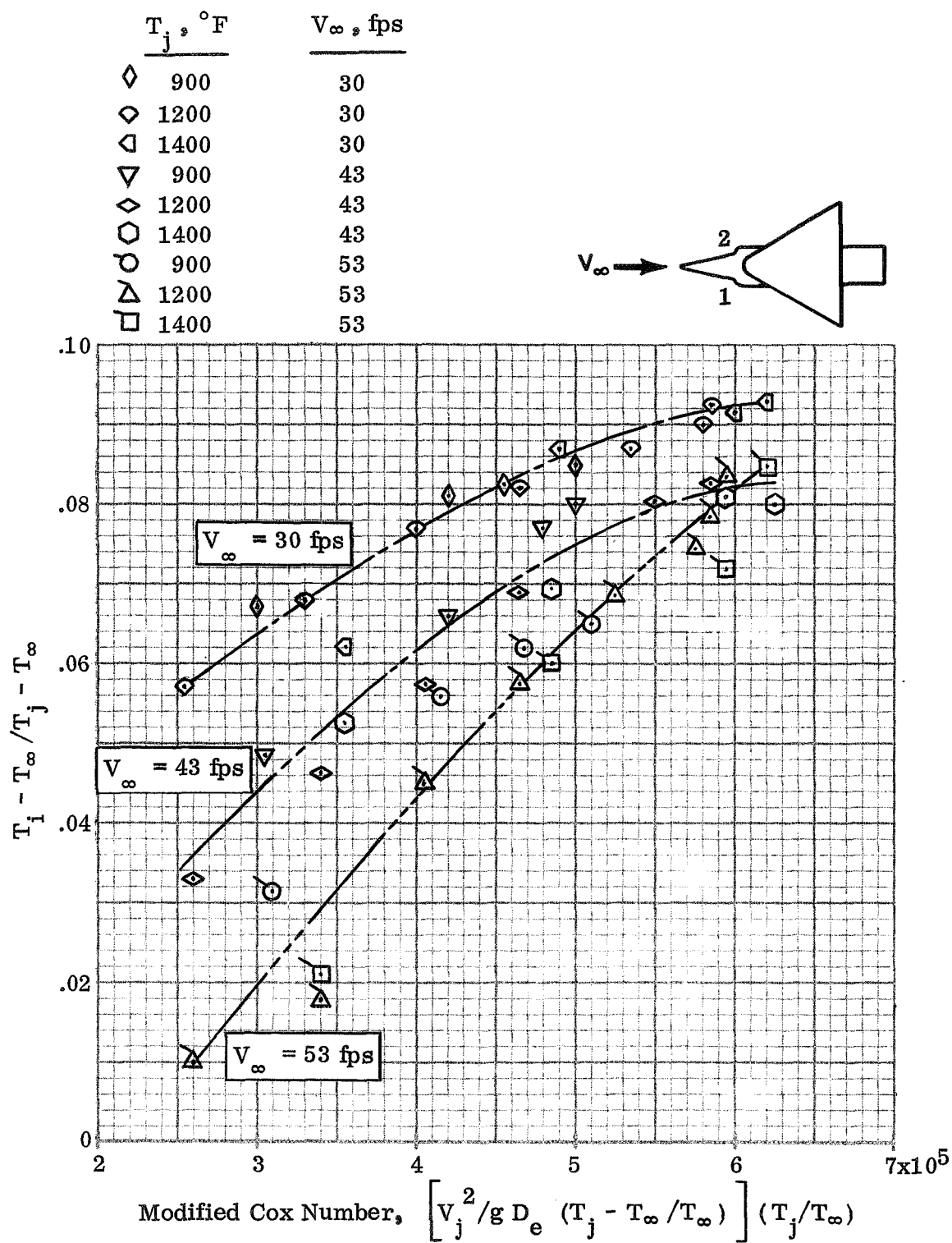
Figure 9. - Correlation of Normalized ITR With Modified Cox Number. Side Inlets Configuration, \psi = 0^\circ .
