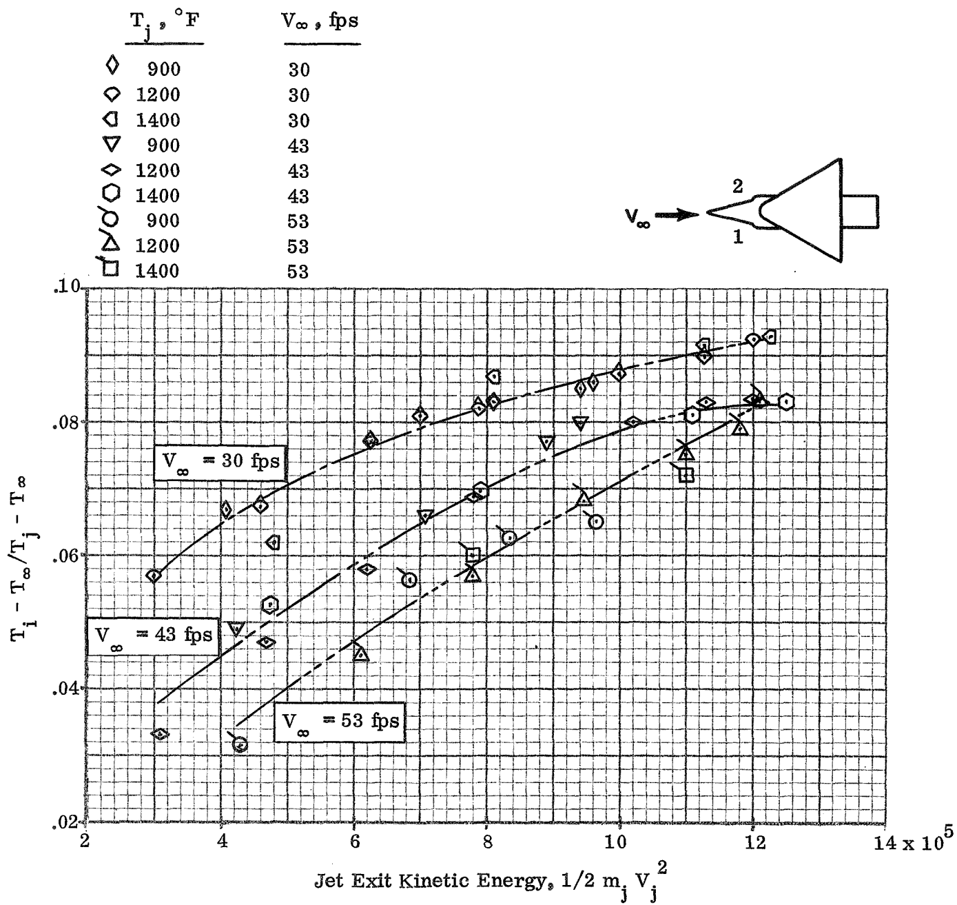
Figure 8. - Correlation of Normalized ITR With Jet Exit Kinetic Energy. Side Inlets Configuration, \psi = 0^\circ .
