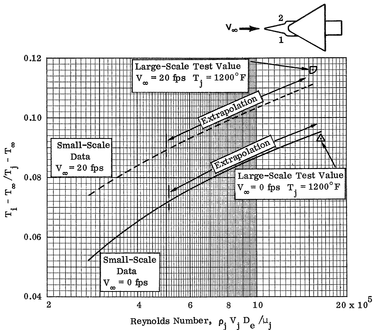
Figure 13. - Comparison of Small and Large-Scale ITR Based On Equal Reynolds Number. Side Inlets Configuration, \psi = 0^\circ .
