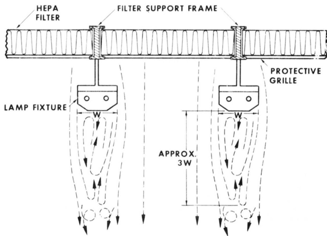
Figure 13. Turbulence from suspended lamp fixtures
