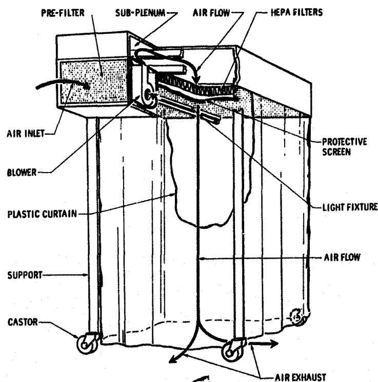
Figure 15. Vertical flow curtain room (portable)
