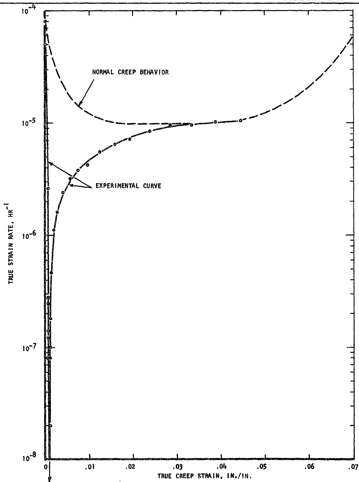
Figure 9. True strain rate as a function of true strain for T-111 alloy annealed 1 hour at 3000°F (1649°C) and creep tested at 1600°F (871°C) and 35 ksi (241 MN/M 2 ) in a vacuum of <1 \times 10^{-8} torr (Test S-60).
