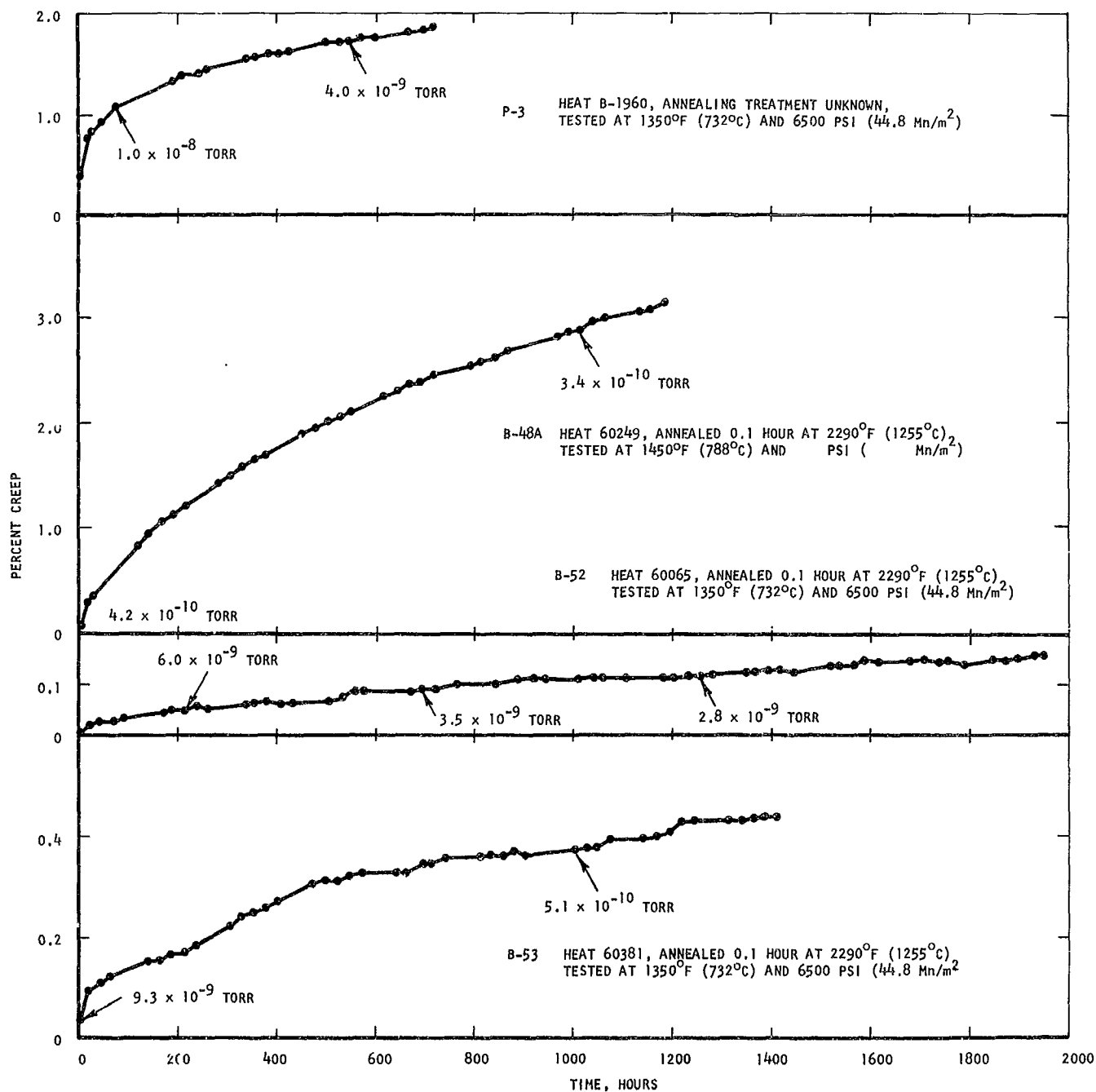
FIGURE III-4. CREEP TEST DATA, PURE Ta, TEST NOS. P-3, B-48A, B-52, and B-53, TESTED IN A VACUUM ENVIRONMENT OF <1 \times 10^{-8} TORR. ARROWS ON THE CURVES INDICATE CHAMBER PRESSURE AT VARIOUS INTERVALS DURING THE TEST.
