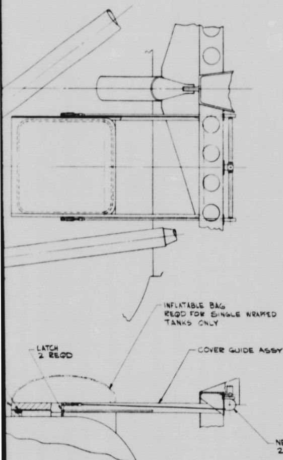
DETAIL - LOUVER COVER ASSY 2 REQD FOR DUAL WRAPPED TANKS 4 REQD FOR SINGLE WRAPPED TANKS
