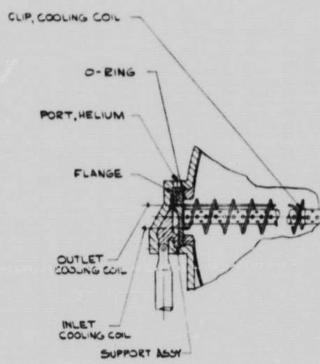
DETAIL - TOP FLANGE ASSY TYP TWO TANKS SHT 1
