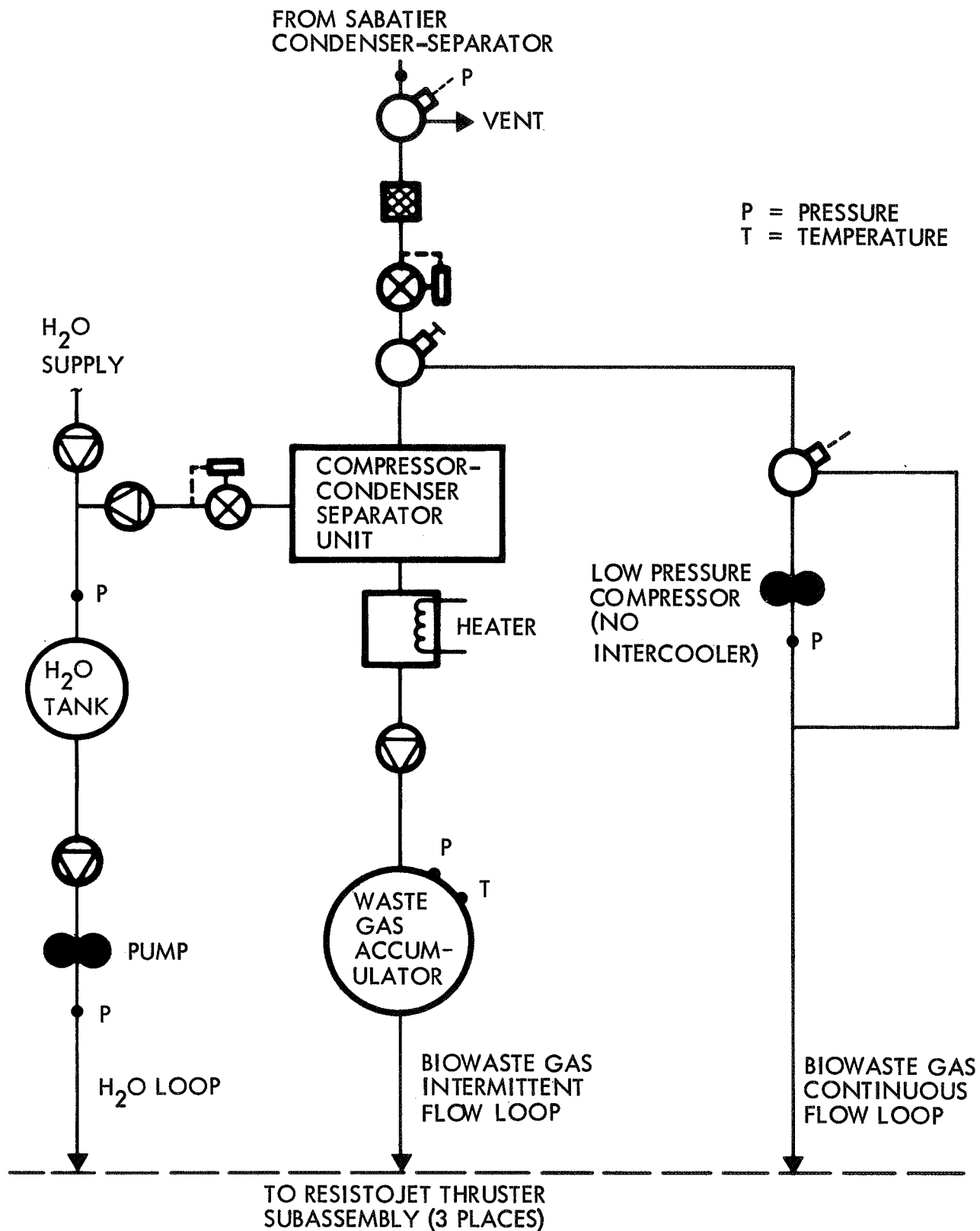
Figure 3-57. Resistojet Propellant Storage Subassembly
