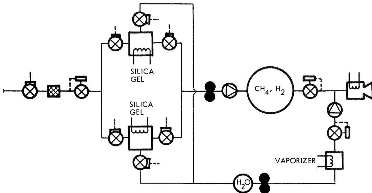
Figure 3-51. Resistojet Assembly Option 1
