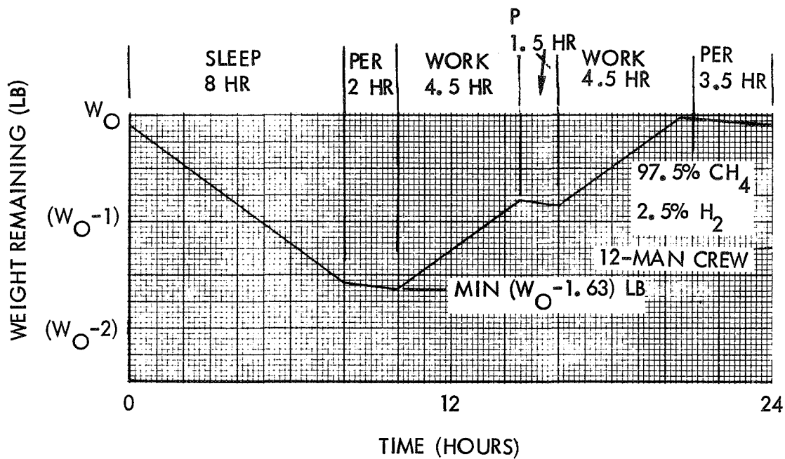
Figure 3-43. Biowaste Propellant Remaining With Average Usage
