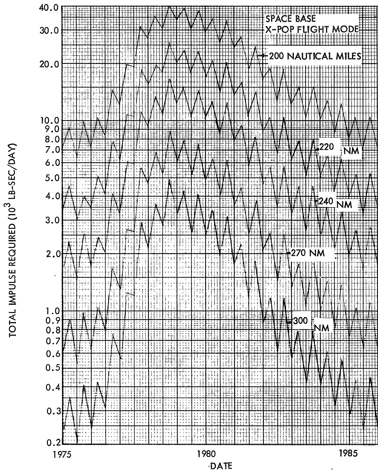
Figure 4-9. Orbit Maintenance Impulse, 2\sigma Atmosphere
