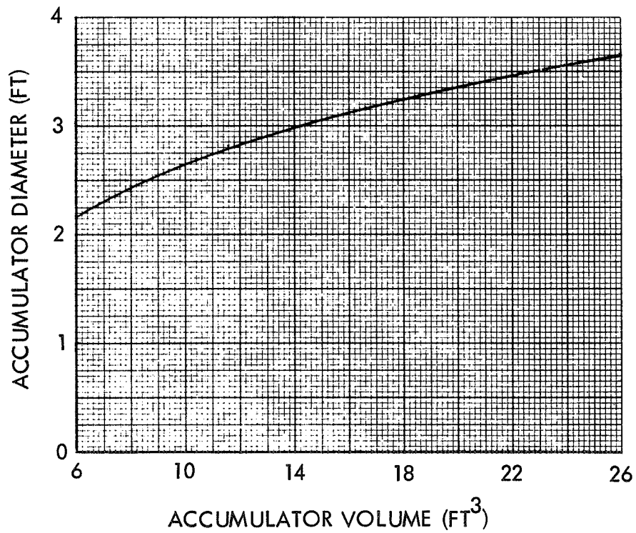
Figure 3-48. Accumulator Diameters
