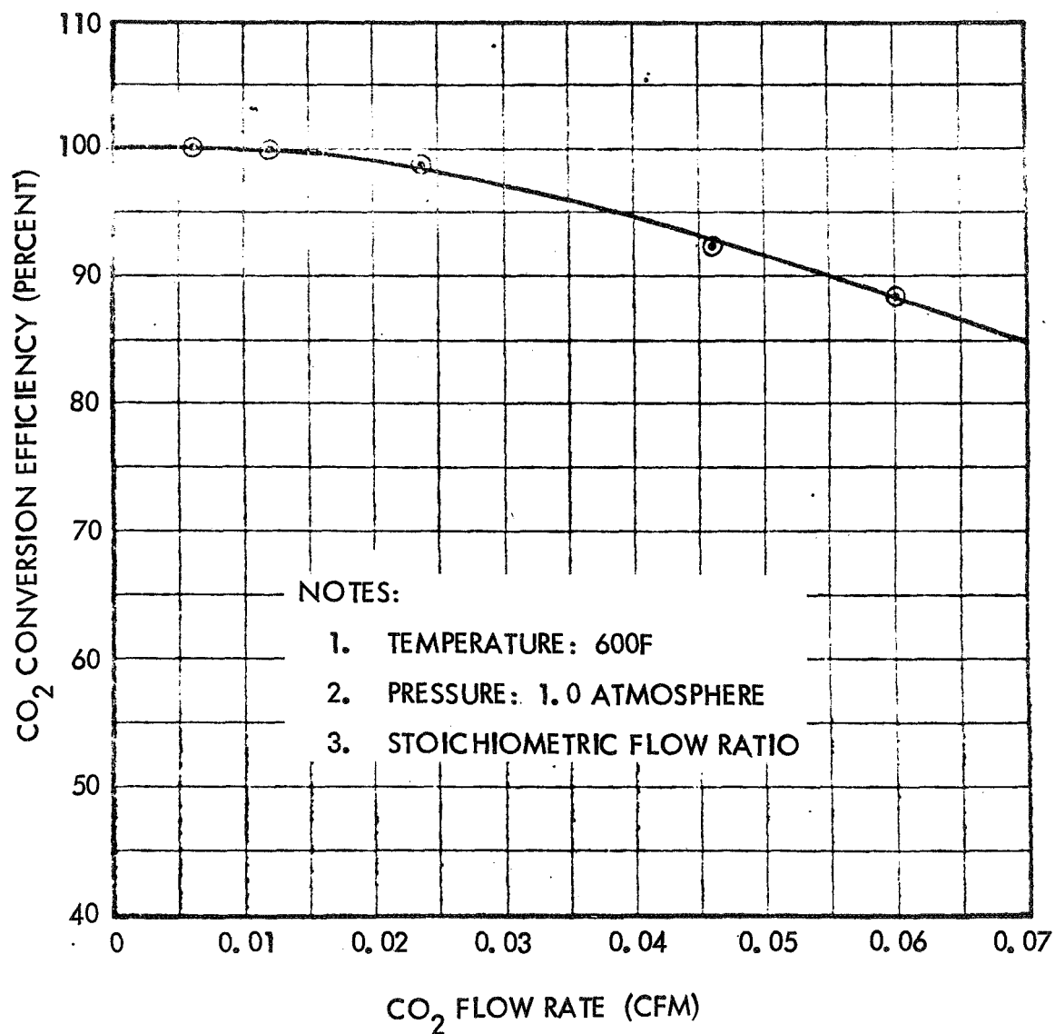
Figure A-4. Nickel on Kieselguhr Performance - Conversion Efficiency Versus Flow Rate
