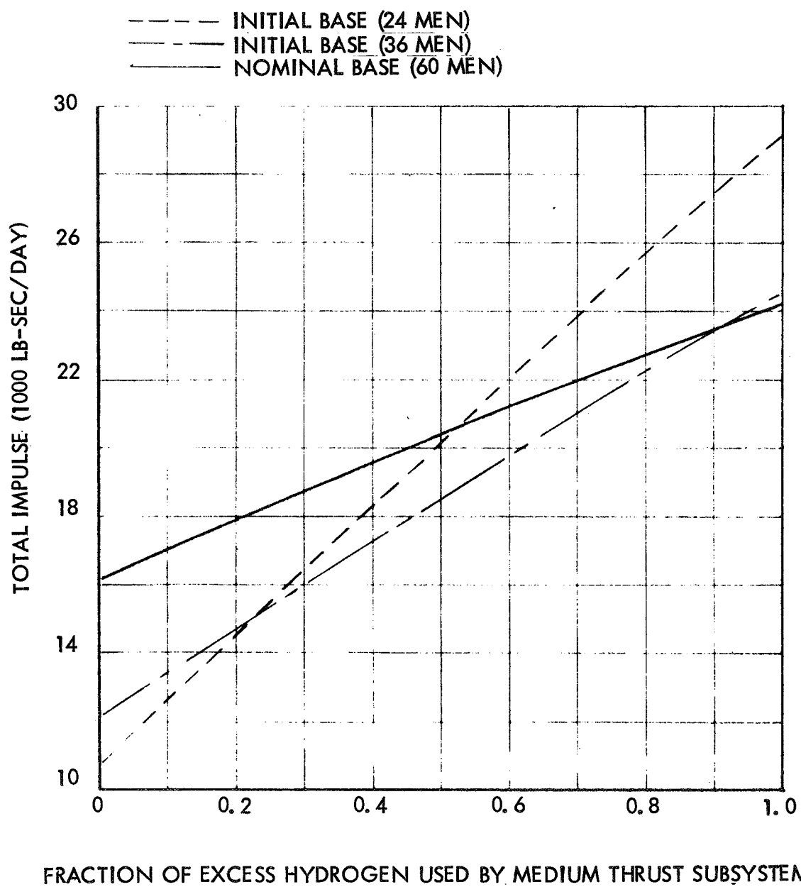
Figure 4-18. Initial and Nominal Space Base Impulse Capability
