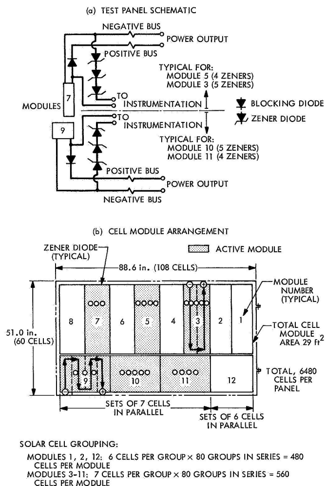
Fig. 7. Electrical design
