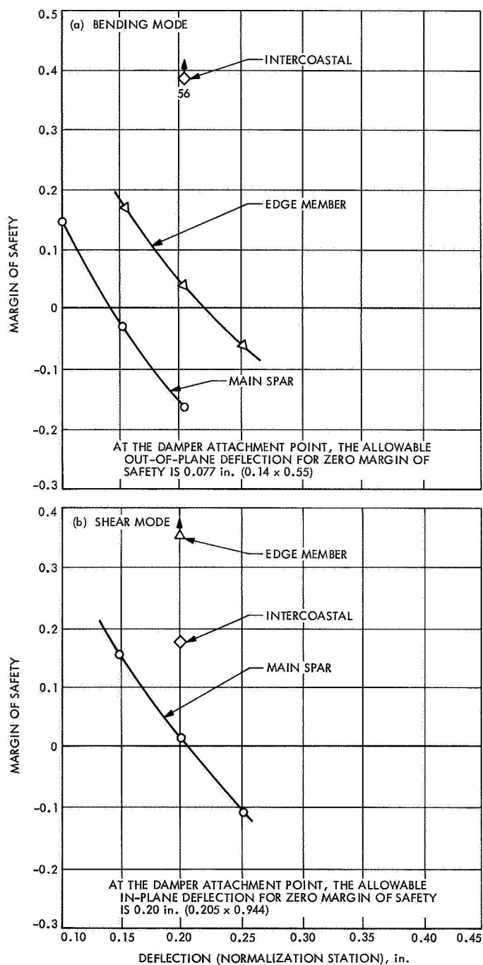
Fig. 10. Dynamic margins of safety vs deflection
