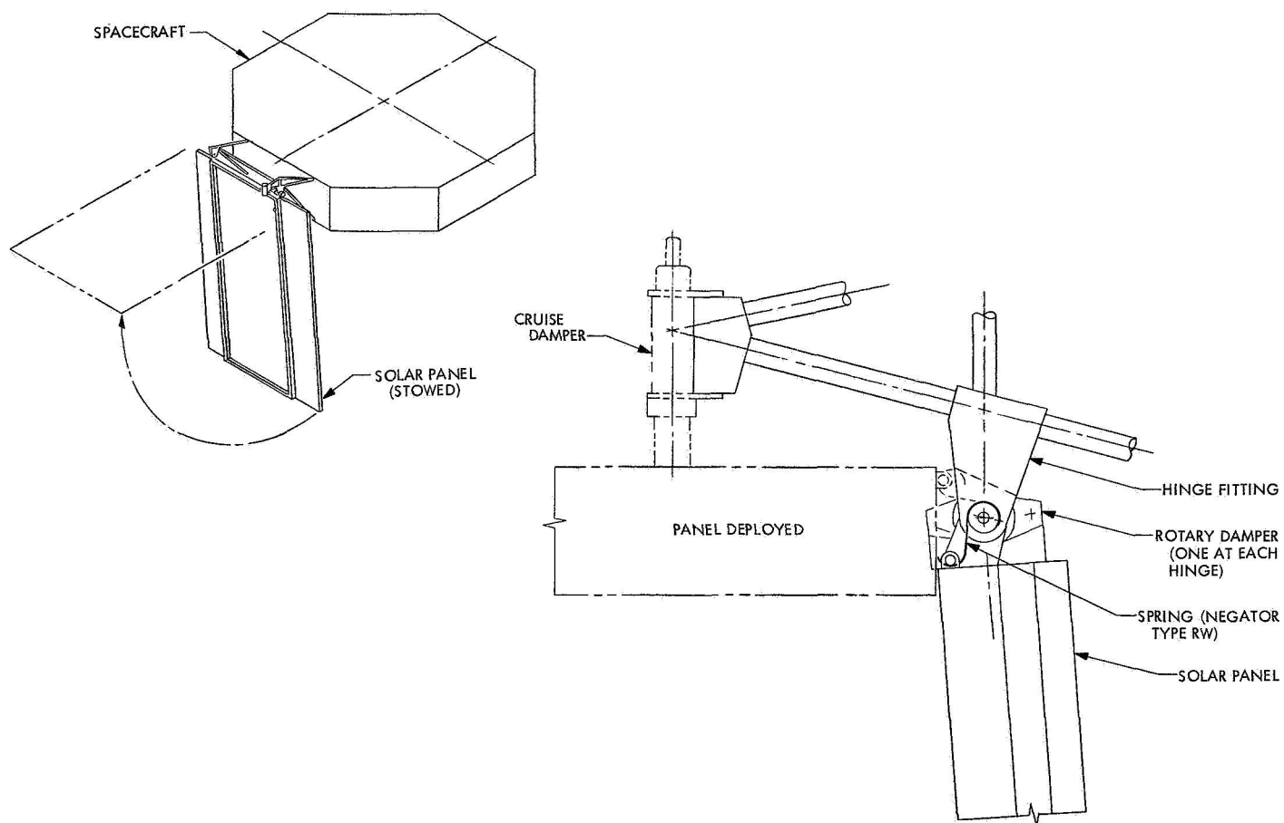
Fig. 5. Deployment equipment
