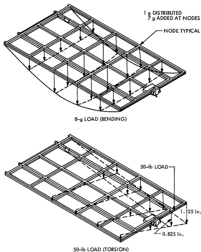
Fig. 11. Static deflection shapes
