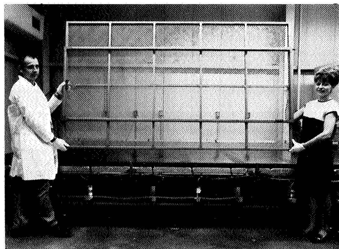
Fig. 24. Completed structural frame assembly
