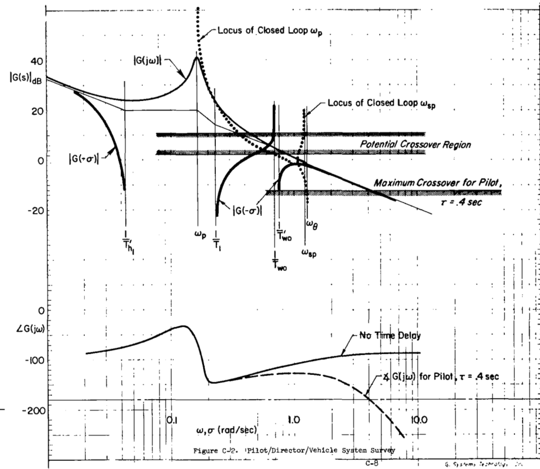
Figure C-2. Pilot/Director/Vehicle System Survey
