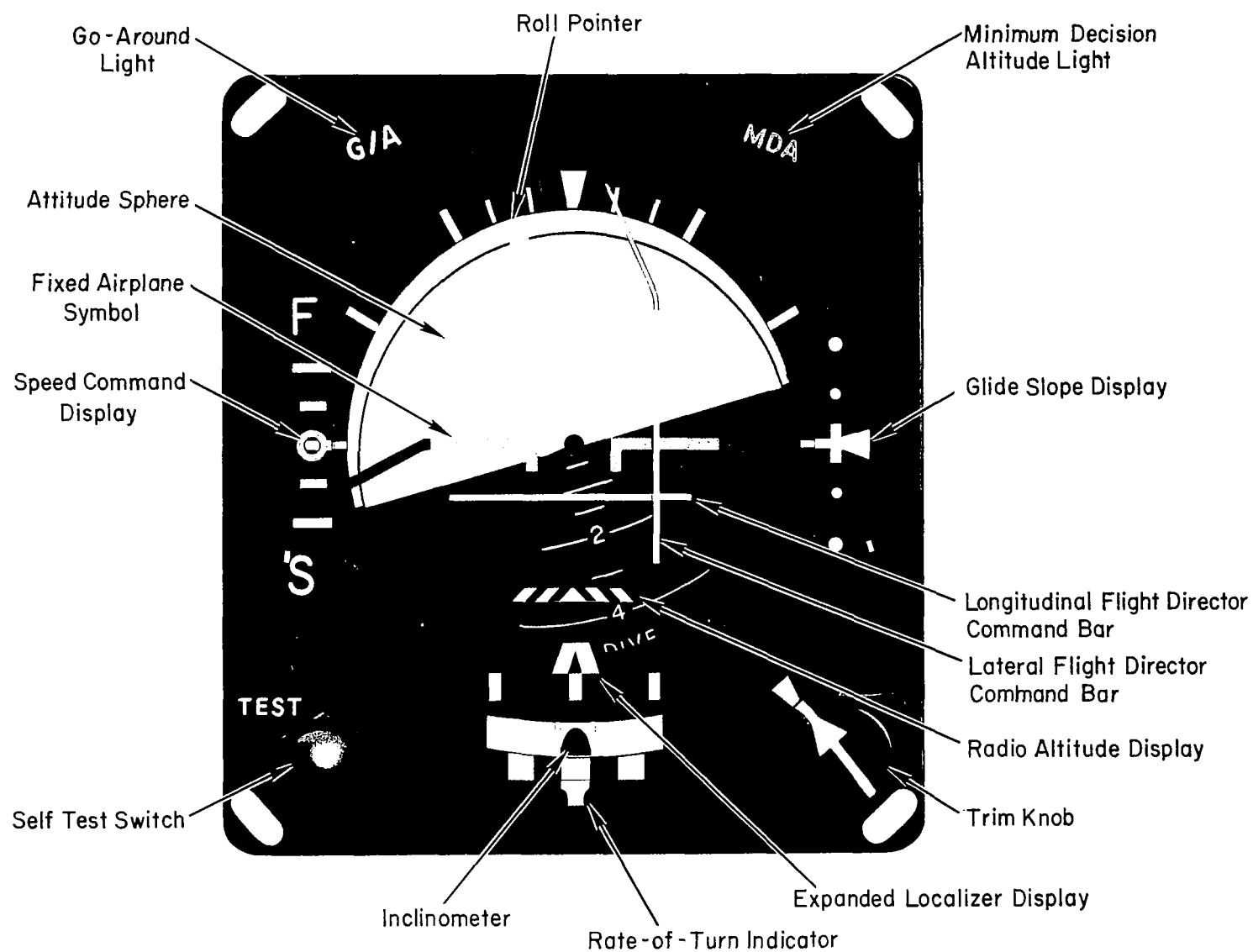
Figure D-4. Sperry HZ-6B Attitude Director Indicator
