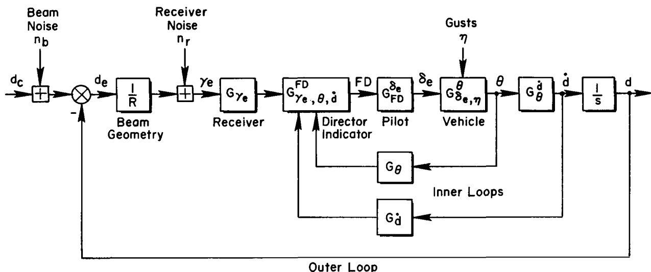
Figure 2. Block Diagram for Approach Control with Flight Director
