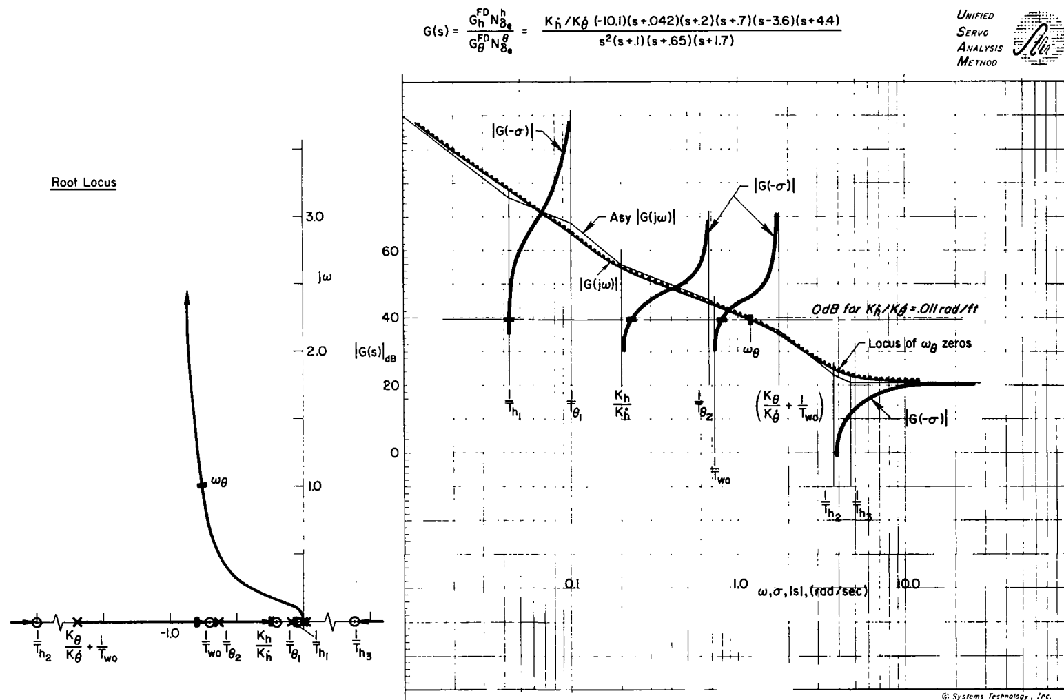
Figure C-1. Flight Director Numerator Survey
