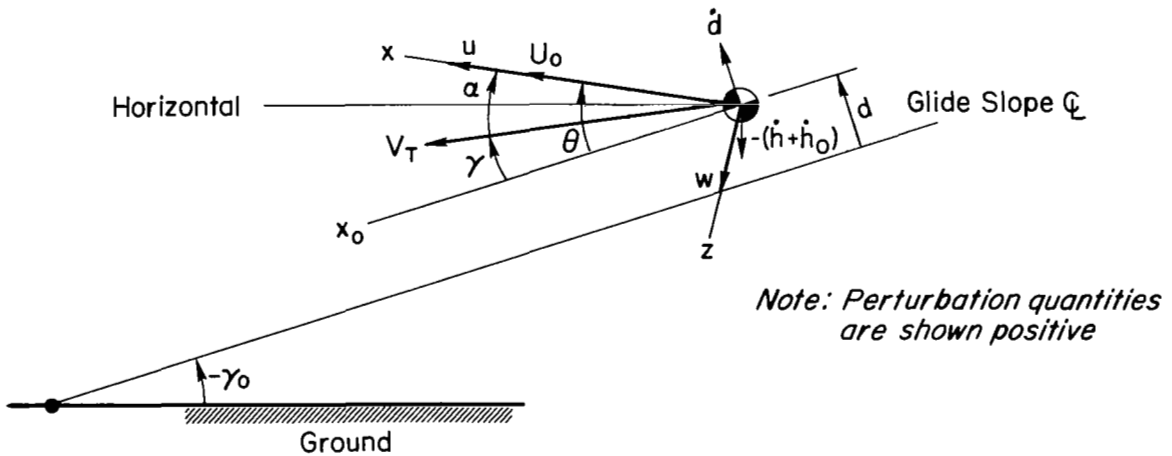
Figure 6. Perturbed Axis System Alignment
