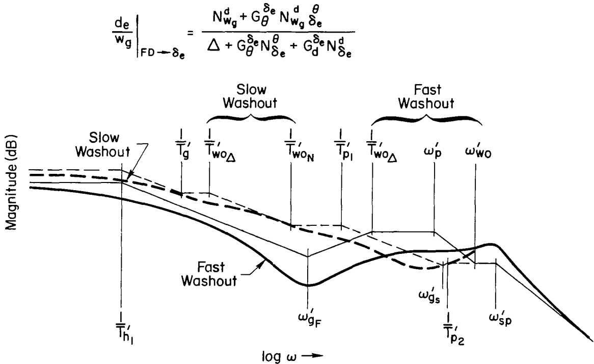
Figure 12. Effect of Pitch Attitude Washout on Beam Error Due to w-Gust
