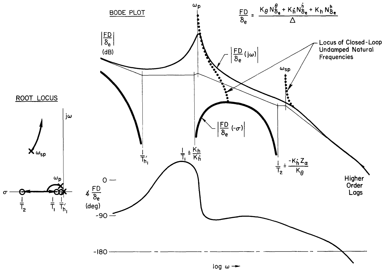
Figure 9. Director/Vehicle Properties with Beam Rate Added
