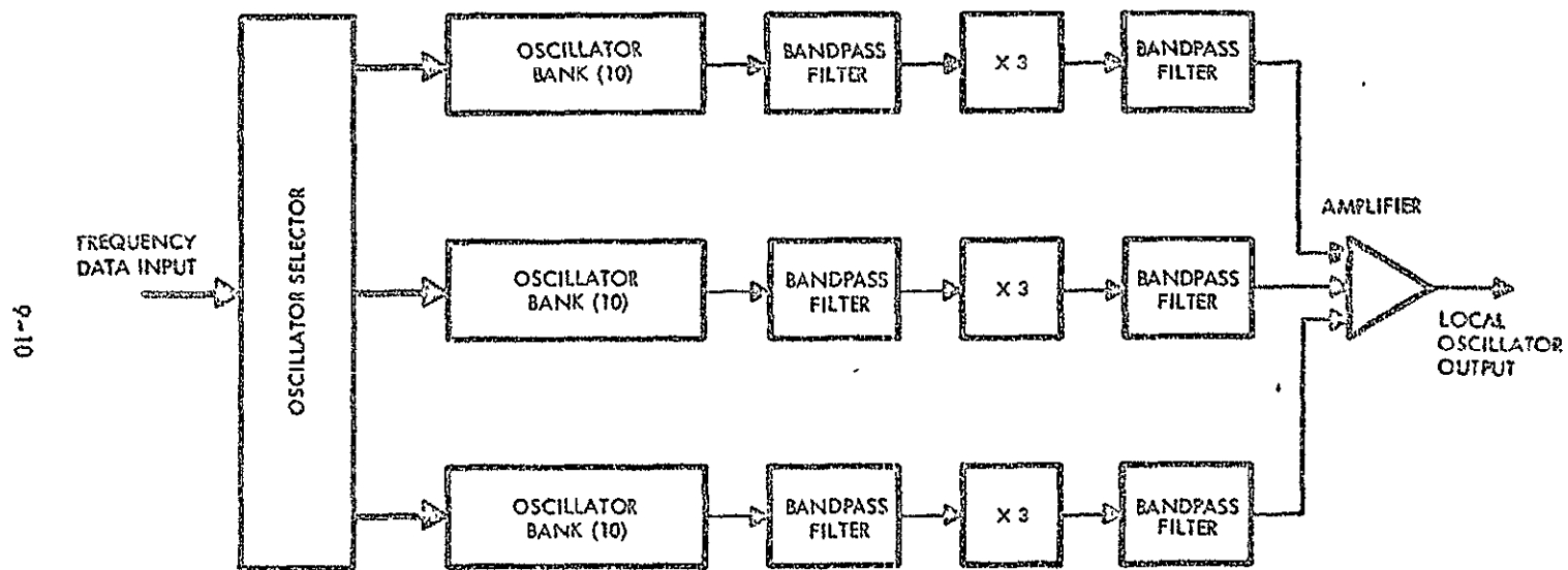
Figure 9.3.2-2. Crystal Oscillator Implementation
