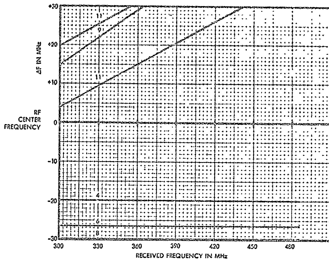
Figure 9.4.1-1. Spurious Responses — F(\text{IF}) = 40 \text{ MHz}
