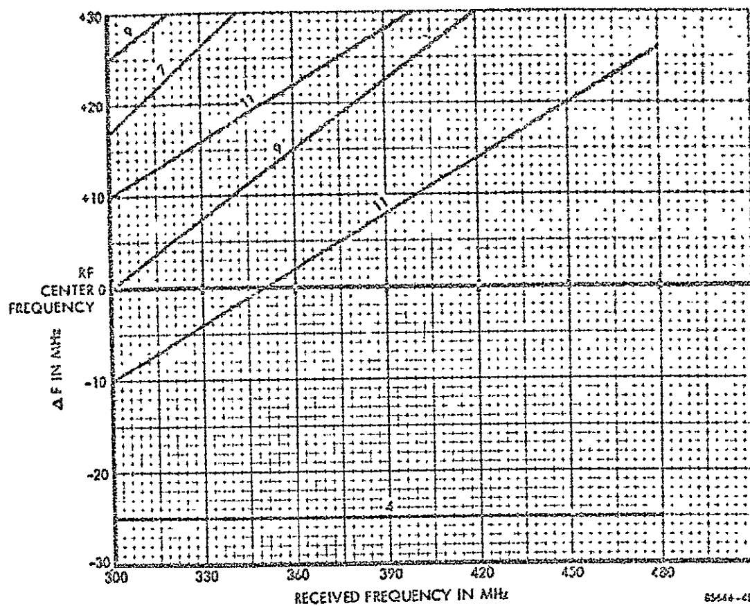
Figure 9.4.1-2. Spurious Response — F(\text{IF}) = 50 \text{ MHz}
