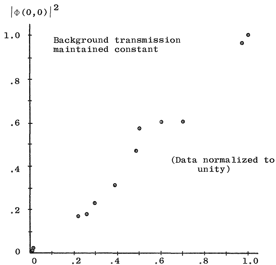
Figure 22. Output correlation intensity as a function of input rectangular aperture transmission.
