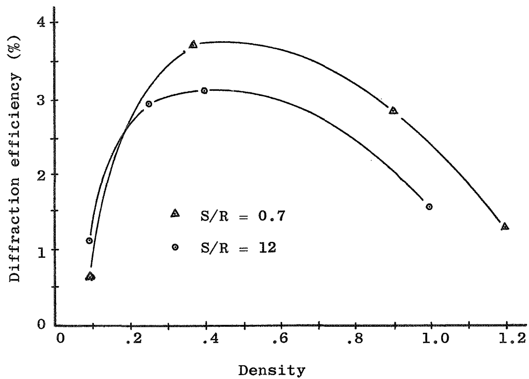
Figure 16. Diffraction efficiency as a function of density.
