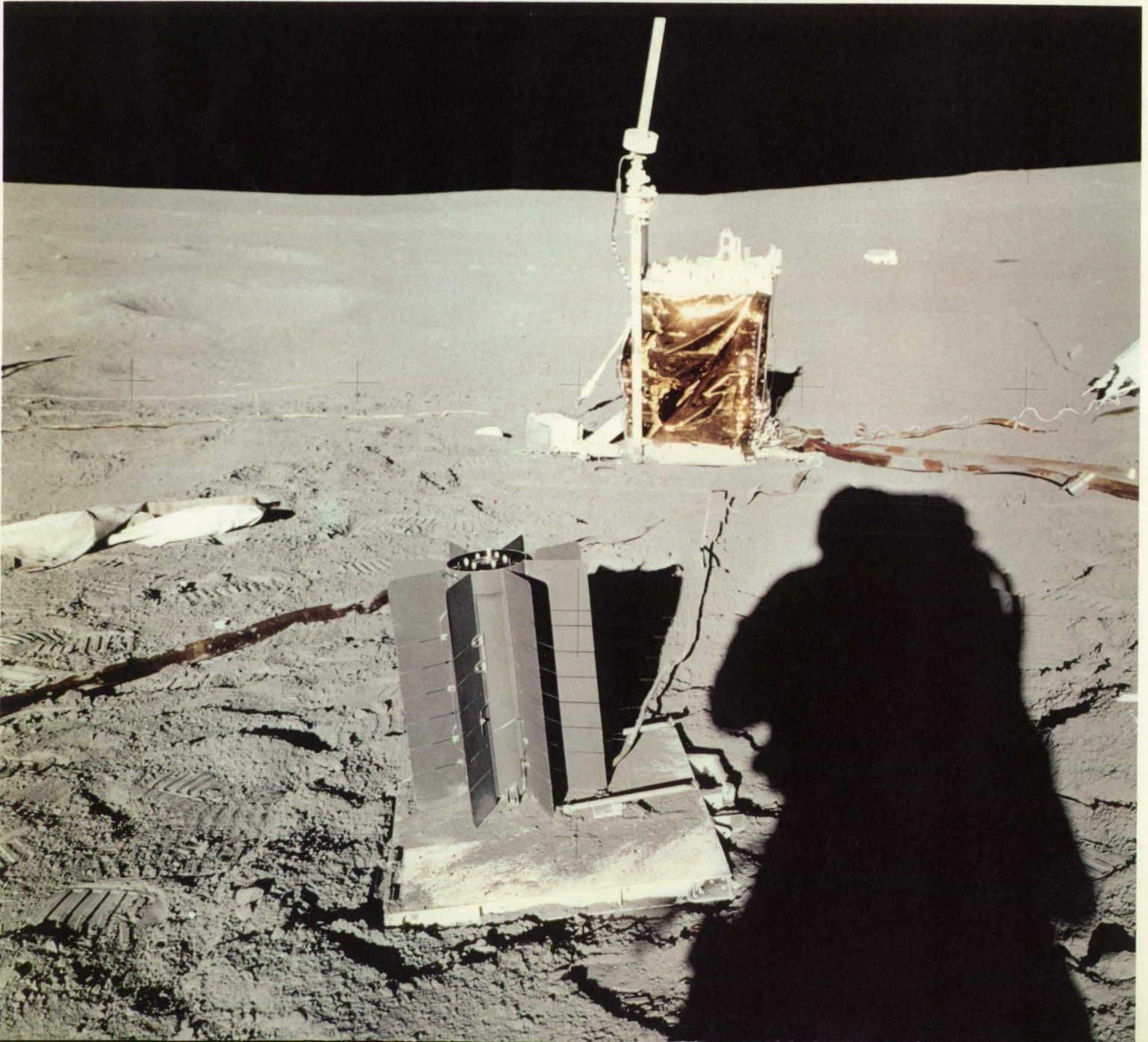
The nuclear power plant in the foreground is the radioisotope thermoelectric generator (RTG) which is connected to scientific instruments to provide them with needed electricity.
