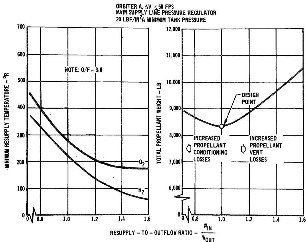
SELECTION OF RESUPPLY FLOW RATE
