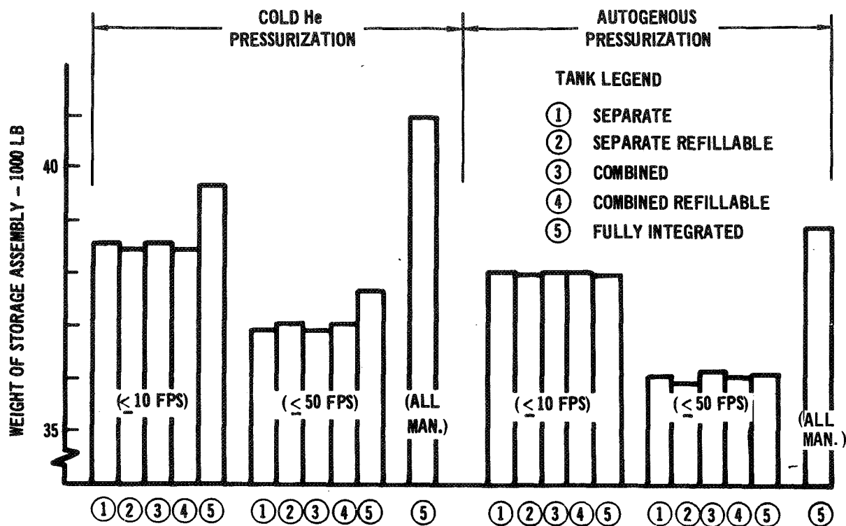
APS/OMS TANKAGE WEIGHT SUMMARY
