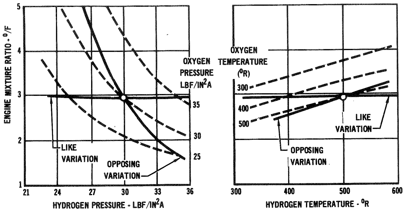
ENGINE MIXTURE RATIO SENSITIVITY CHAMBER PRESSURE - 20 LBF/IN²A
