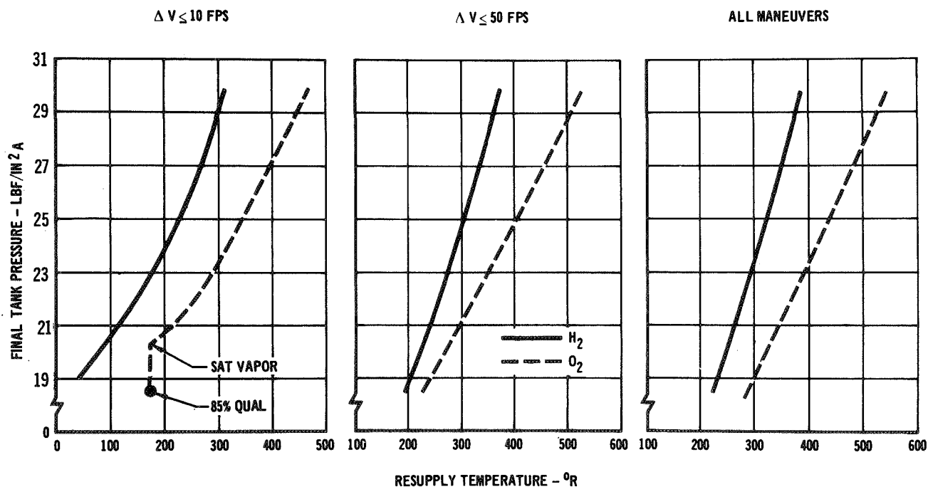
MAIN TANK PRESSURE DEPENDENCY ON RESUPPLY TEMPERATURE (Orbiter A)
