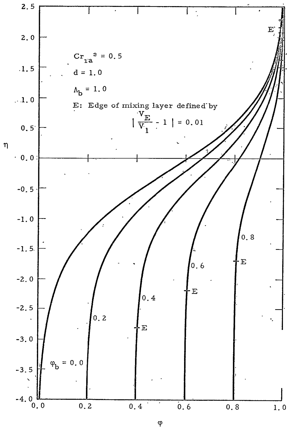
Figure 7 Turbulent velocity profiles for various velocity ratio:
