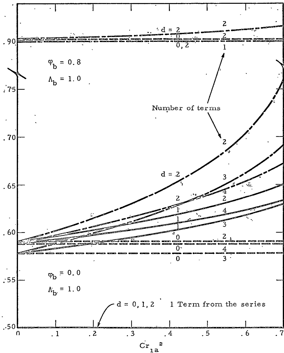
Figure 3 Isoenergetic results of a_1 for isobaric mixing
