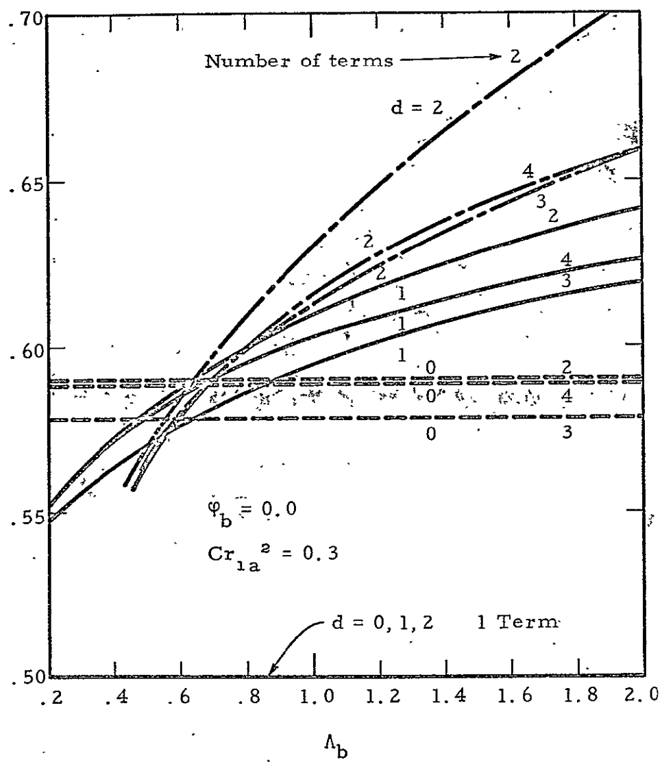
Figure 5 Non-isoenergetic results of a_1 for isobaric mixing
