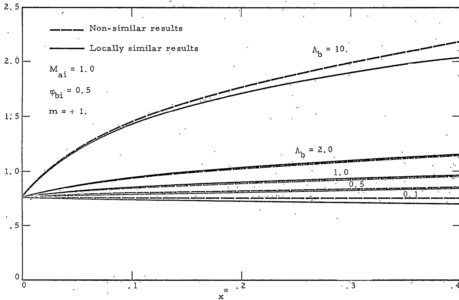
Figure 19a Comparison of a_1 as a function of x^* for the locally similar and non-similar solutions
