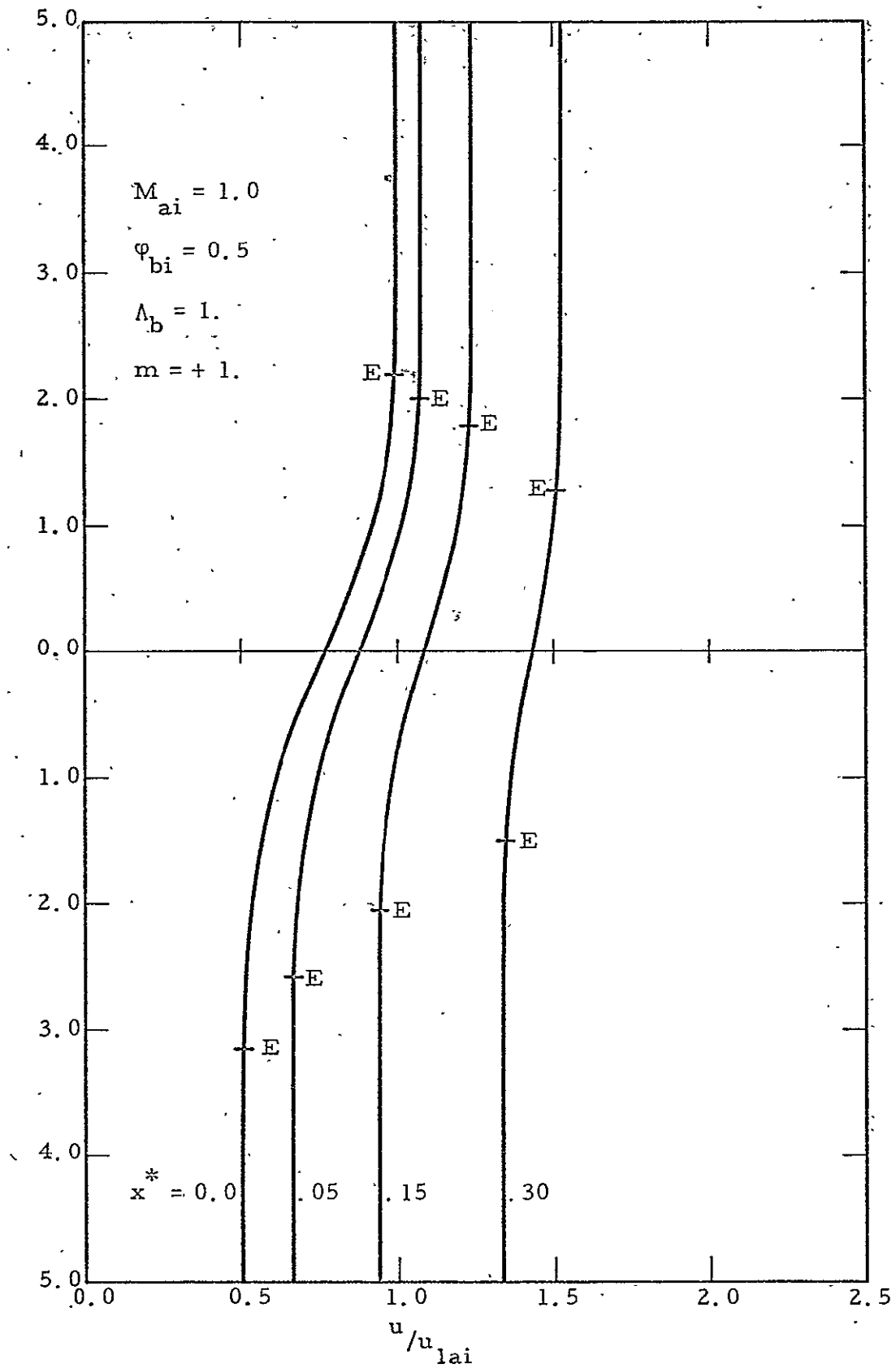
Figure 14b Velocity profiles for \Lambda_b = 1.0
