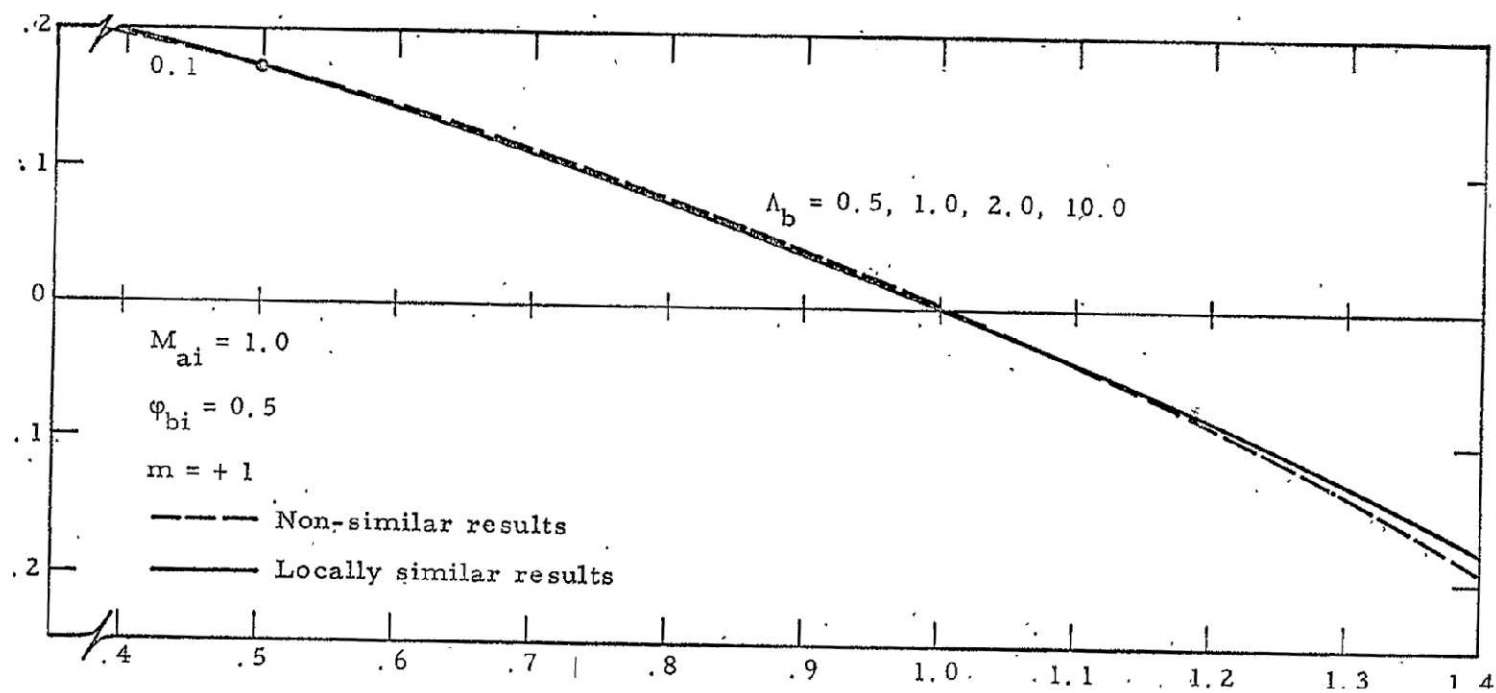
Figure 19d Comparison of a_2 as a function of \phi_b for the locally similar and non-similar solutions
