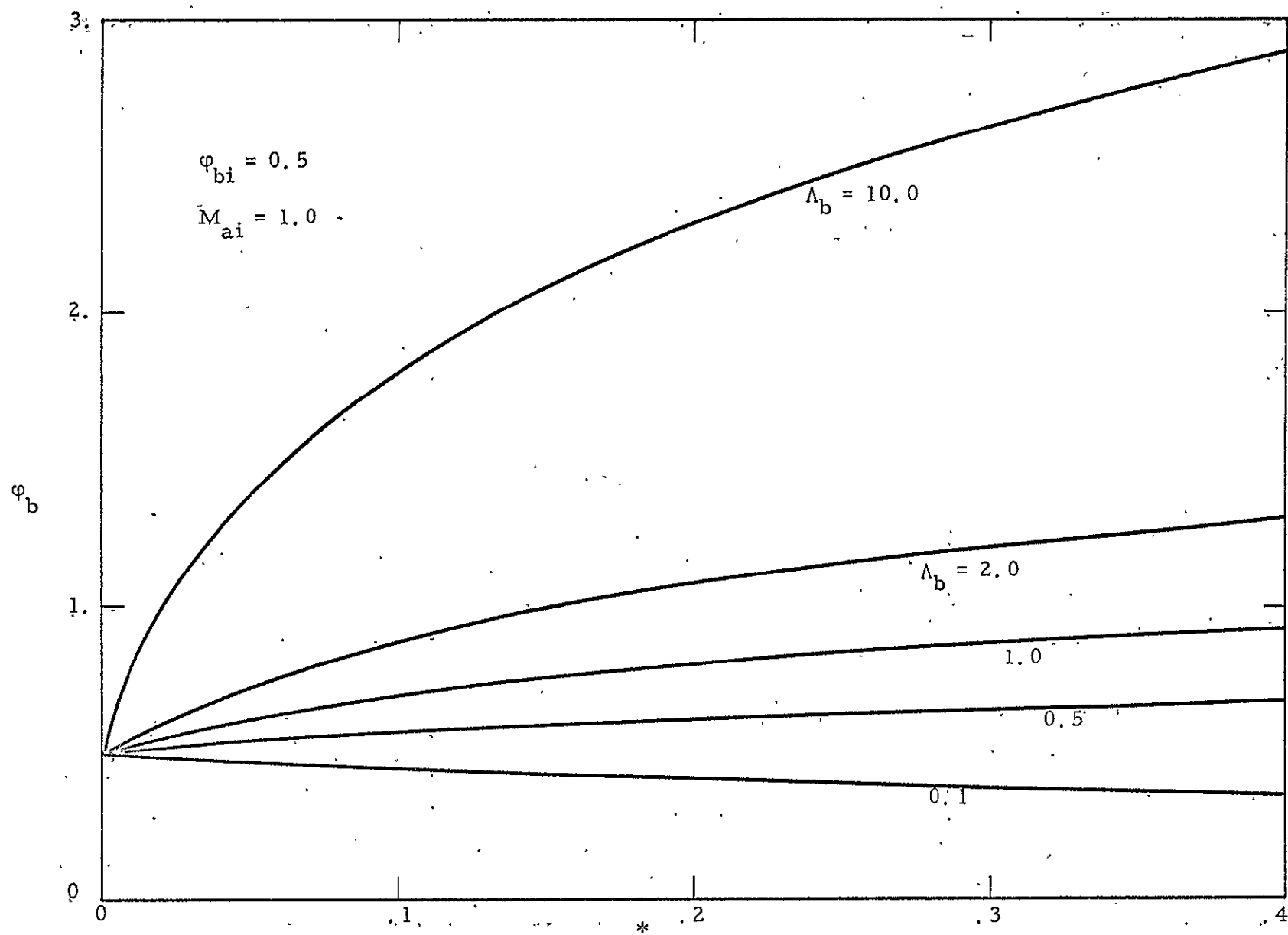
Figure 12 Local freestream velocity ratio as a function of x^*
