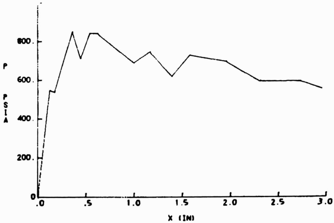
TWO-PHASE DETONATION
