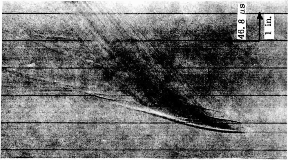
Figure 6. Non-reacting 2130 \mu DECH Drop.
