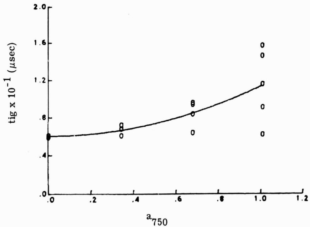
Figure 10. Position Behind Leading Shock and Time of Ignition vs. Equivalence Fraction of 750\mu Diameter Drops; \phi_T = .430 .
