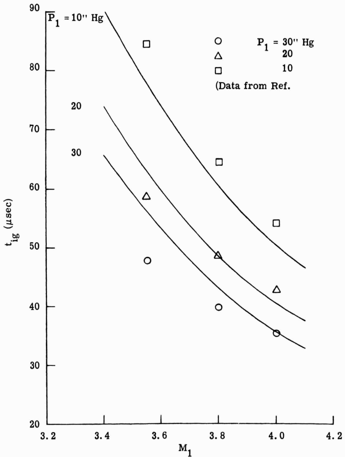
Figure 14. Ignition Time from Single Micromist Droplet Ignition Theory; D_0 = 2130\mu , q_{vT} = 3240 \text{ ft-lb/ft}^3 .
