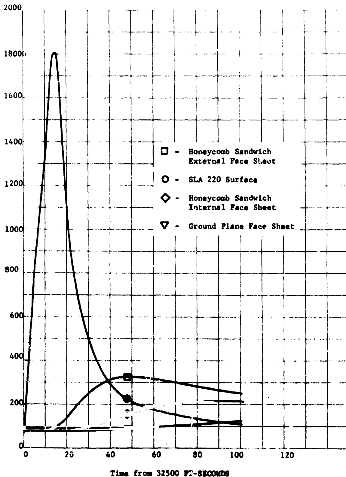
FIGURE 5 - PAET Afterbody Thermal Response, \dot{q}/\dot{q}_s = 0.10 , 27 One-Dimensional Analysis
