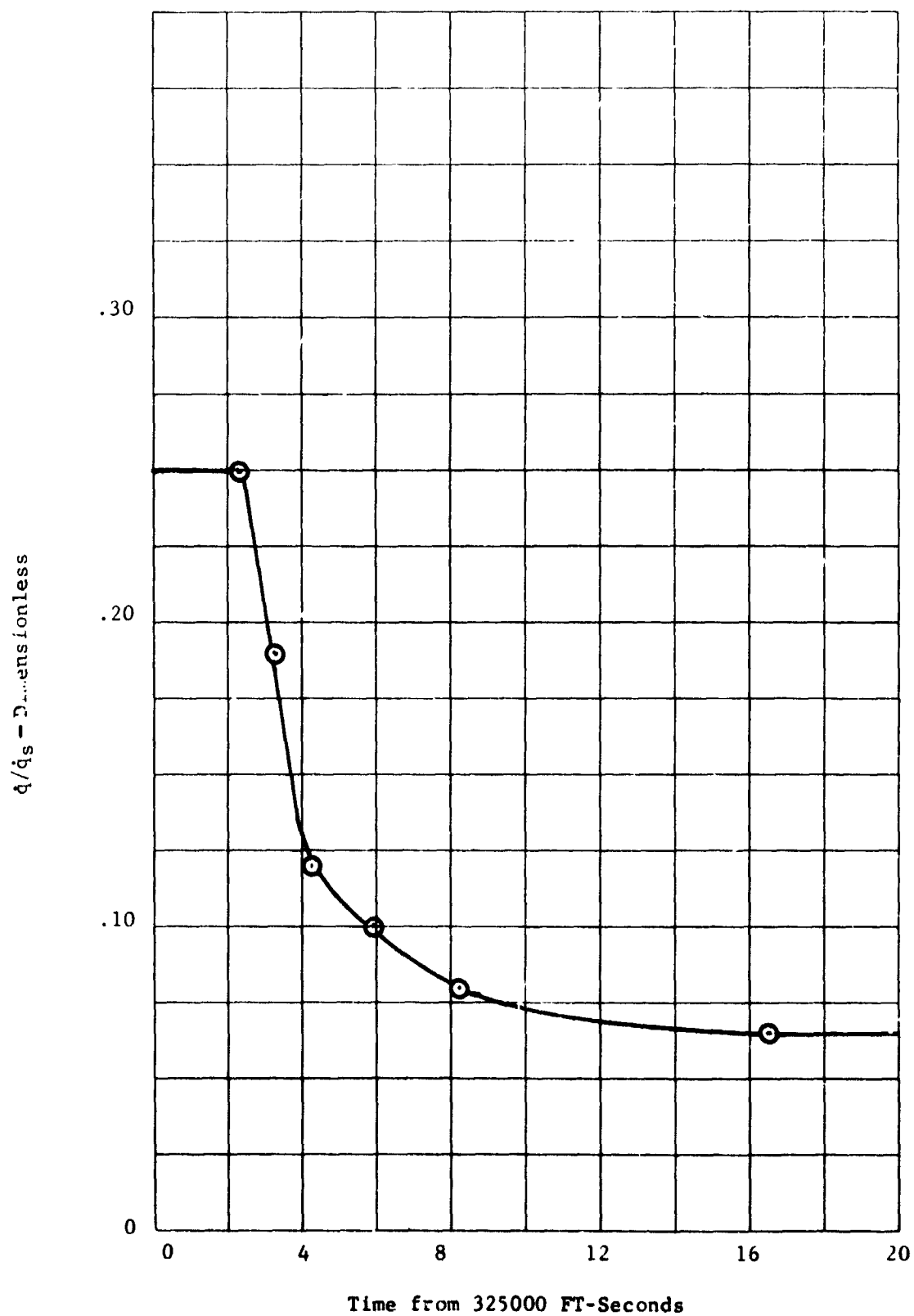
Figure 2. Variable q/q_s for One-Dimensional Thermal Analysis
