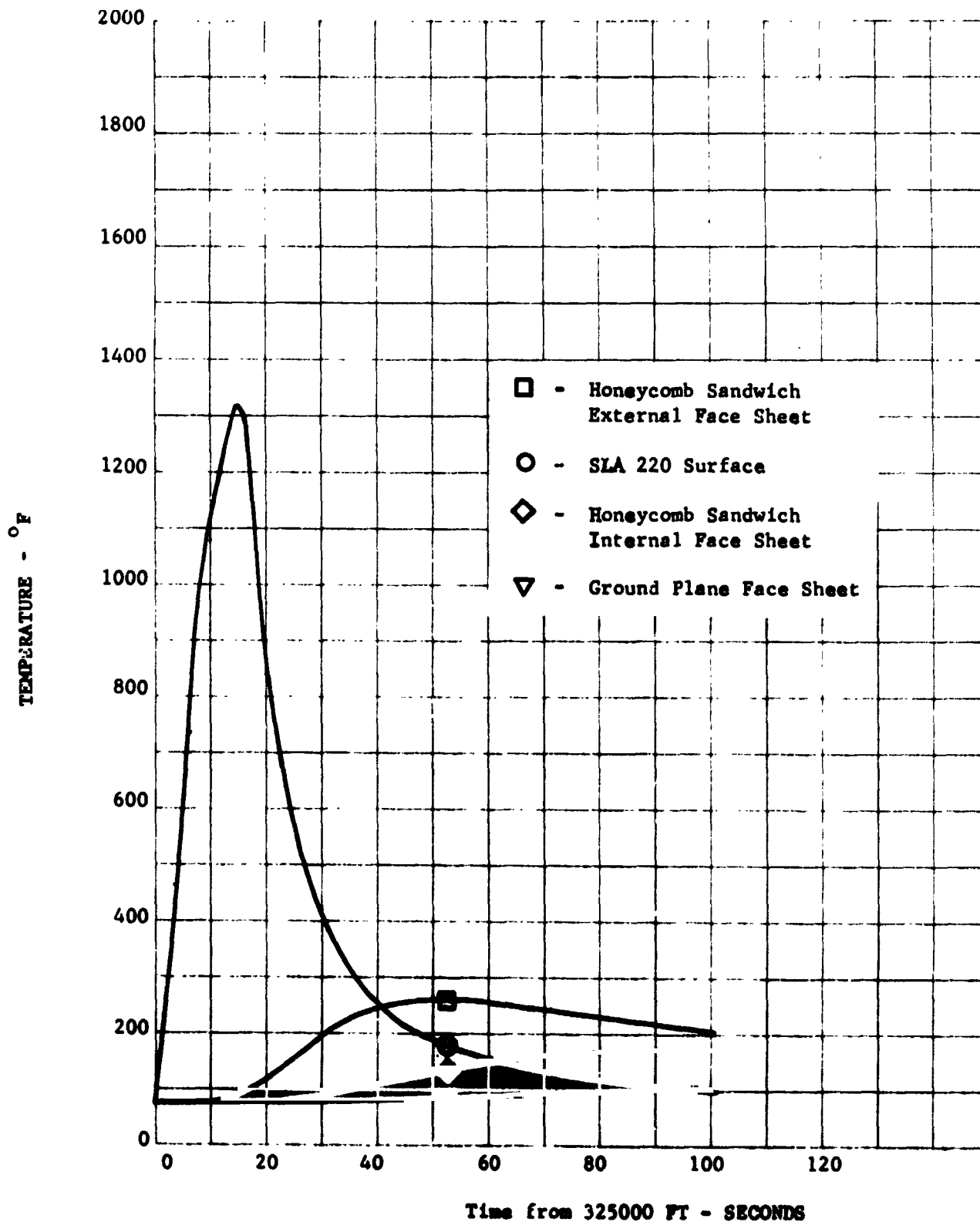
FIGURE 4 - PAET Afterbody Thermal Response, \dot{q}/\dot{q}_s = 0.05 , One-Dimensional Analysis
