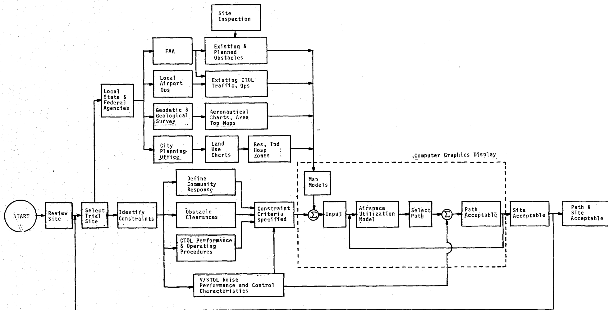
FIGURE 4 PLANNING SEQUENCE DIAGRAM FOR THE DETERMINATION OF V/STOL FLIGHT PATHS
