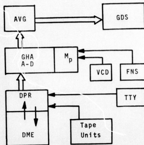
FIGURE A1 ADAGE 30 GRAPHICS TERMINAL
