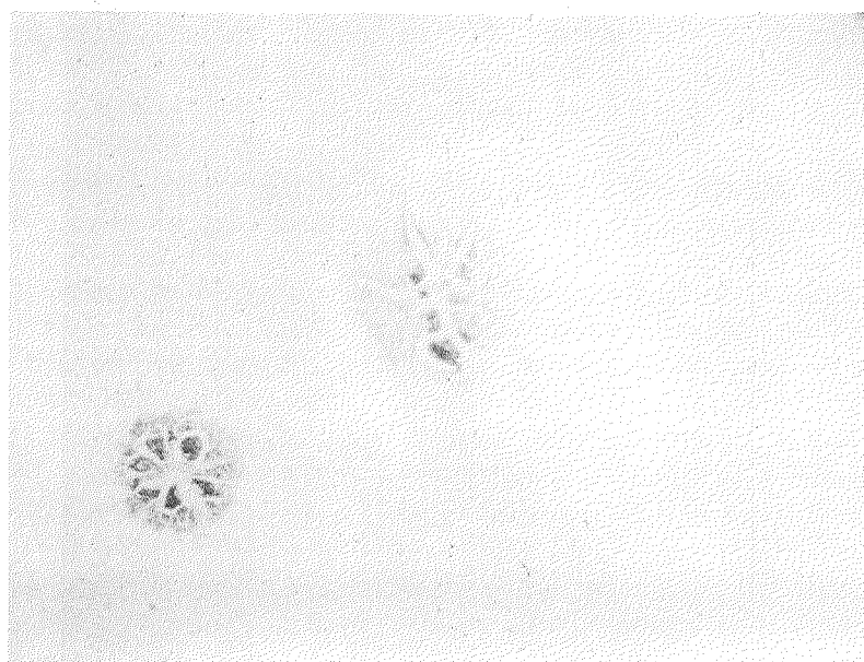
Figure A-2. - Oxide Defect Decoration After Fluid Evaporation. 100X
