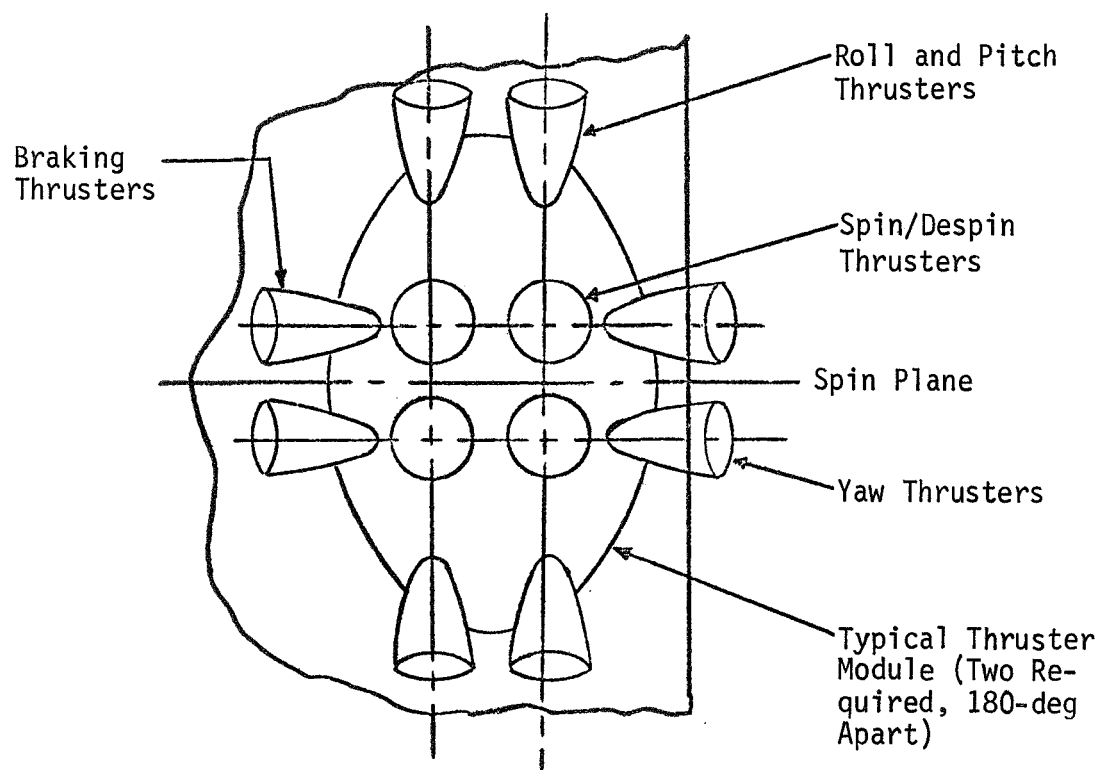
Fig. II-1 Thruster Location
