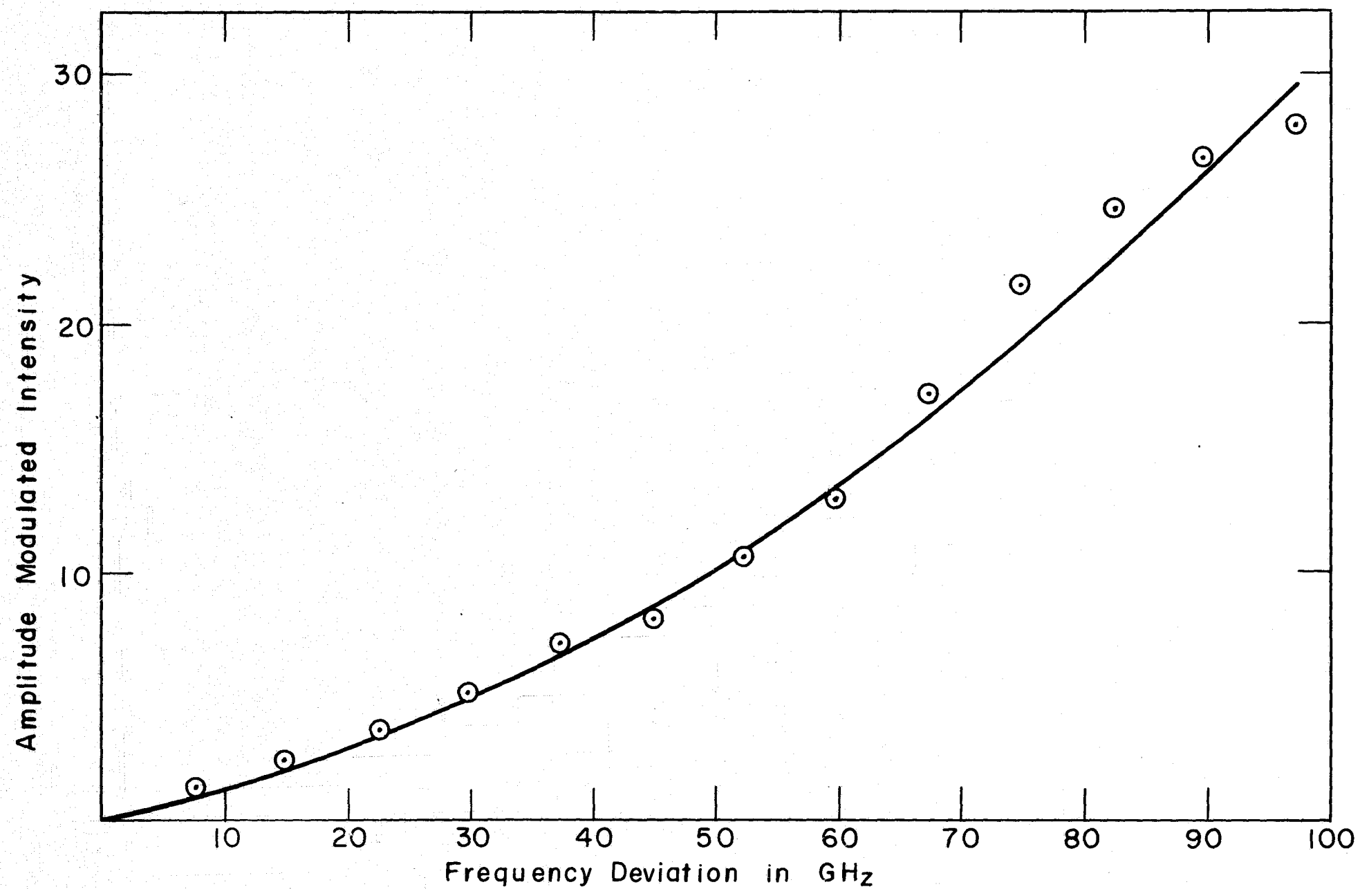
Figure 4-13 Component of the Amplitude Modulated Intensity at the Modulating Frequency vs Frequency Deviation
