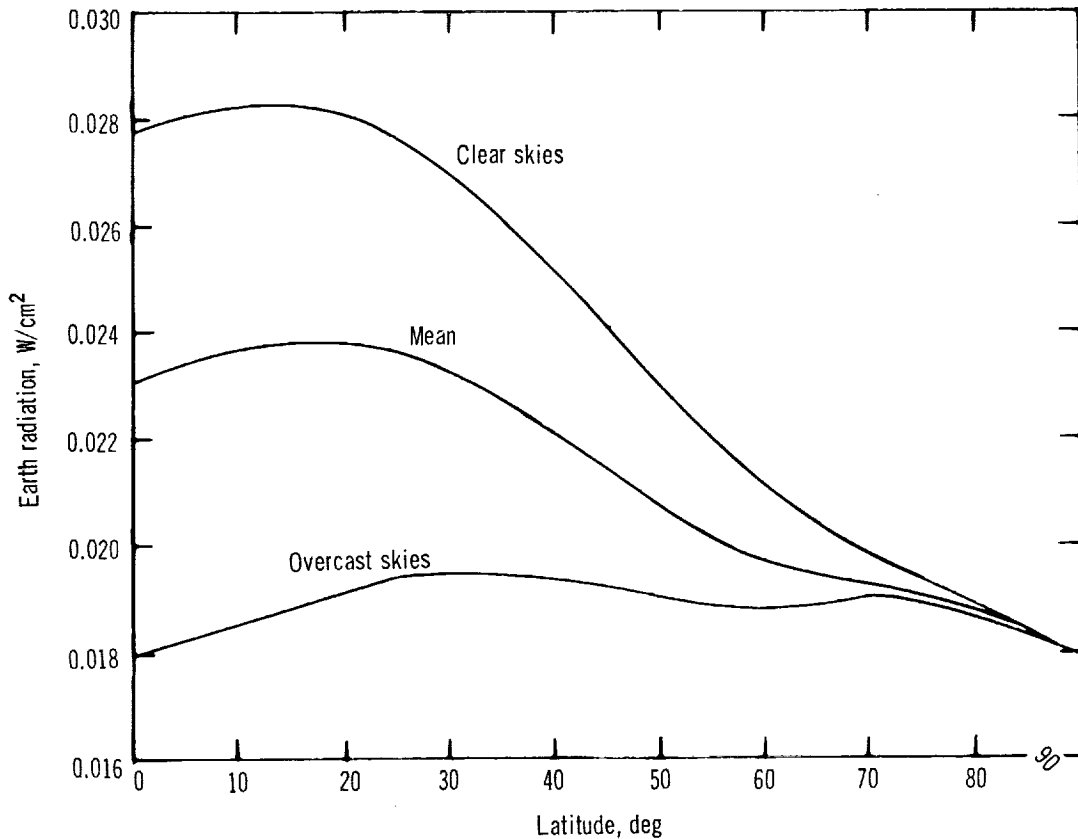
Figure 10.—Earth radiation as function of latitude under various sky conditions.
