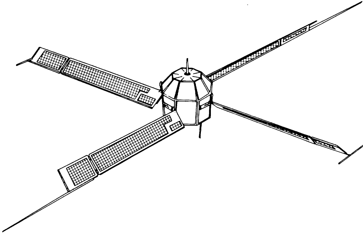
Figure 3.—Beacon Explorer-B (Explorer 22).
