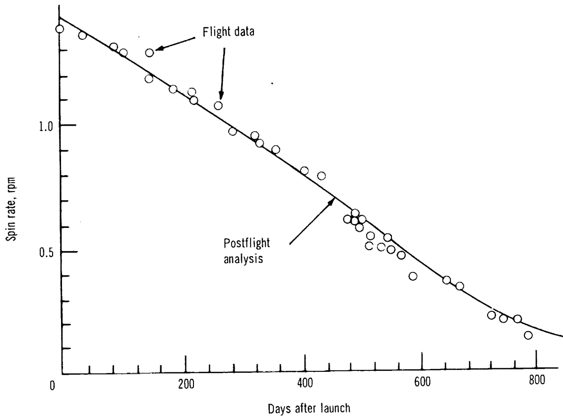
Figure 2.—Alouette 1 spin decay (ref. 9).
