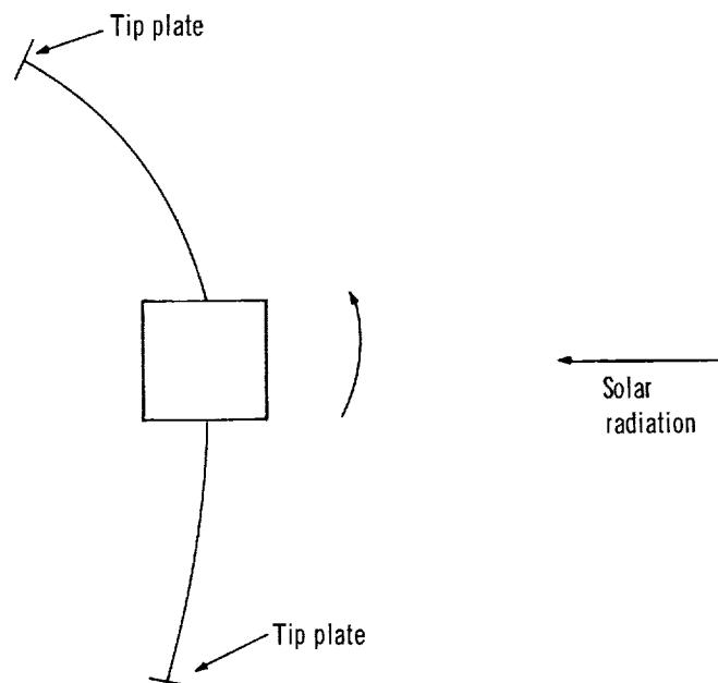
Figure 16.—Tip plates.
