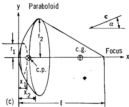
Figure 15.—Torque and center of pressure for absorbing surfaces of revolution: (a) cone, (b) spheroid, and (c) paraboloid.
