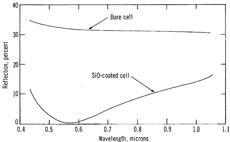
Figure 14.—Reflection from bare and coated solar cells as a function of wavelength (ref. 33).
