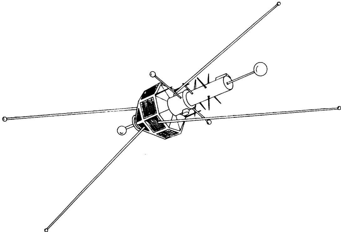
Figure 4.—DODGE satellite.
