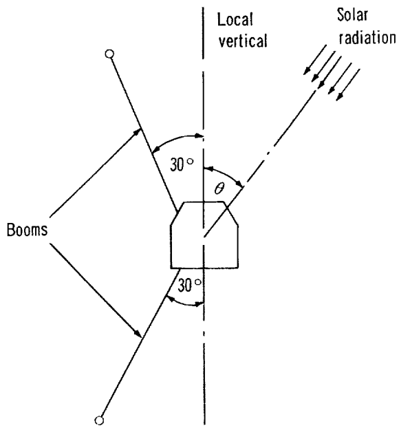
Figure 5.—Unsymmetrical configuration for DODGE satellite.
