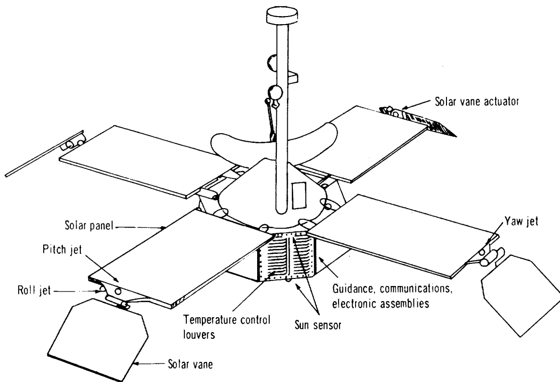
Figure 6.—Mariner 4 satellite.
