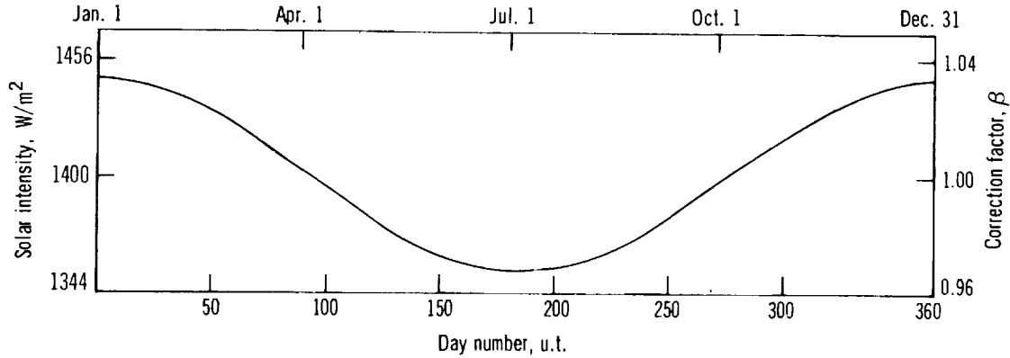
Figure 7.—Solar intensity as a function of day number.
