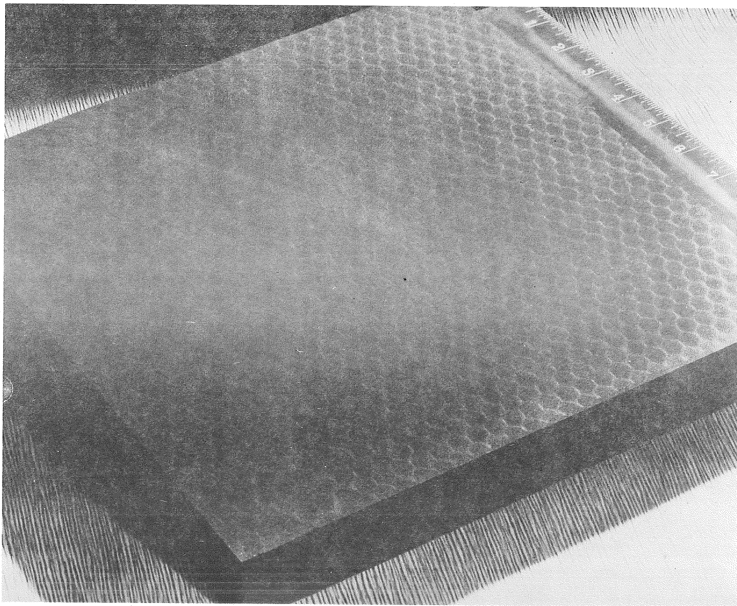
FIGURE 14 Cured 12 inch x 12 inch sub-scale ablation test panel No. S-4 10 Percent Elastomer, 90 Percent Microballoons
