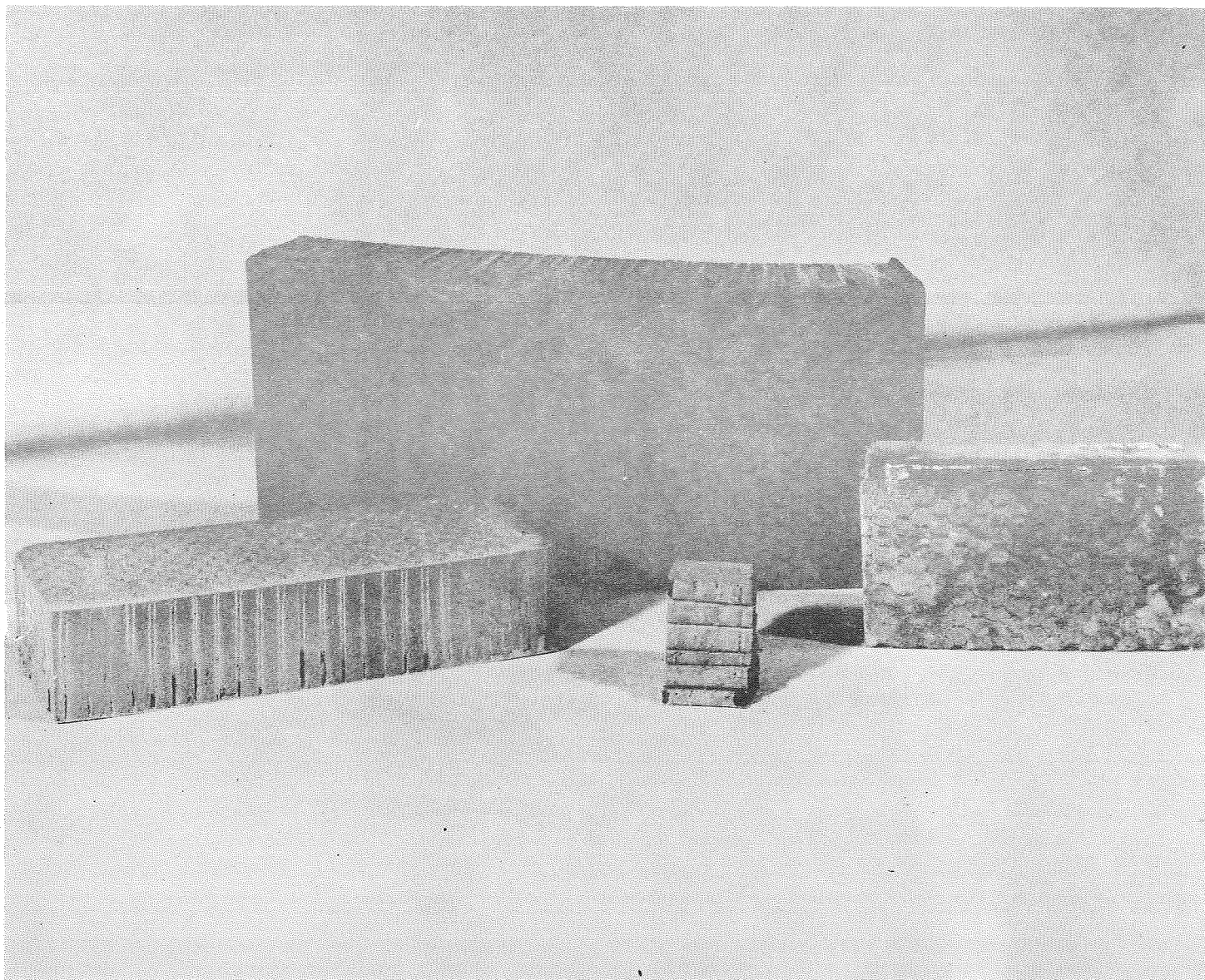
FIGURE 16 Sub-scale and Full scale test panel specimens Elastomer 20 percent, Microballoons 80 percent
