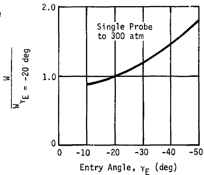
Fig. II-12 Effect of Entry Angle on Probe System Weight
