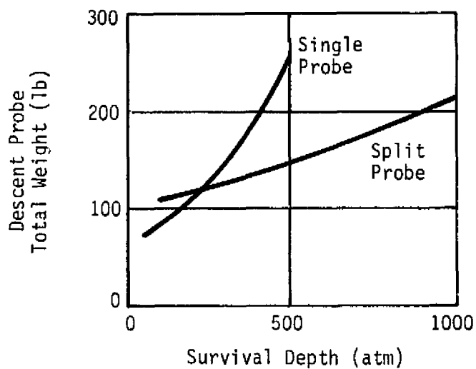
Fig. II-10 Effect of Depth on Descent Probe Weight
