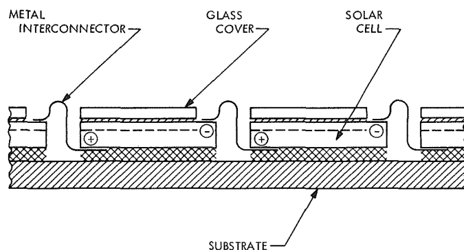
Fig. C-1. Solar cell interconnect design
