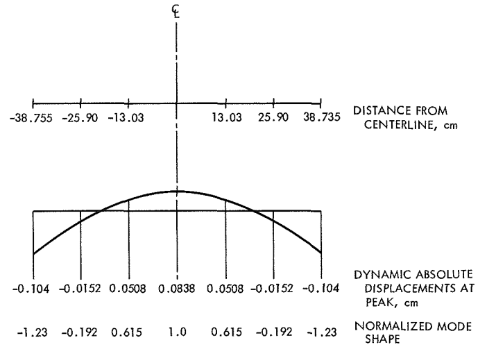
Fig. 5. End view of Mariner Mars 1969 panel
