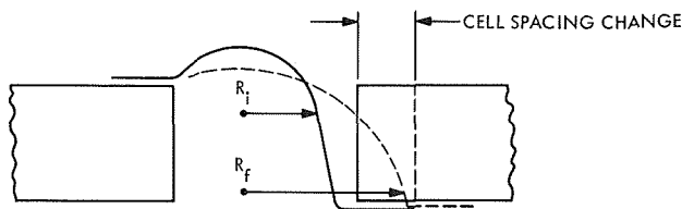
Fig. C-3. Interconnect design with essentially no expansion loop
