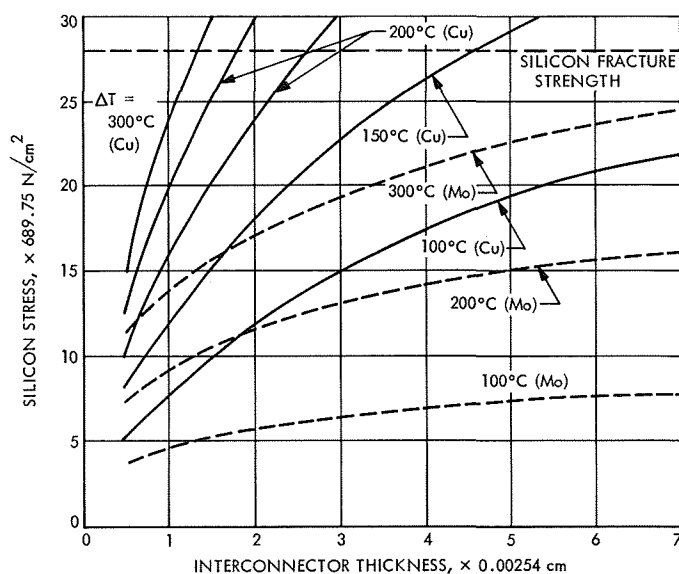
Fig. C-7. Thermal stresses in silicon under a metal tab of various thicknesses
