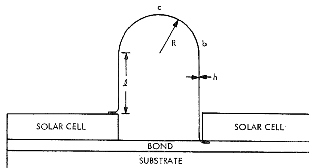
Fig. 6. Typical interconnect
