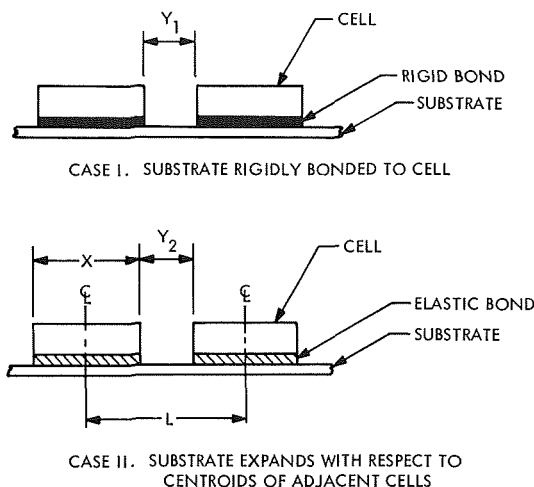
Fig. C-2. Solar cell thermal expansion model
