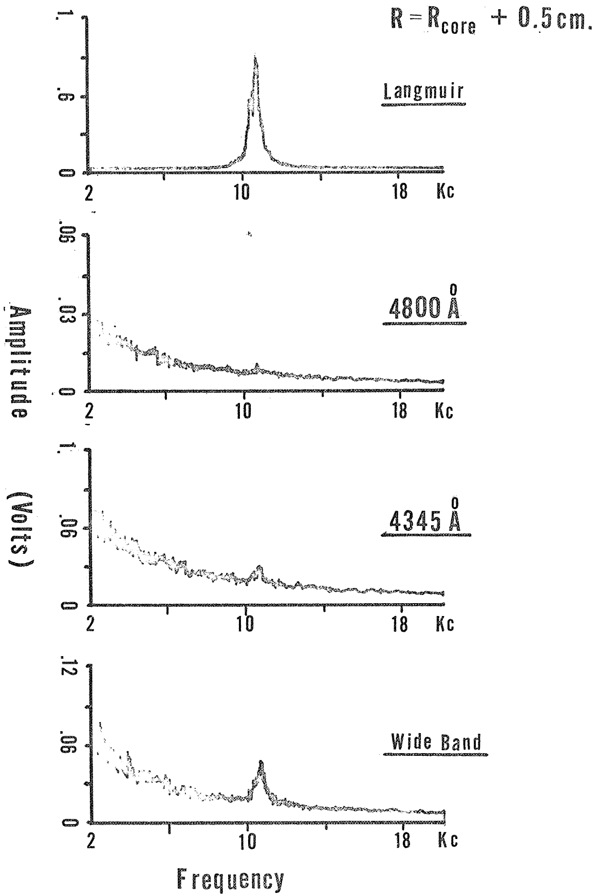
Frequency spectra under the same condition as Figure 19 taken at 0.5 cm from the edge of the core
