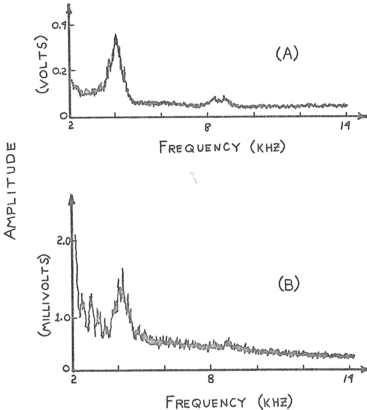
Amplitude of Ion Acoustic Wave vs. Frequency. (a) Langmuir Probe; (b) Magnetic pickup Coil. B = 580 Gauss, P = 4.0 \times 10^{-4} torr.
